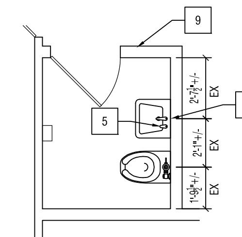
1 3RD FL POWDER RM FL PL SCALE: 1/4" = 1'-0" ROOM 2C003
