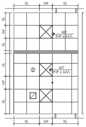
2 2ND FLR PUBLIC RESTROOM RCP ROOM 2N007 A103 1/4"=1'-0"
