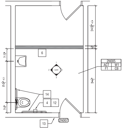
1 2ND FLR PUBLIC RESTROOM PL ROOM 2N007 A103 1/4"=1'-0"
