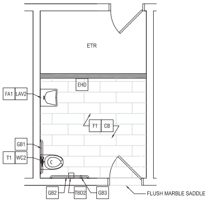
3 2ND FLR PUBLIC RESTROOM FINISH PL ROOM 2N007 A103 1/4"=1'-0"
