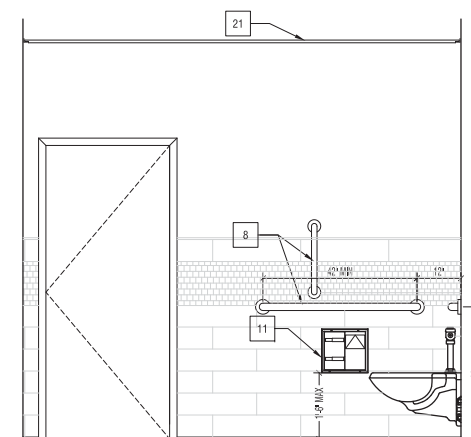
3 2ND FLR PUBLIC RESTROOM ELEV A204 1/2"=1'-0" ROOM 2N007
