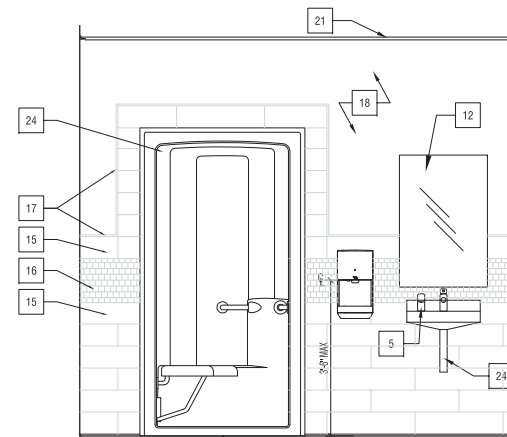
1 2ND FLR PUBLIC RESTROOM ELEV A204 1/2"=1'-0" ROOM 2N007
