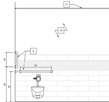
2 2ND FLR PUBLIC RESTROOM ELEV A204 1/2"=1'-0" ROOM 2N007
