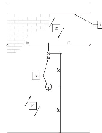
6 2ND FLR SHOWER STALL ELEV ROOM 2N006 A-204 1/2"=1'-0"
