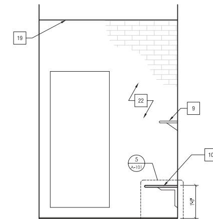
2 2ND FLR SHOWER ELEV ROOM 2N006 A-204 1/2"=1'-0"
