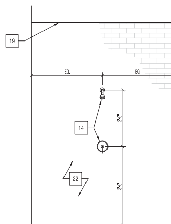
8 2ND FLR SHOWER STALL ELEV ROOM 2N006 A-204 1/2"=1'-0"
