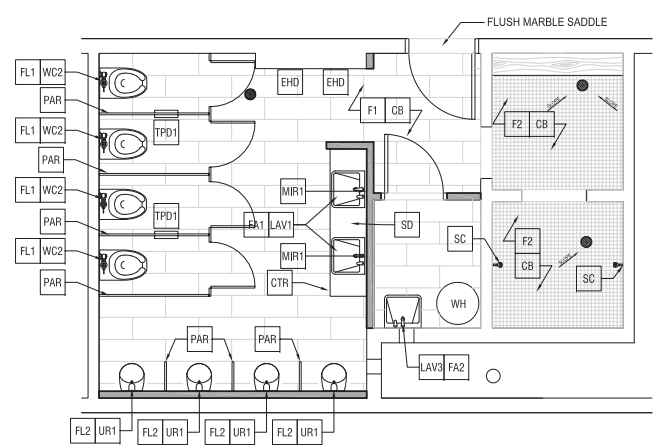
3 1ND FLR MENS RESTROOM FINISH PL ROOM 2N006 SCALE: 1/4" = 1' - 0"
