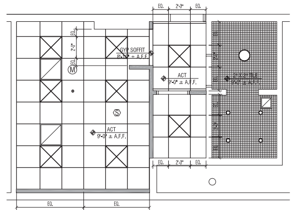
2 2ND FLR MENS RESTROOM RCP ROOM 2N006 SCALE: 1/4" = 1' - 0"
