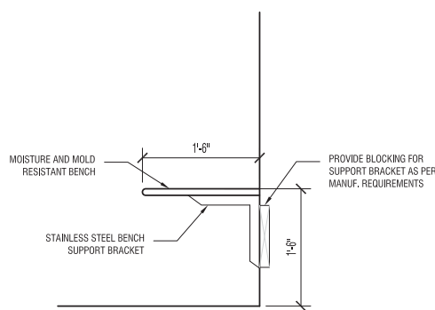
5 SHOWER ROOM BENCH DETAIL SCALE: 1/4" = 1' - 0"
