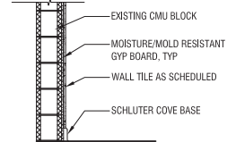
4 TYP TILE WALL DETAIL SCALE: 1/2" = 1' - 0"
