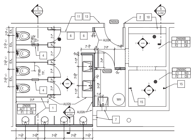
1 2ND FLR MENS RESTROOM PL ROOM 2N006 SCALE: 1/4" = 1' - 0"
