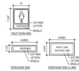
SIGNAGE MOUNTING DETAILS
