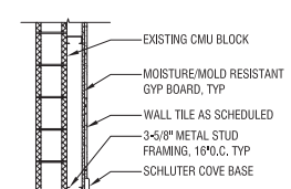
6 URINAL WALL DETAIL SCALE: 1/2" = 1' - 0"
