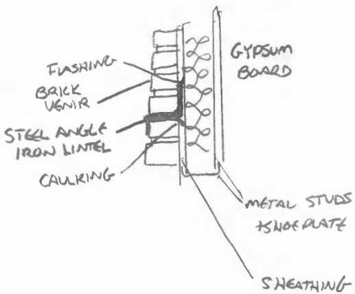
HEADER DETAIL OVER NEW DOORWAY (EXISTING WINDOW HEADER - MODIFYING ONLY FOR DOOR)
