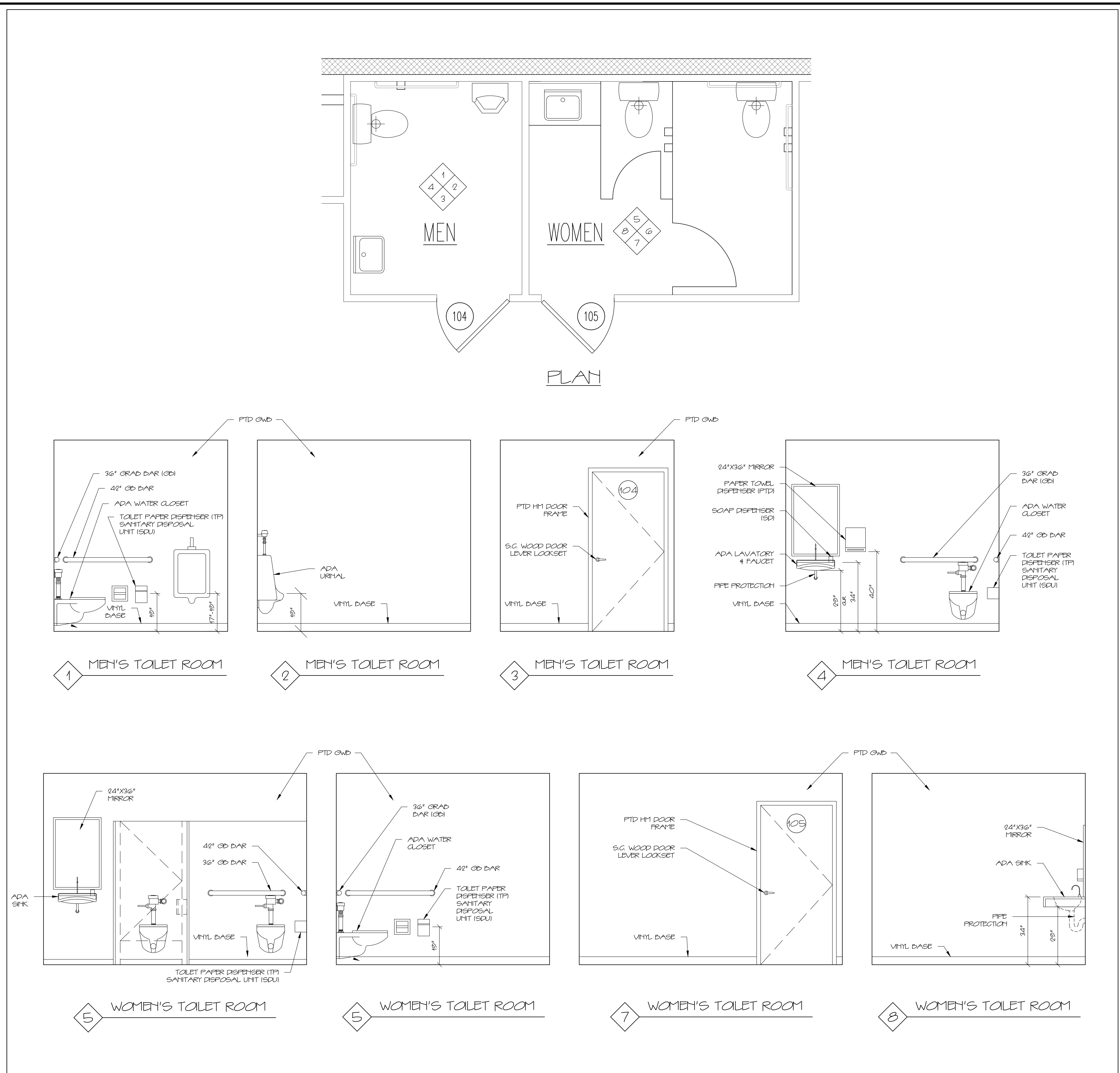
2 ADA TOILETS PLAN & ELEVATIONS 1/2" = 1'-0"
