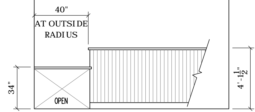
1 COUNTER ELEVATION - ADA SCALE: 1/2" = 1'-0"
