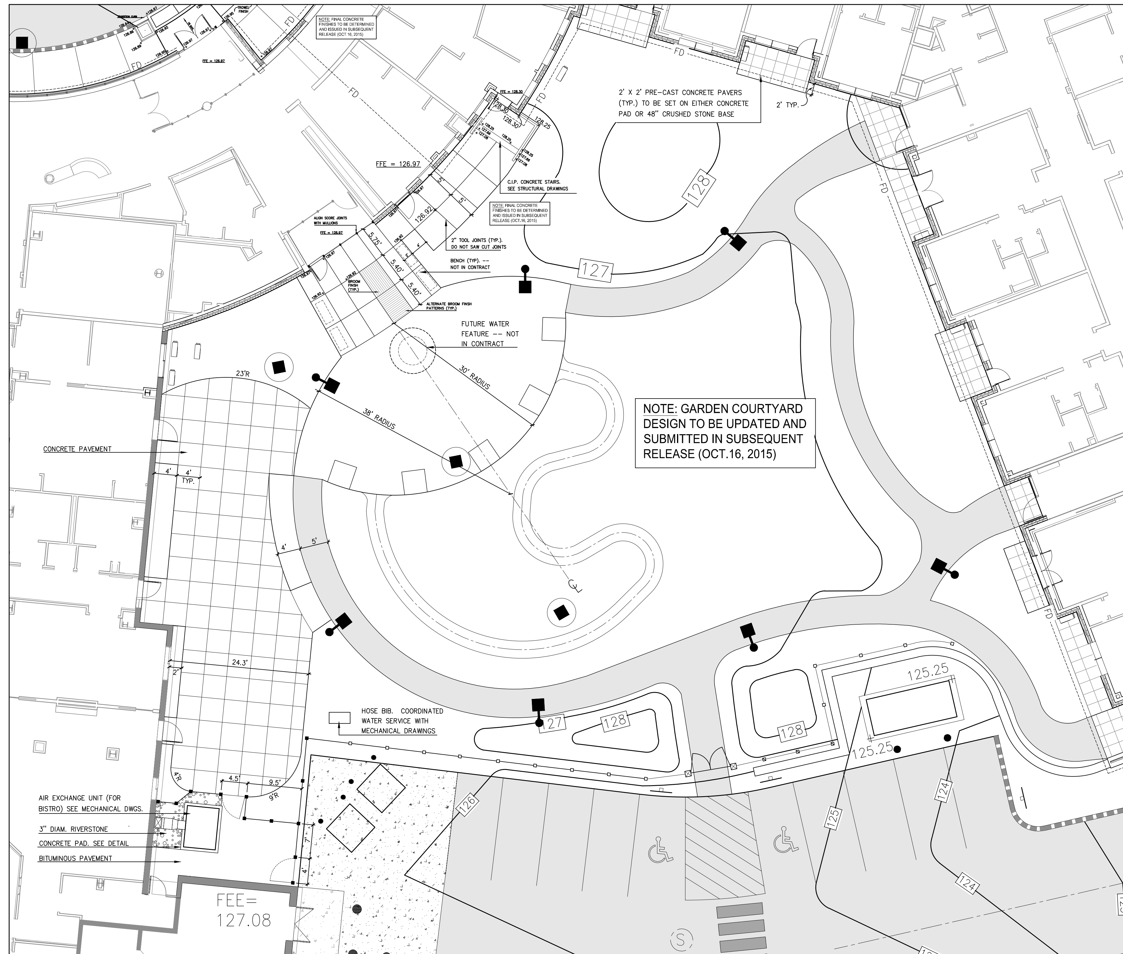
COURTYARD DETAIL PLAN SCALE: 1" = 10'
