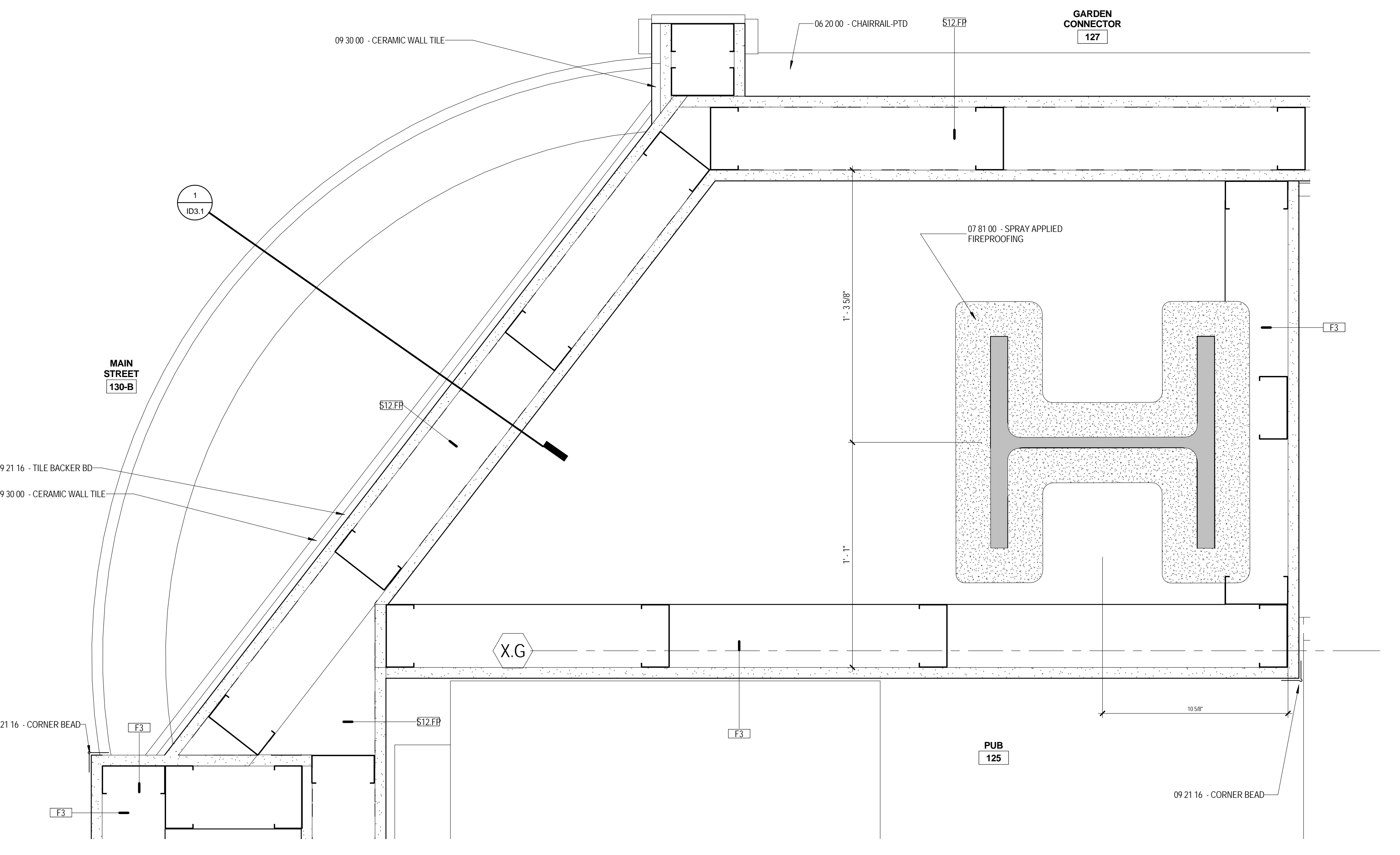
J6 PLAN DETAIL @ GARDEN CONNECTION 127 A5.9 3" = 1'-0"
