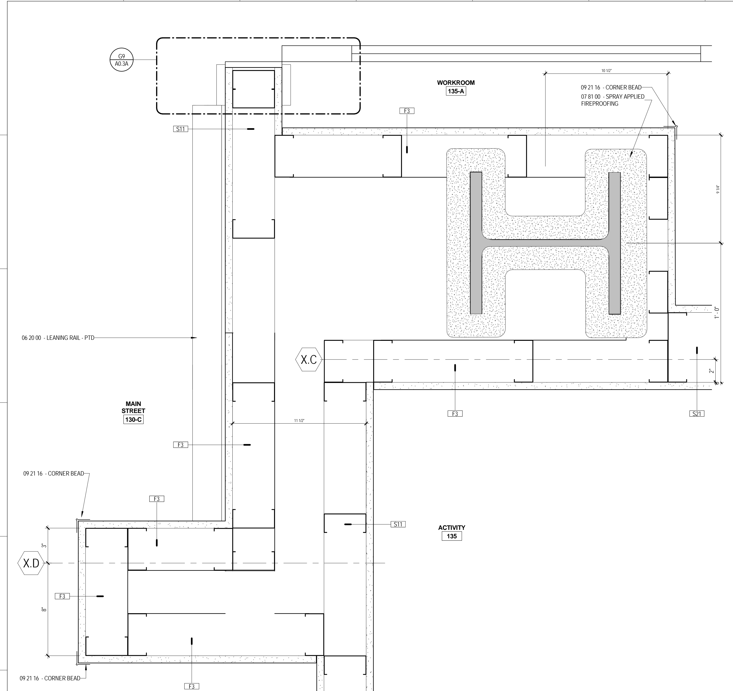
F1 PLAN DETAIL @ ACTIVITY 133 A5.9 3" = 1'-0"
