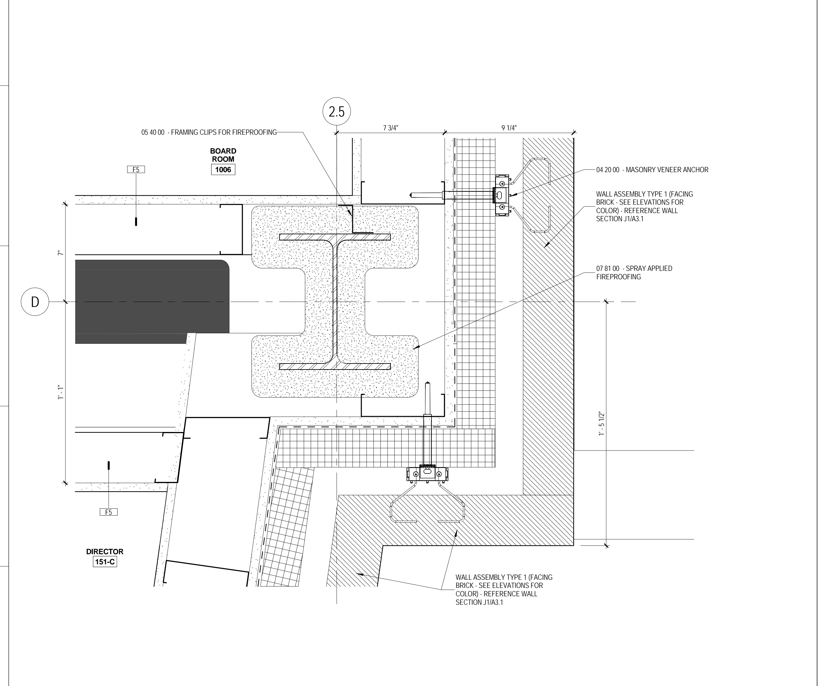
J1 PLAN DETAIL @ BOARD ROOM 1101 A5.9 3" = 1'-0"
