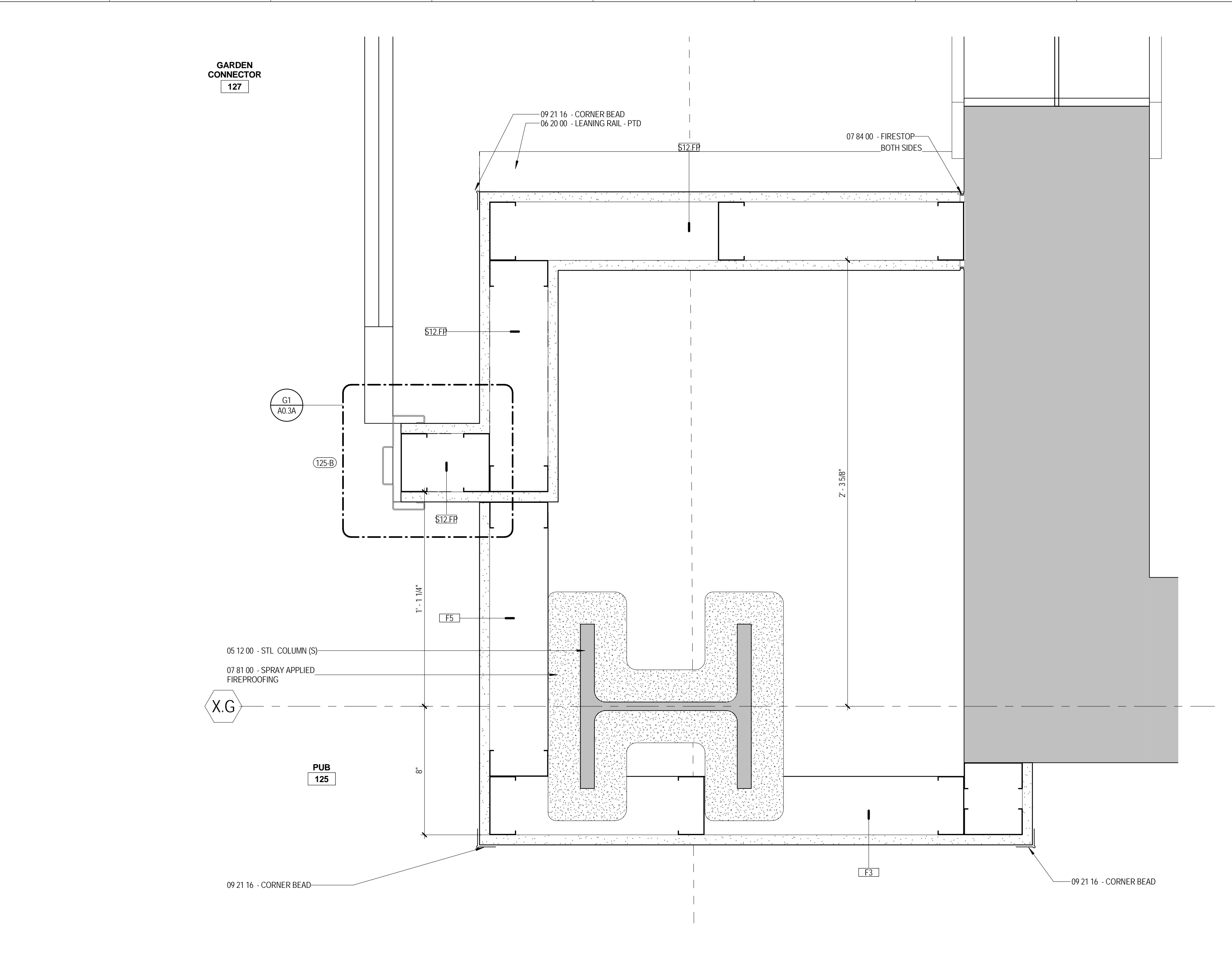
F7 PLAN DETAIL @ PUB 125 A5.9 3" = 1'-0"
