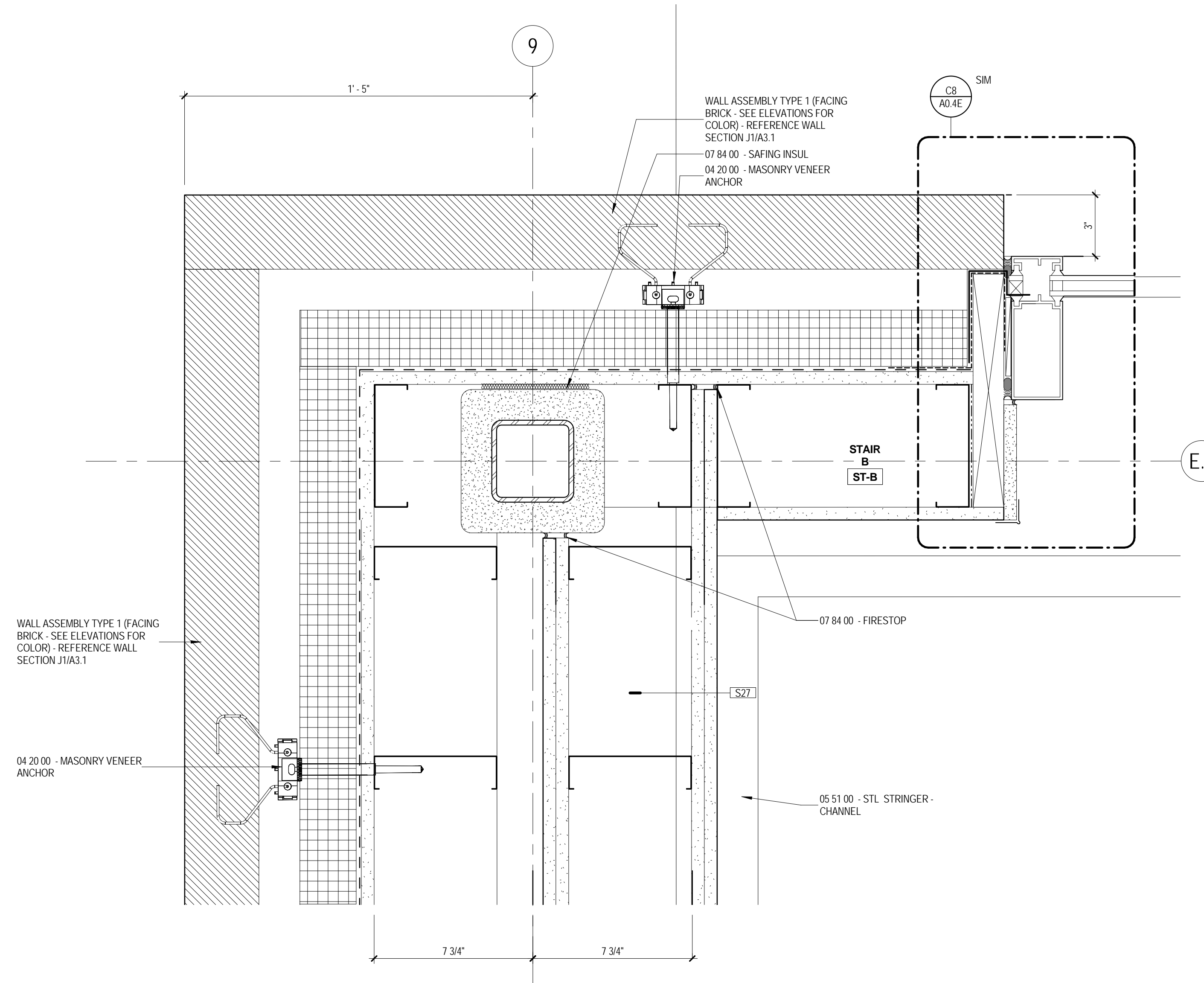
J9 PLAN DETAIL LEVEL 5 - STAIR B A5.6 3" = 1'-0"
