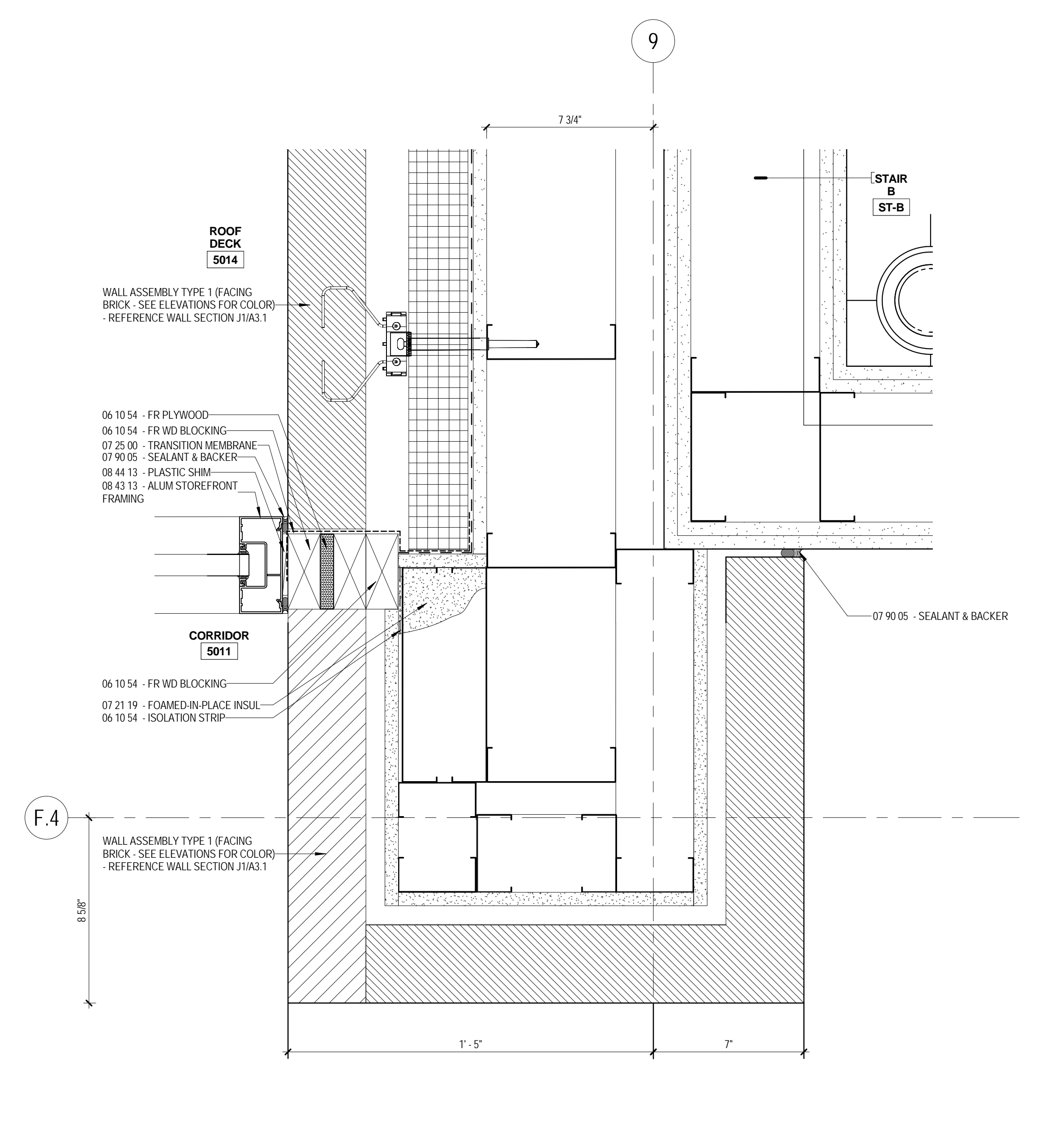
E10 NEW BUILDING - LEVEL 5 - CORRIDOR 5012 A5.6 3" = 1'-0"
