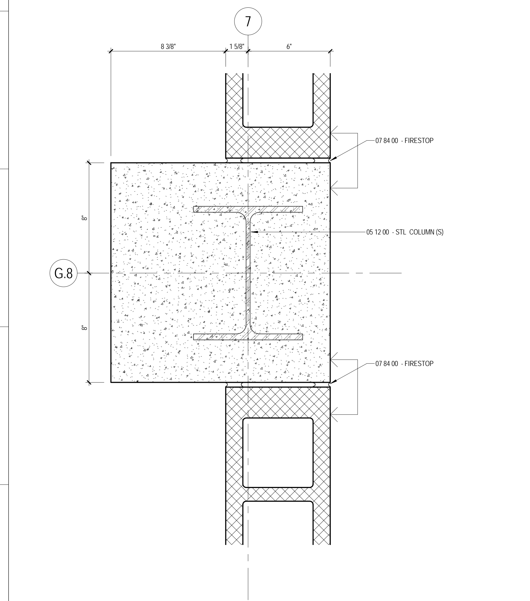
E1 PLAN DETAIL GARAGE LEVEL @ TRASH COLLECTION G011 A5.6 3" = 1'-0"
