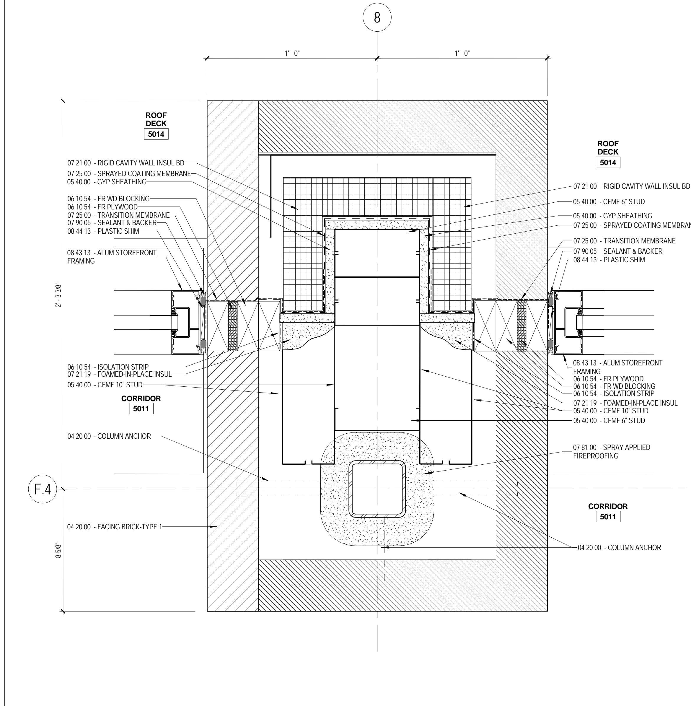
E5 BLDG C - CORRIDOR PILASTER DETAIL @ LEVEL 5 ROOF DECK A5.6 3" = 1'-0"
