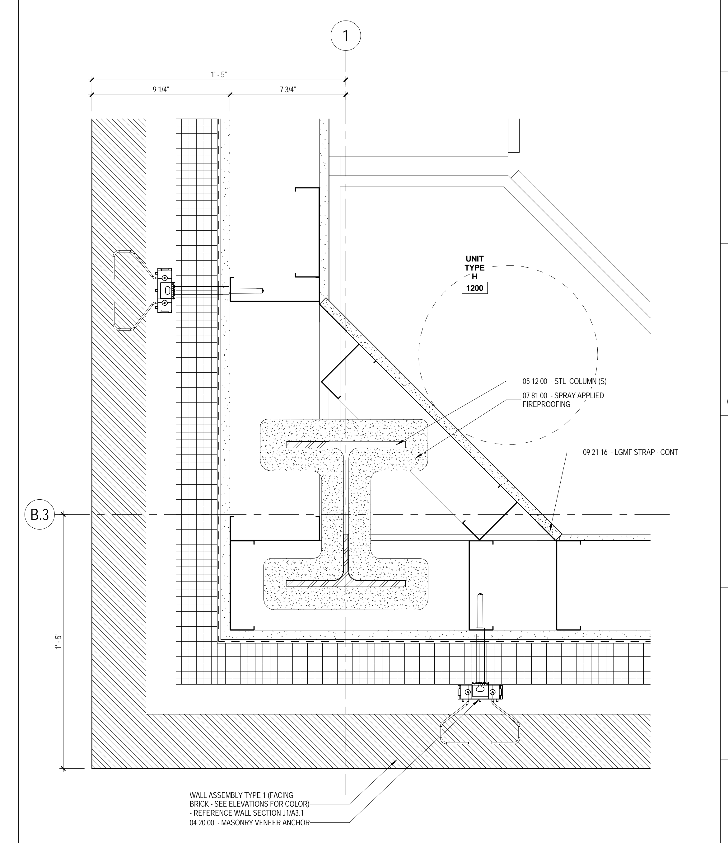
J10 PLAN DETAIL @ UNIT TYPE H 1200 KITCHEN A5.5 3" = 1'-0"
