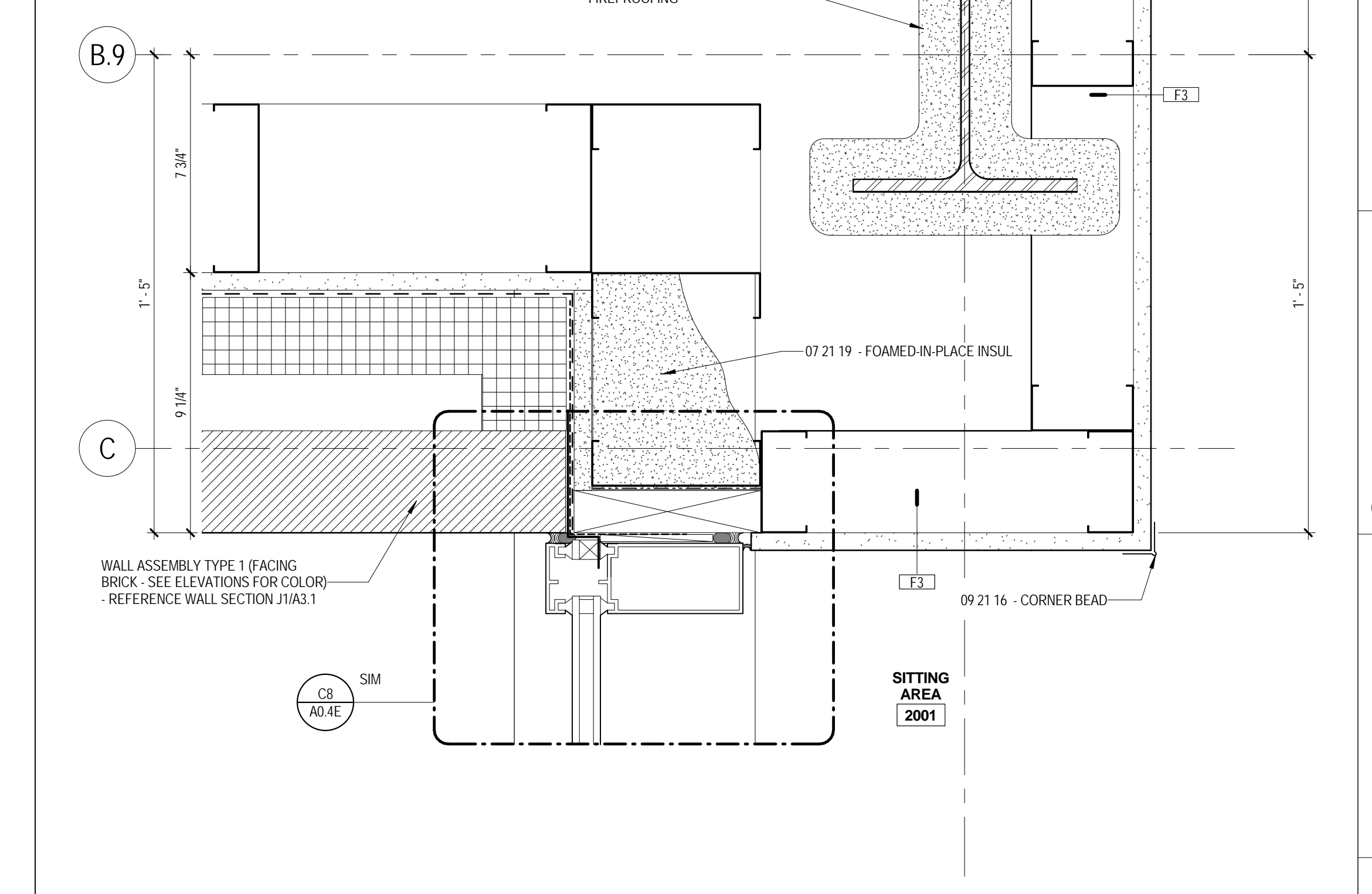
E10 PLAN DETAIL LEVEL 2 - SITTING AREA 2001 A5.5 3" = 1'-0"
