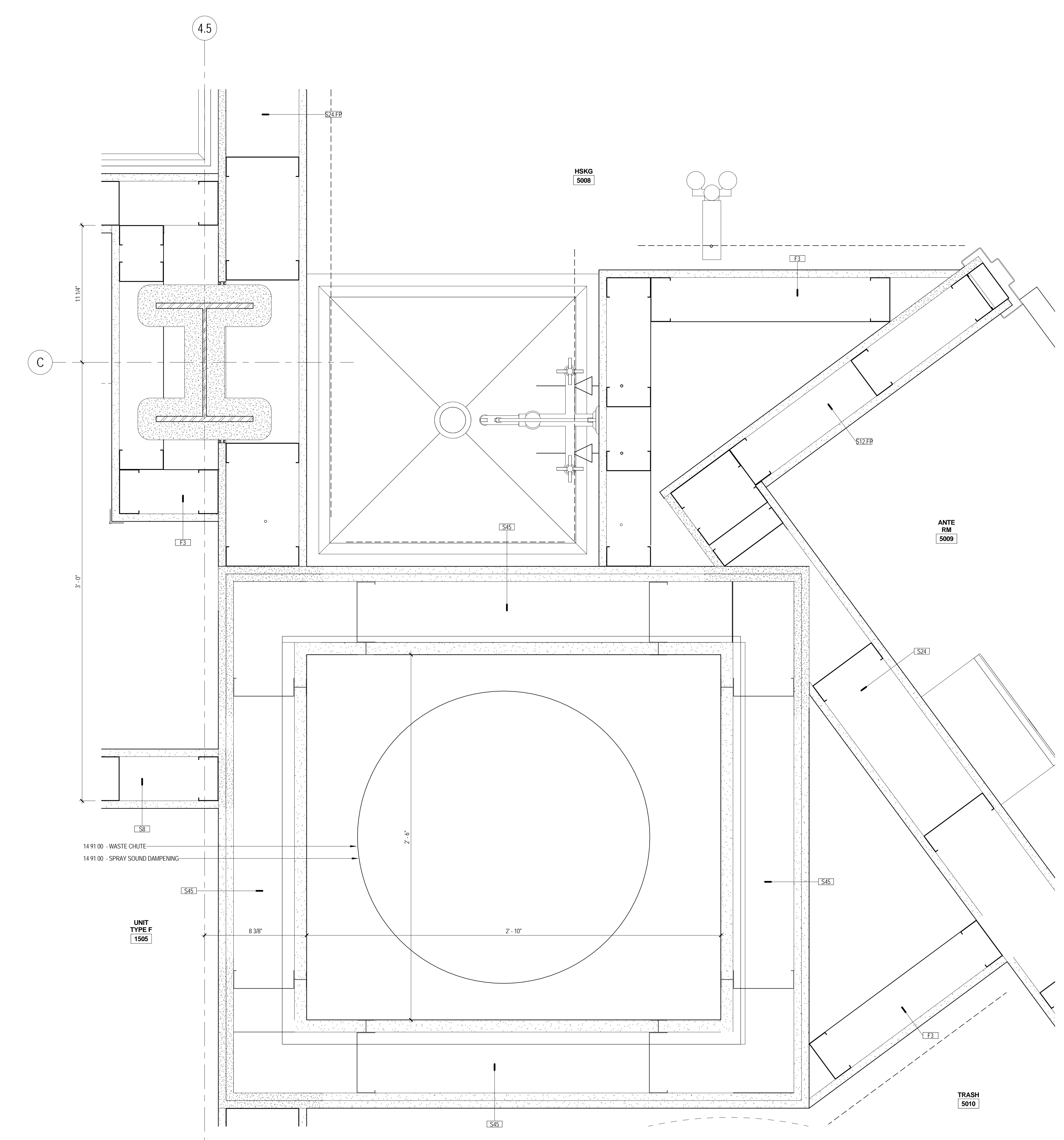
J1 PLAN DETAIL @ INTERIOR TRASH SHUTE A5.5 3" = 1'-0"
