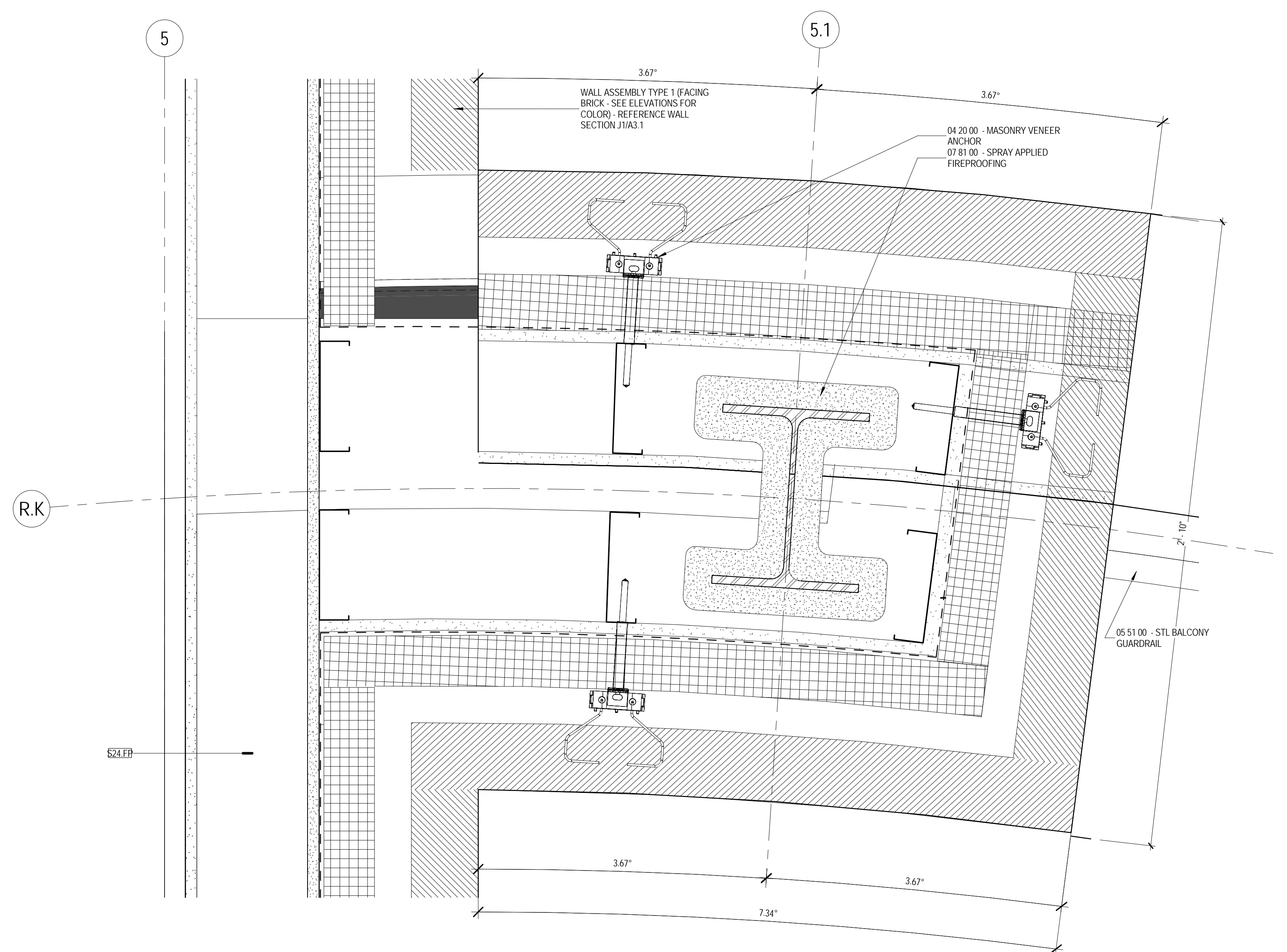
J1 PLAN DETAIL LEVEL 3 @ COMMUNITY DECK 1322A A5.3 3" = 1'-0"
