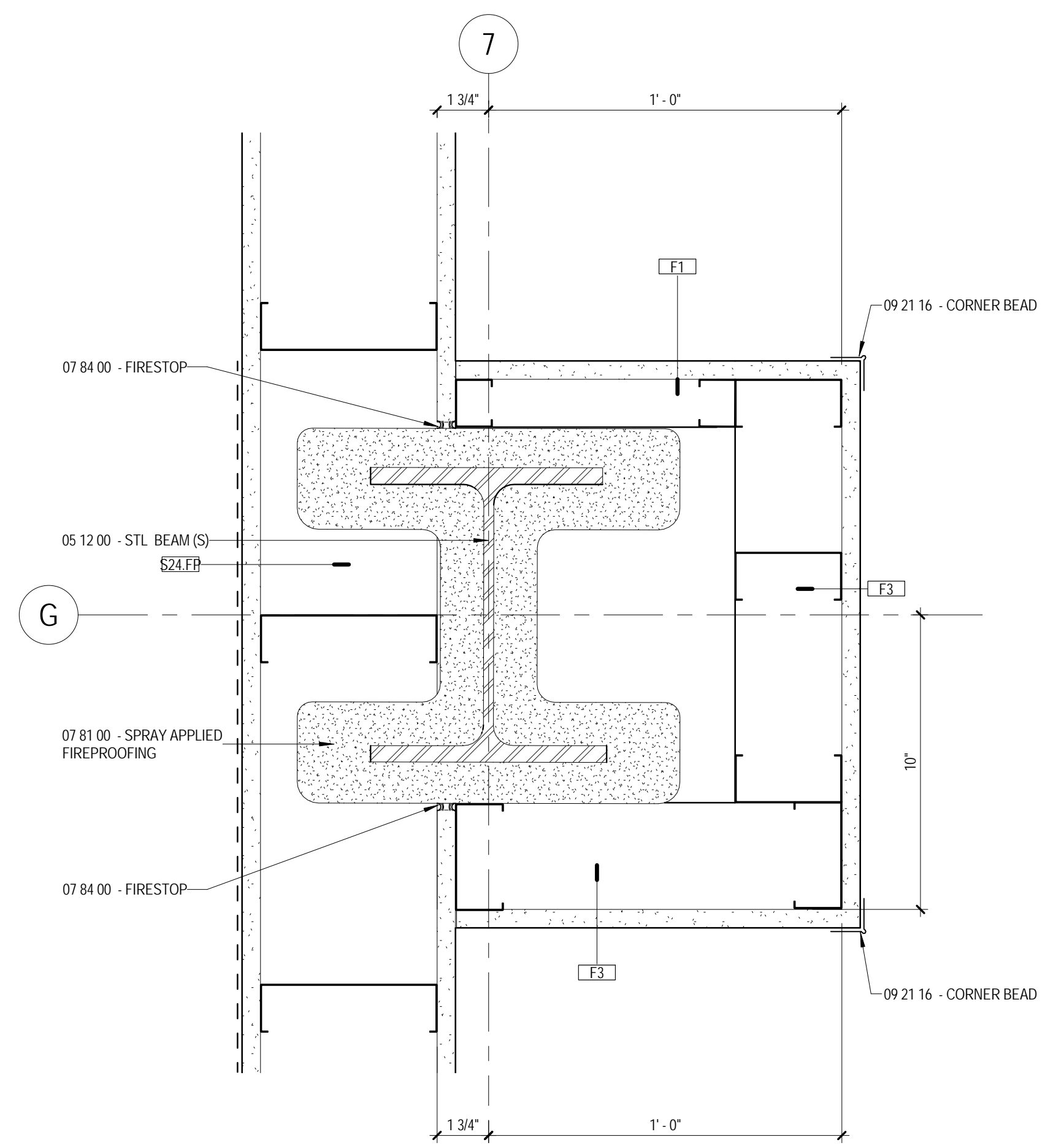
E1 PLAN DETAIL @ UNIT TYPE E 1207 KITCHEN A5.3 3" = 1'-0"
