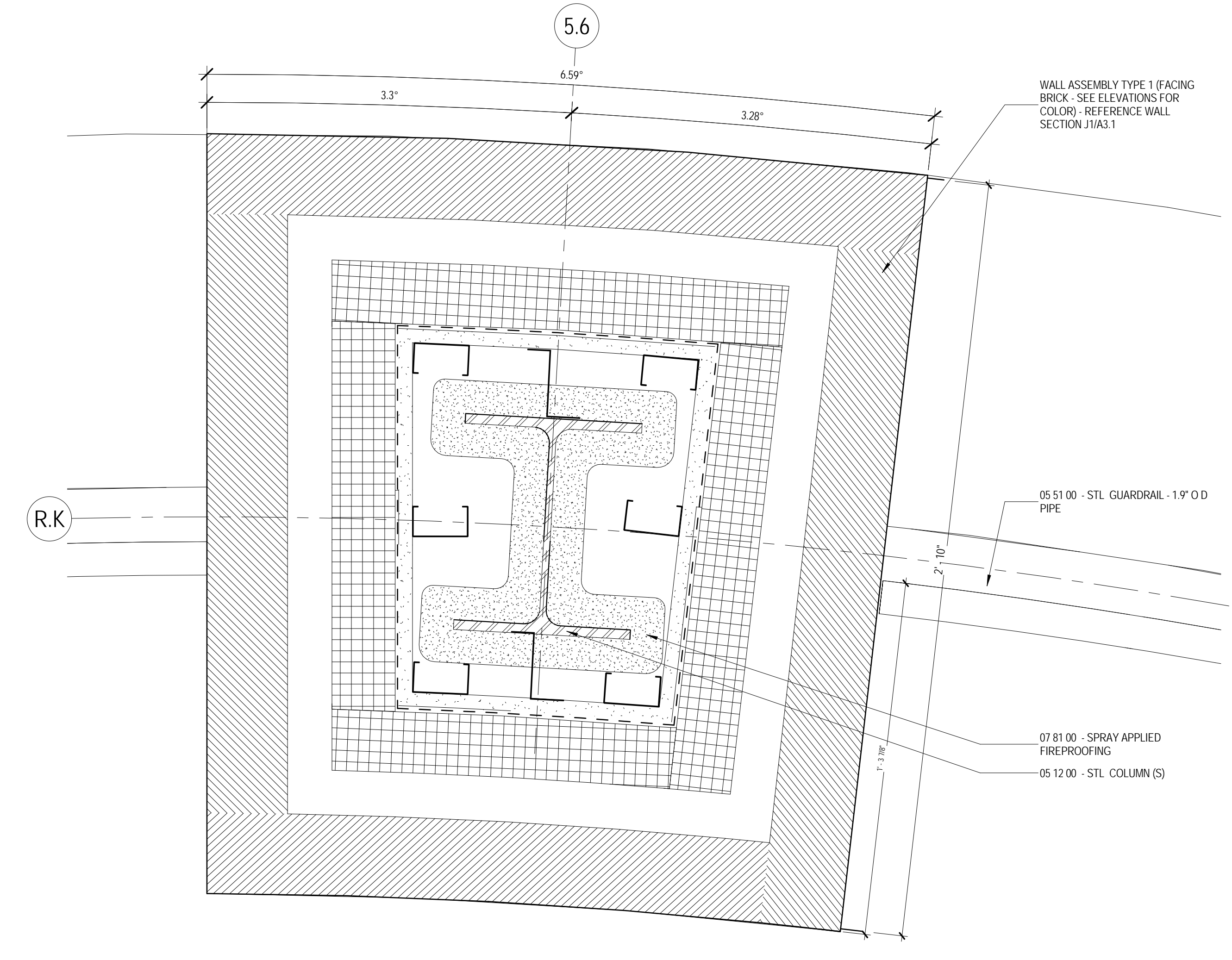
J9 PLAN DETAIL @ COMMUNITY DECK 3004 RAILING AND BRICK PIER A5.3 3" = 1'-0"
