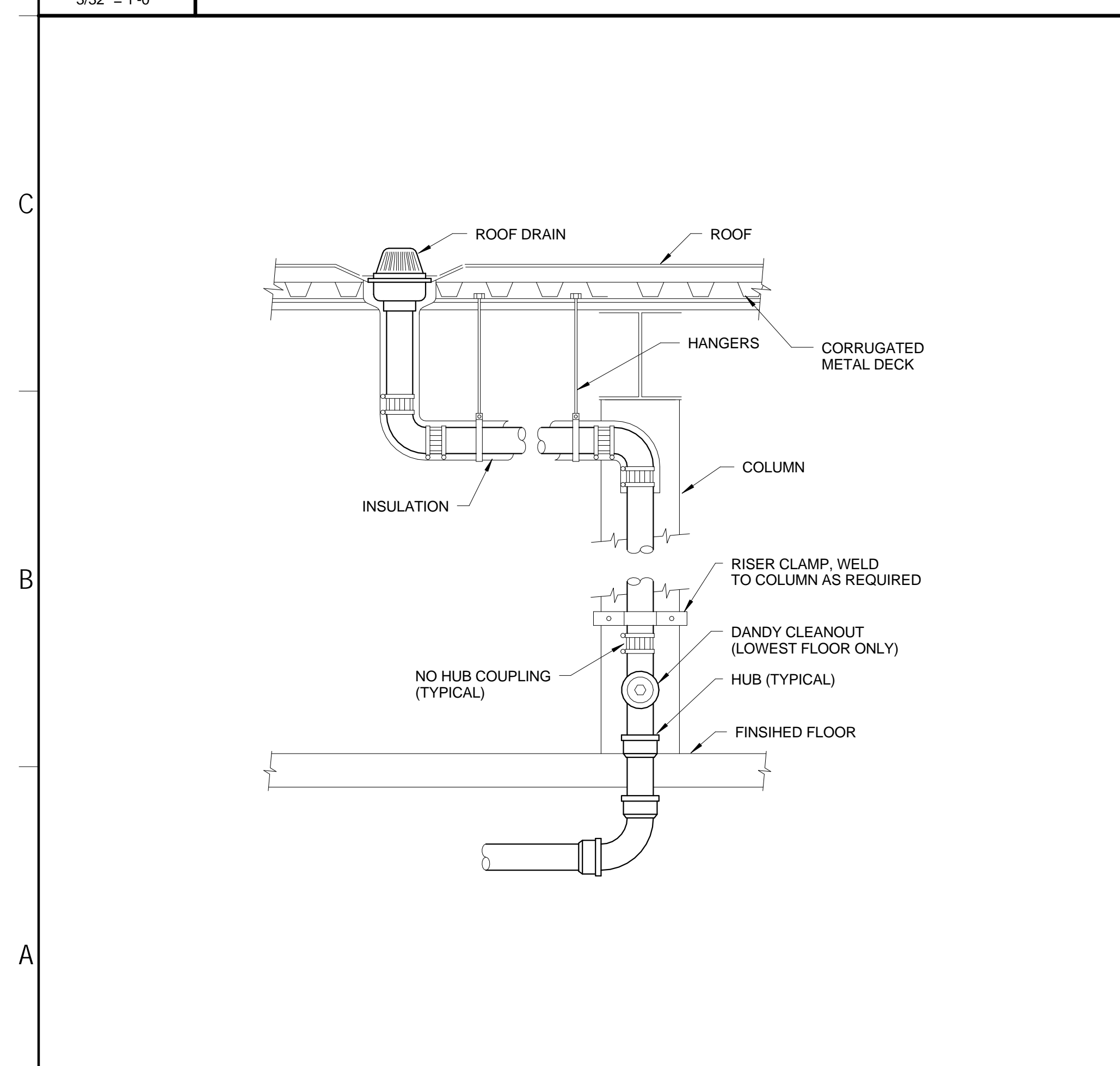
A1 DETAIL - ROOF DRAIN PIPING NOT TO SCALE
