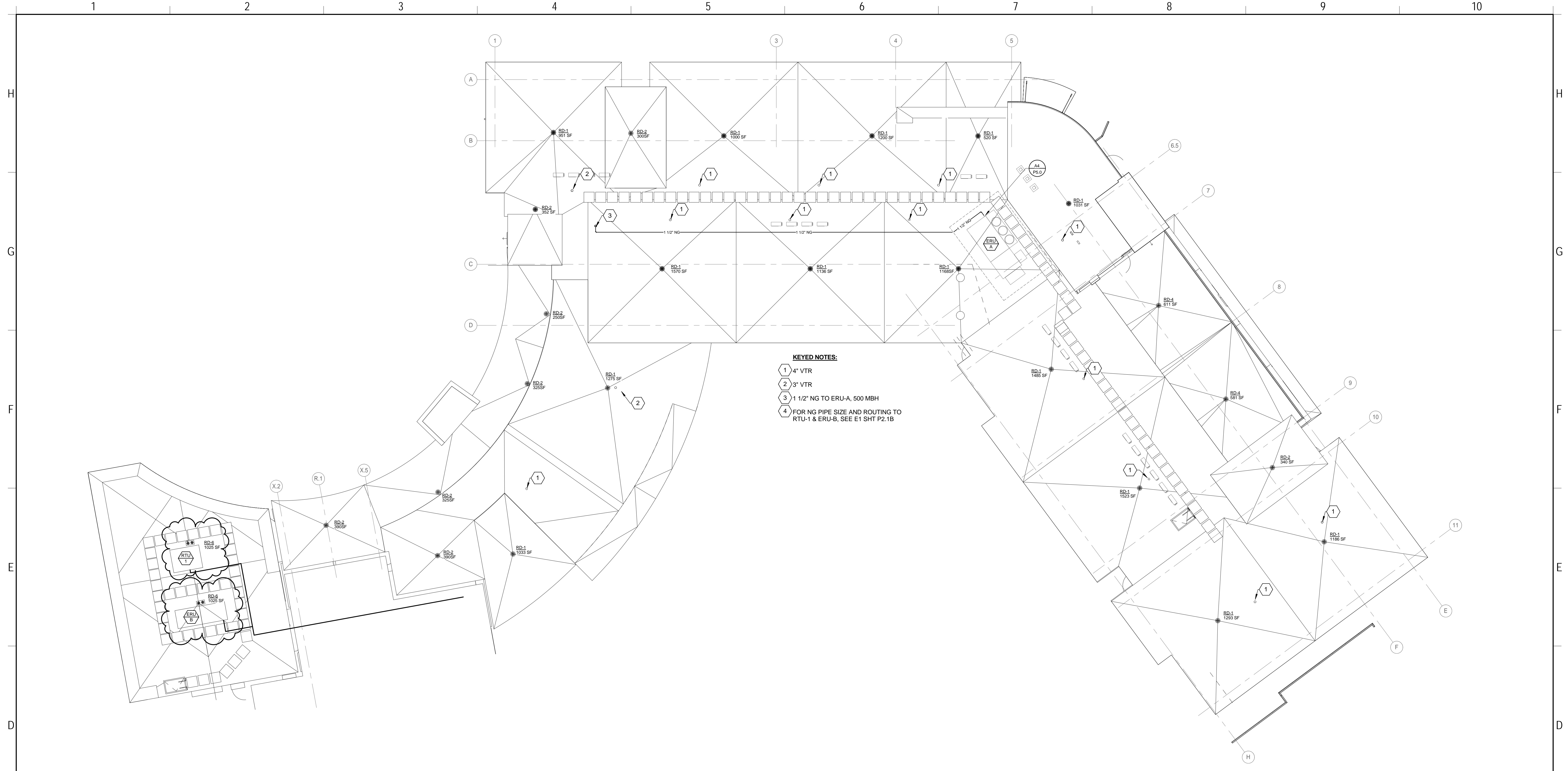
D1 MECHANICAL PLAN - ROOF - NEW BUILDING 3/32" = 1'-0"
