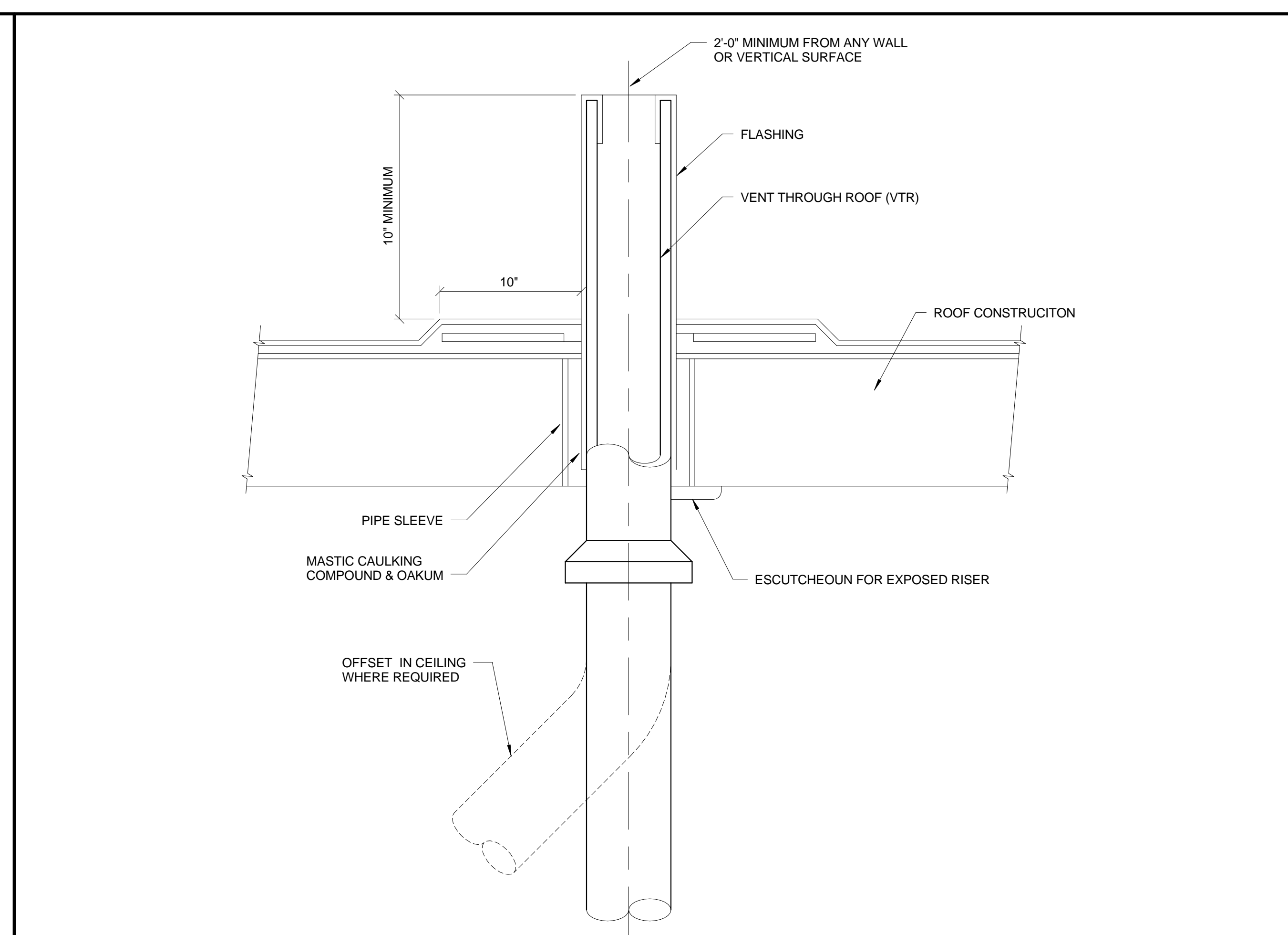
A4 DETAIL - GAS EQUIPMENT CONNECTION NOT TO SCALE
