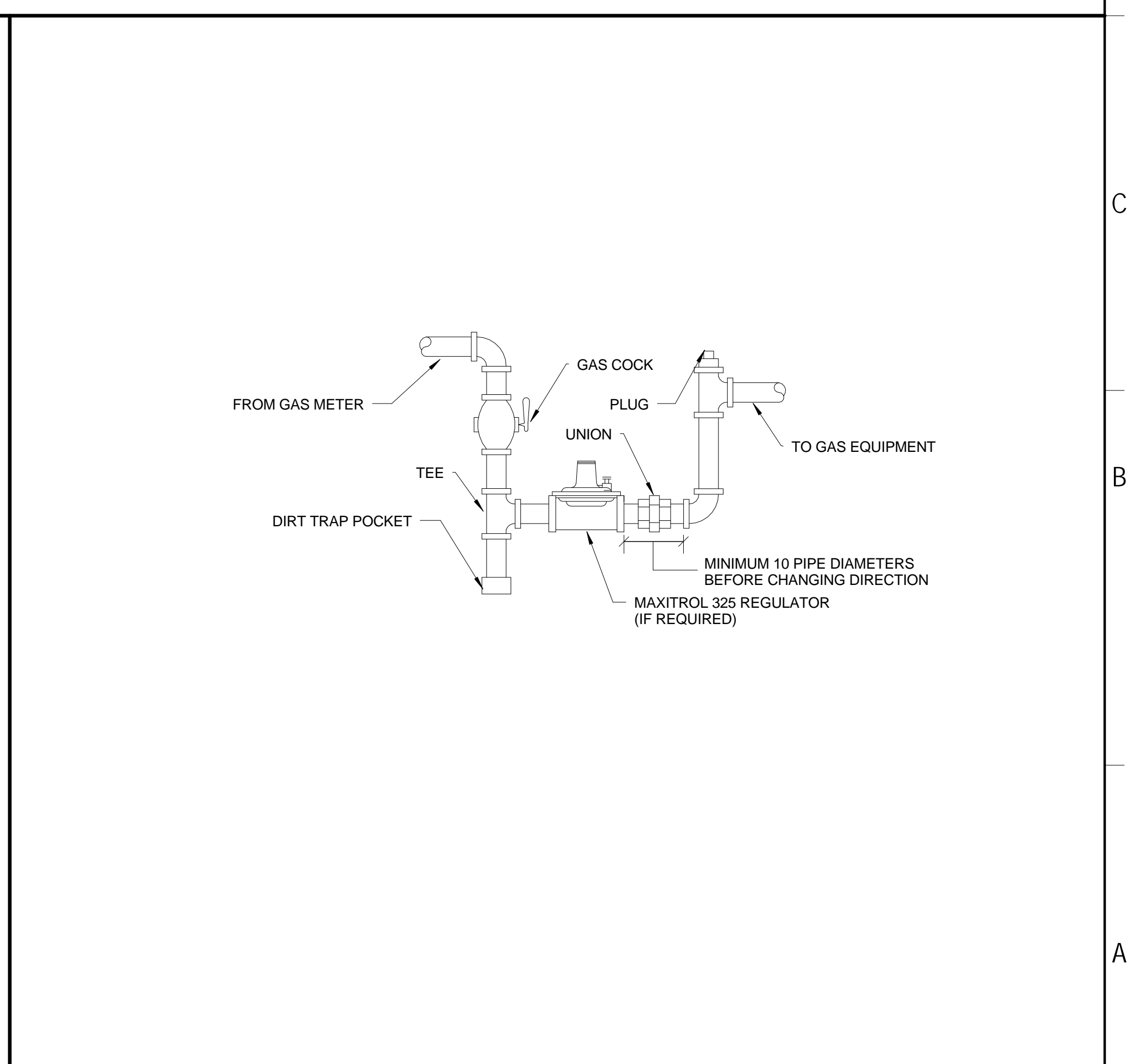
A8 DETAIL - GAS EQUIPMENT CONNECTION NOT TO SCALE
