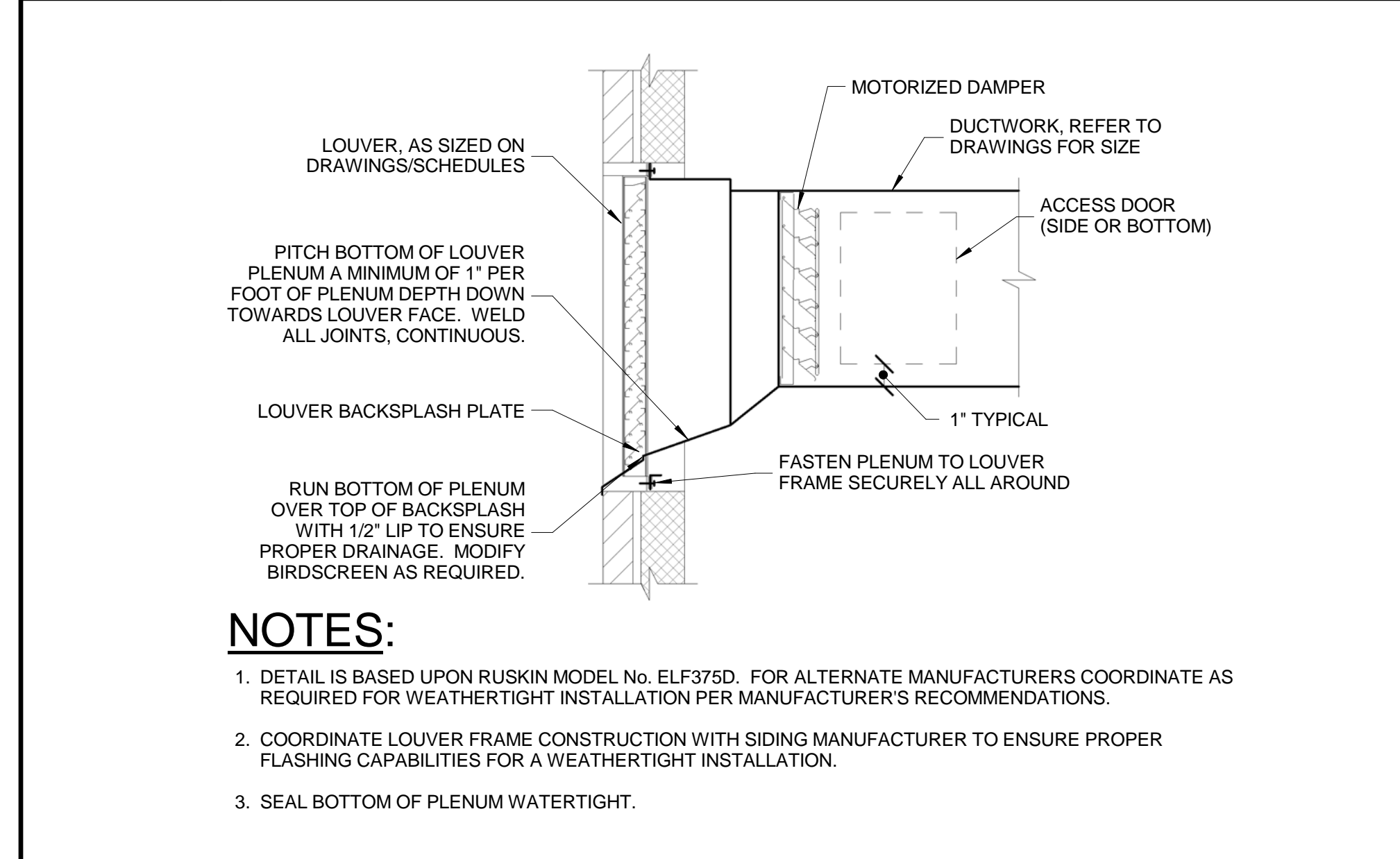
A4 DETAIL - EXTERIOR LOUVER NOT TO SCALE
