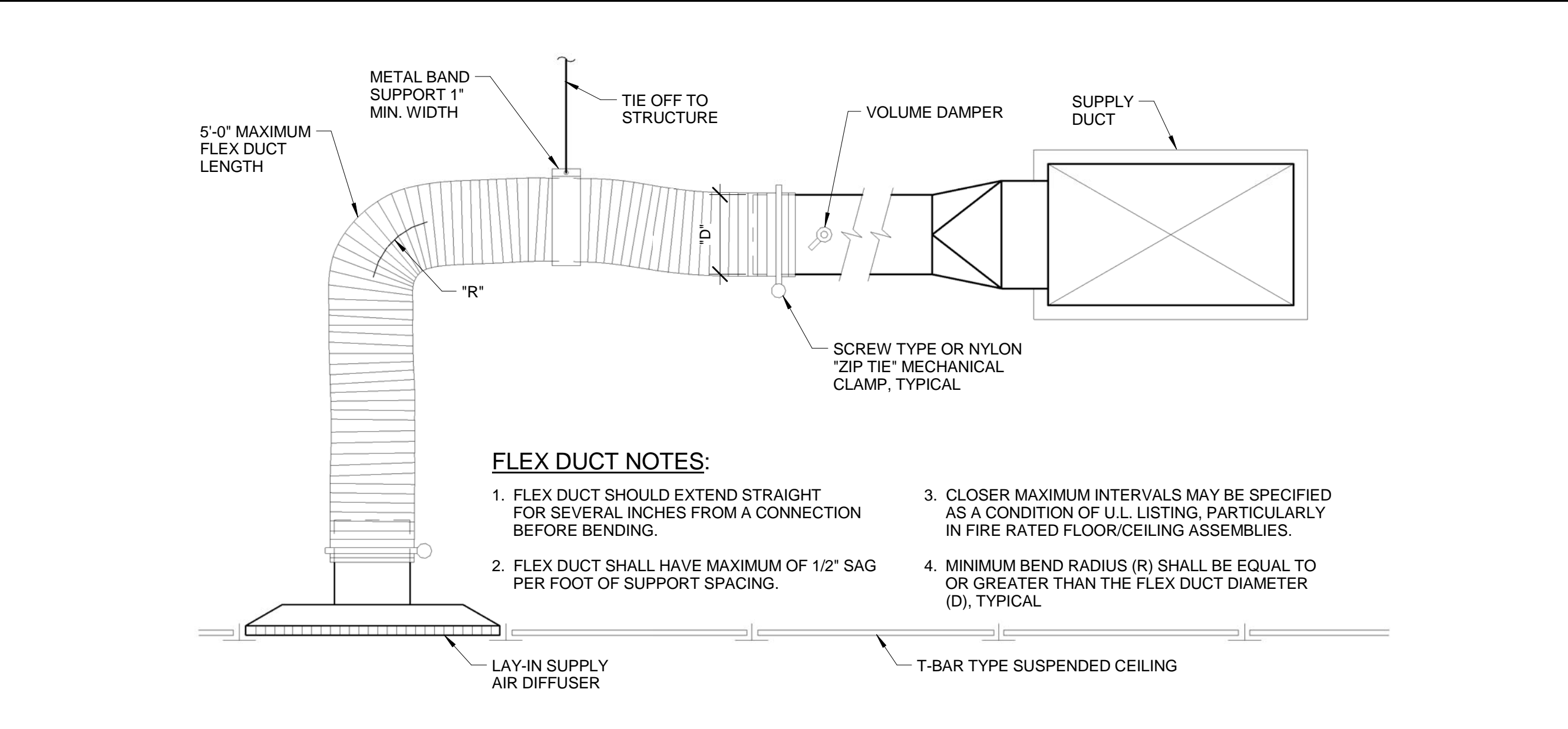
C7 DETAIL - SUPPLY AIR BRANCH CONNECTION NOT TO SCALE
