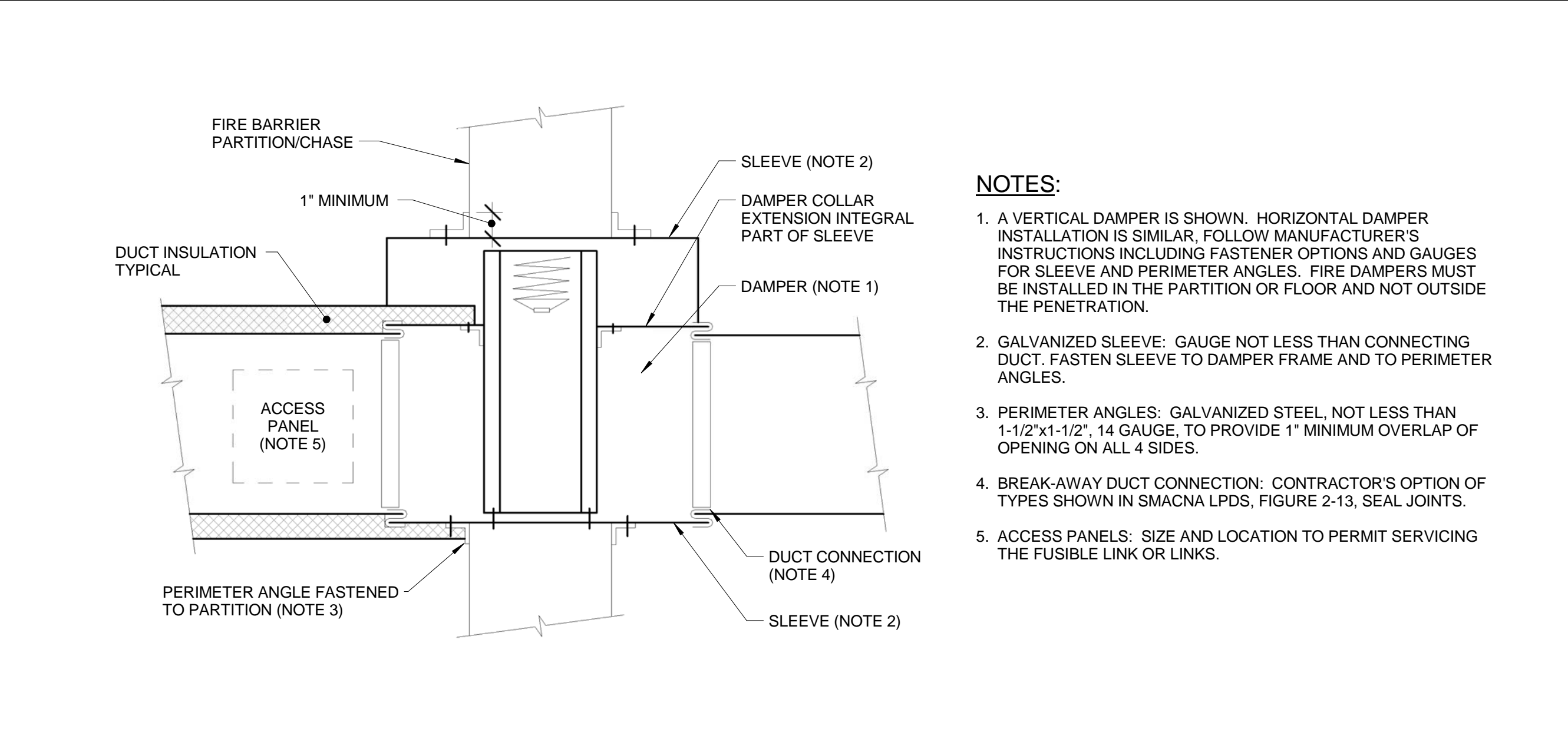
A7 DETAIL - TYPICAL FIRE DAMPER NOT TO SCALE
