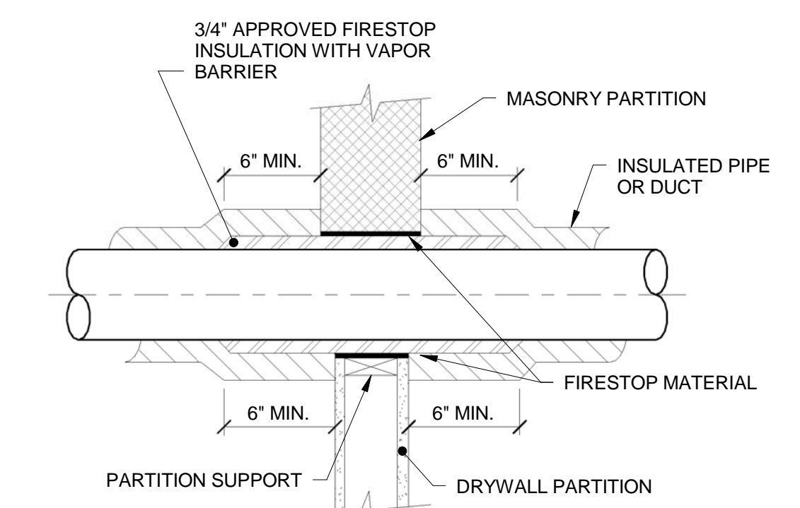
PARTITION OR CHASE PENETRATION
