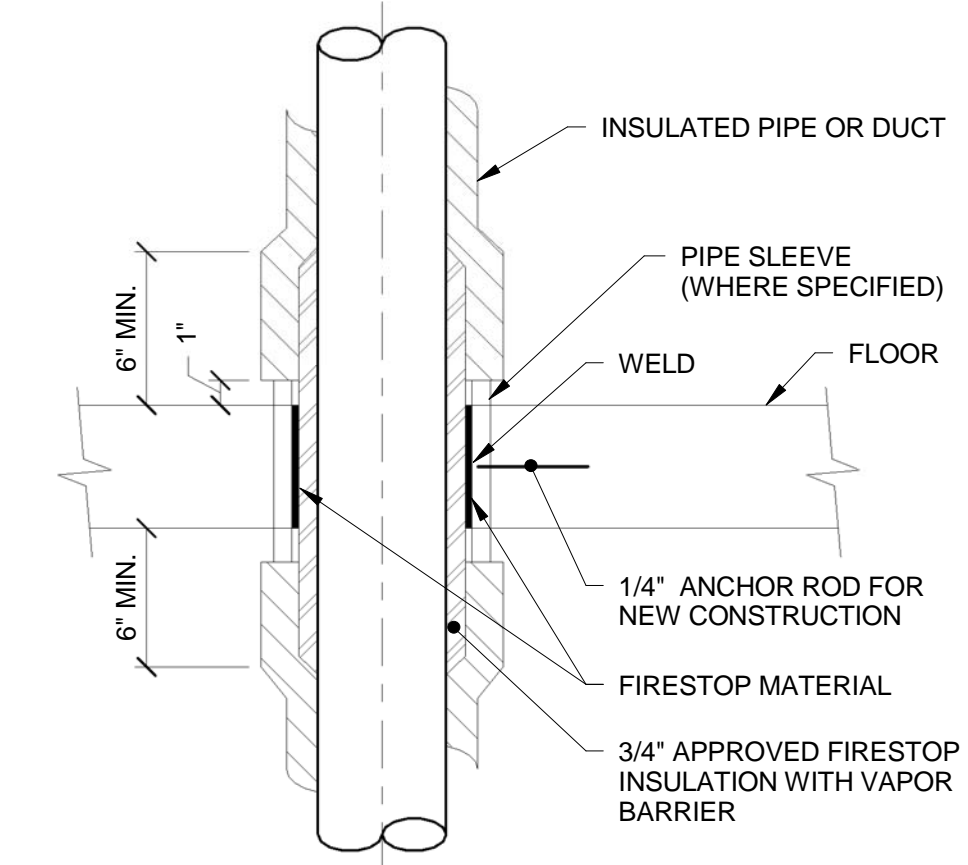
FLOOR OR DECK PENETRATION
