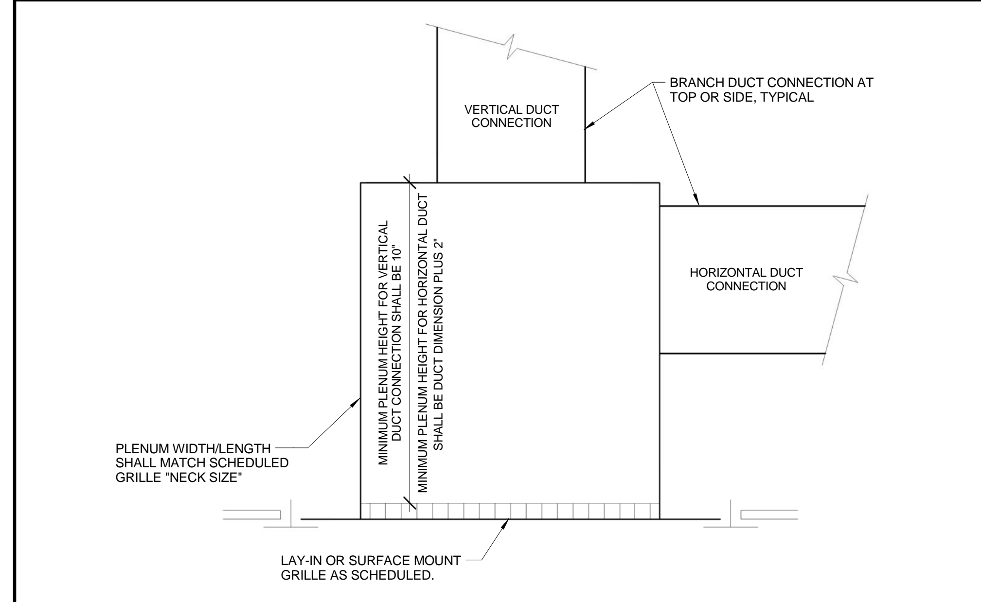
C4 DETAIL - SUPPLY/RETURN AIR REGISTER BOOT NOT TO SCALE
