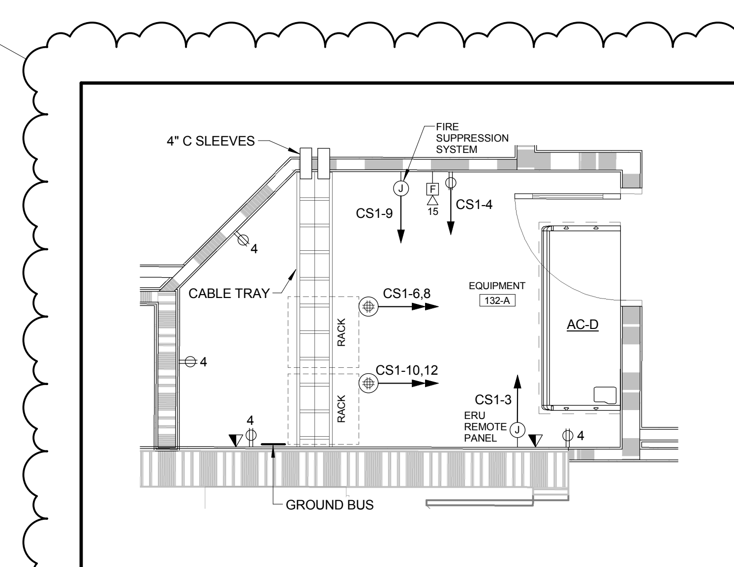
A9 ENLARGED EQUIPMENT/SERVER ROOM 132-A 3/8" = 1'-0"
