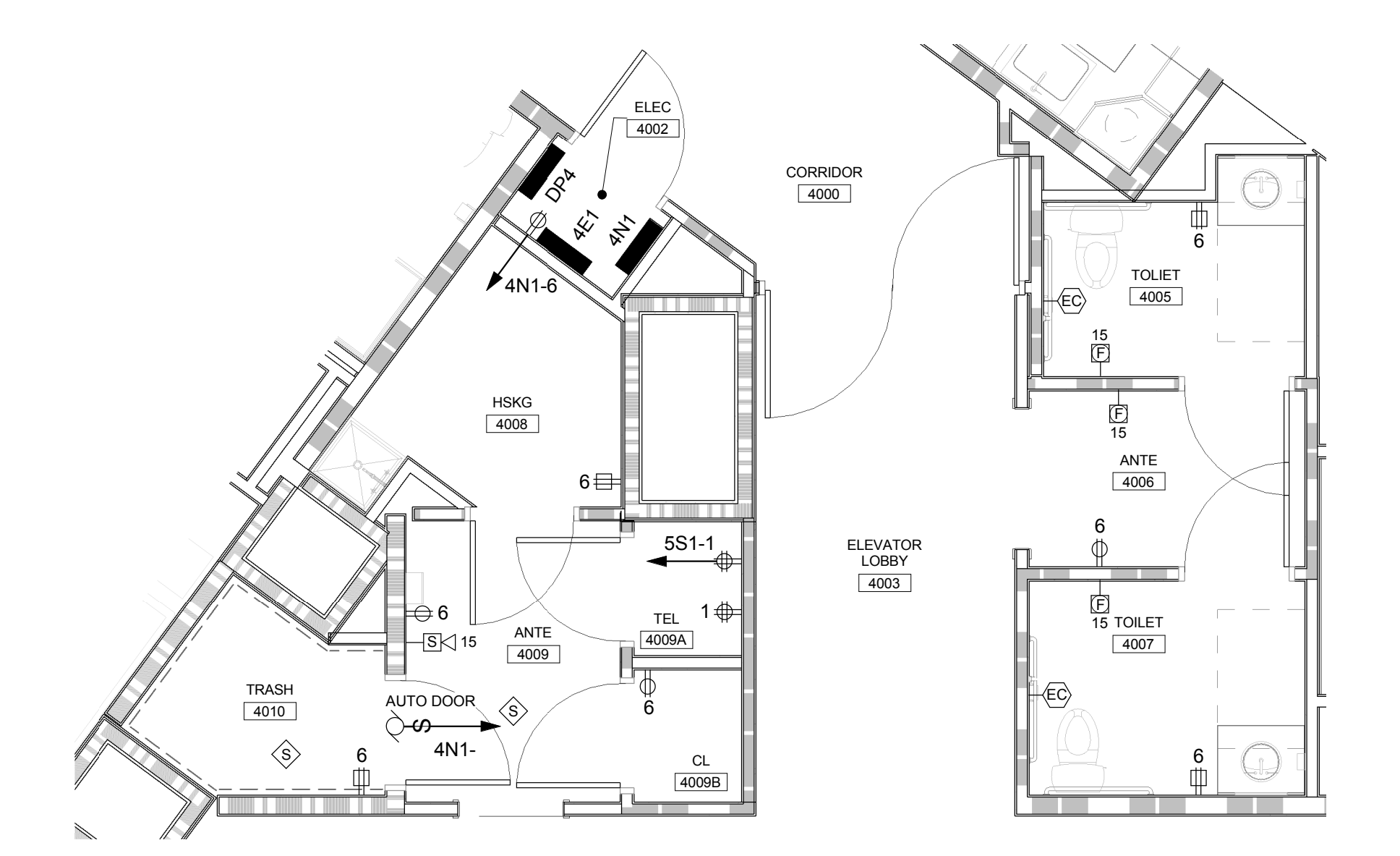
A1 ENLARGED LEVEL 4 PART PLAN 1/4" = 1'-0"
