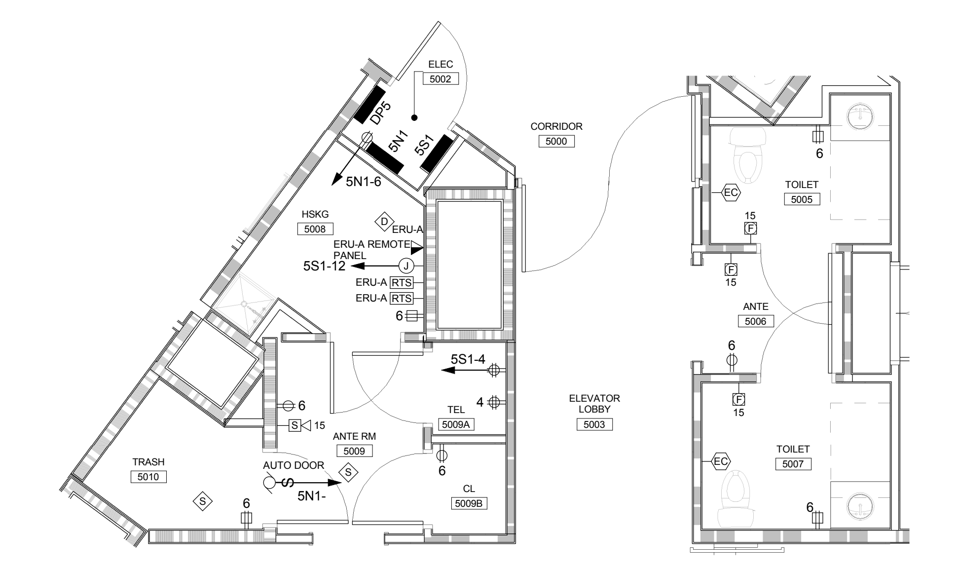
C1 ENLARGED LEVEL 5 PART PLAN 1/4" = 1'-0"
