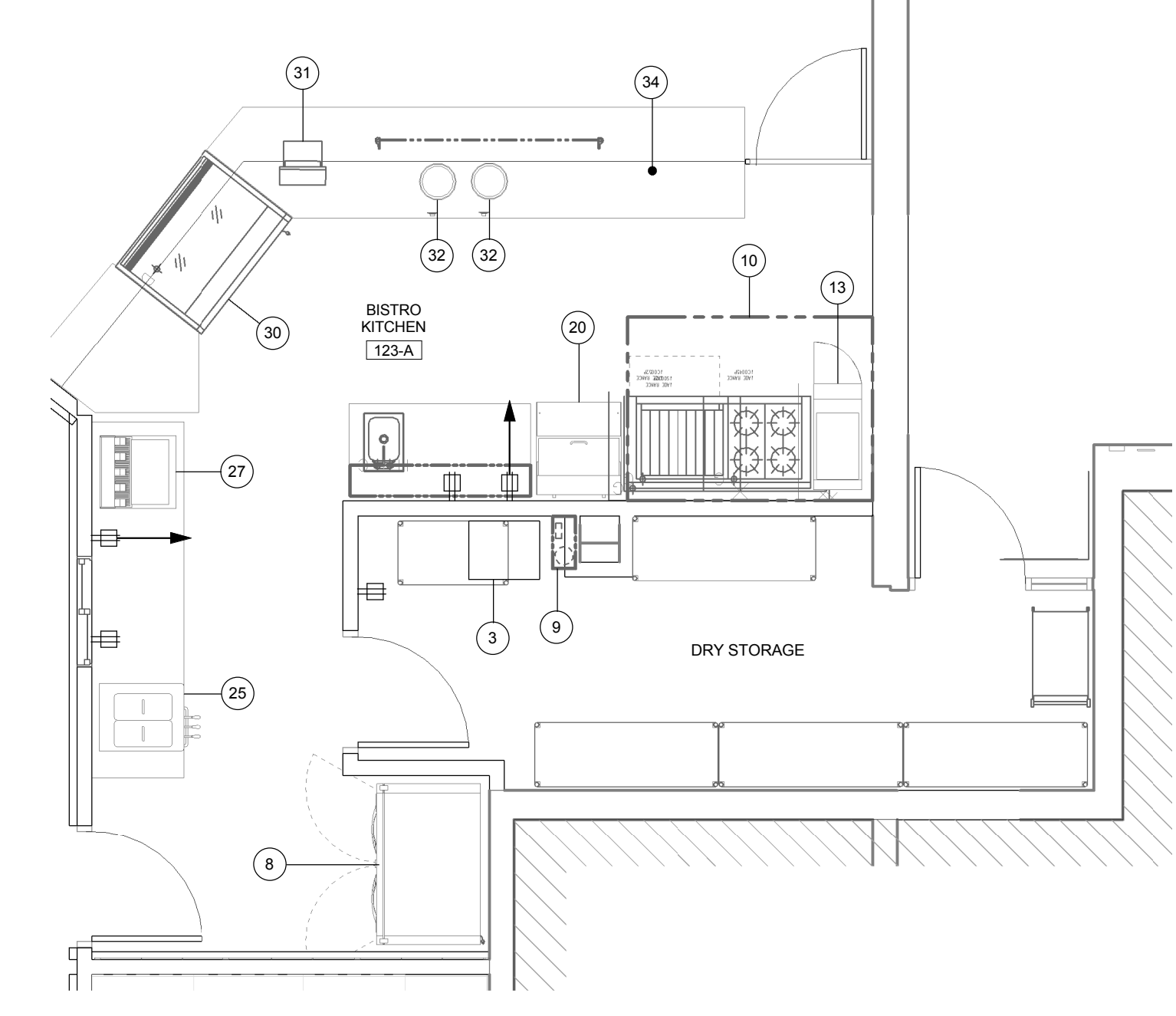
A8 ENLARGED BISTRO KITCHEN PLAN 1/4" = 1'-0"
