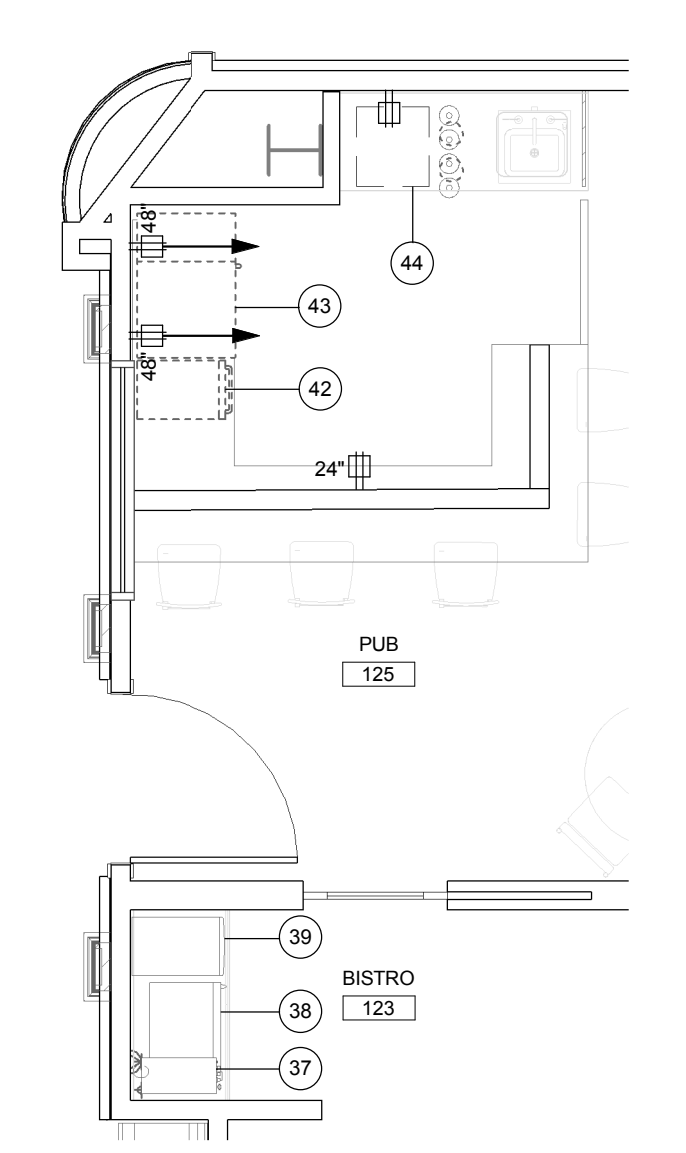
A6 ENLARGED BAR/BISTRO PLAN 1/4" = 1'-0"
