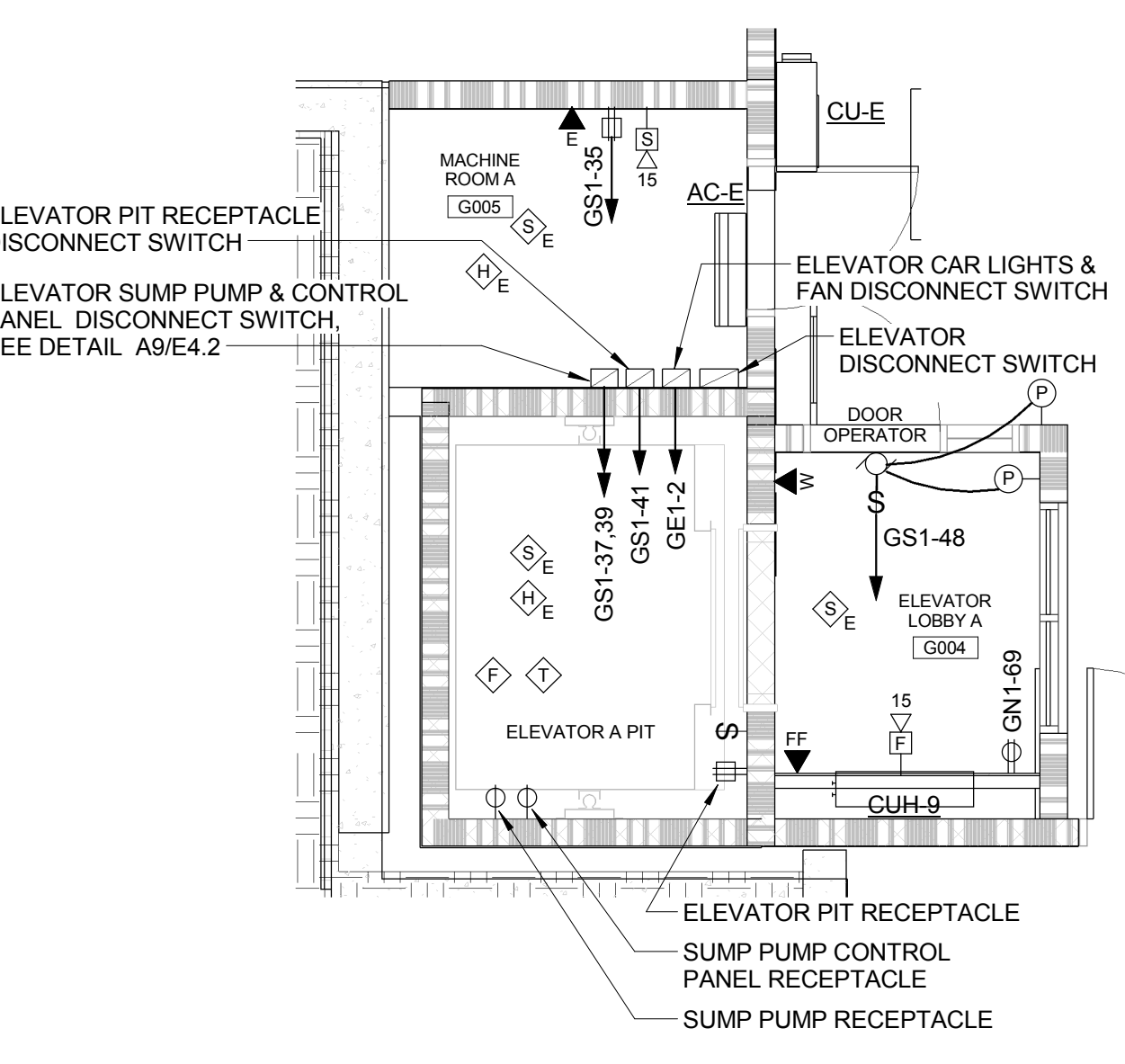
A4 ELEVATOR A PLAN 1/4" = 1'-0"
