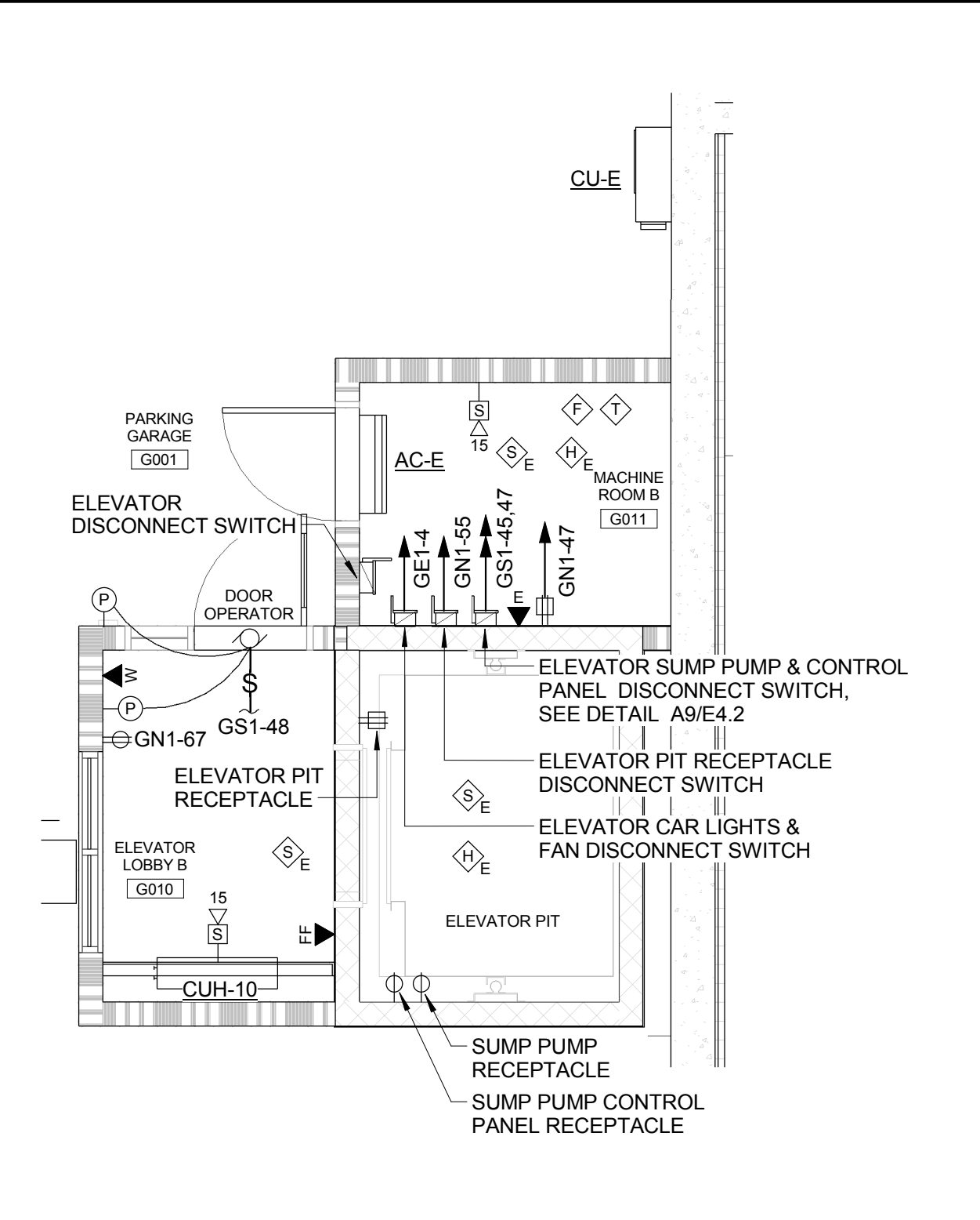
C4 ELEVATOR B PLAN 1/4" = 1'-0"
