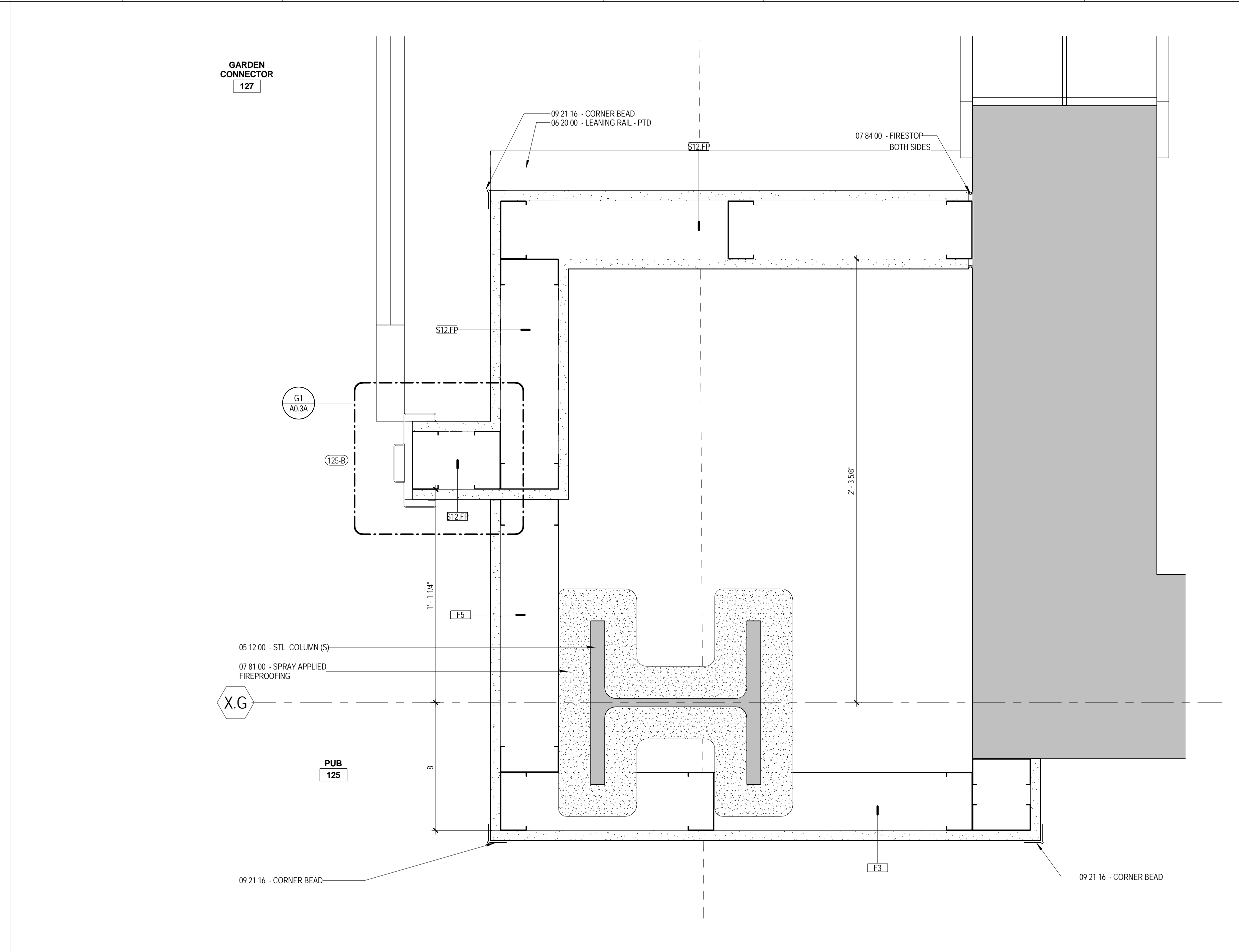
F7 PLAN DETAIL @ PUB 125 A5.9 3" = 1'-0"
