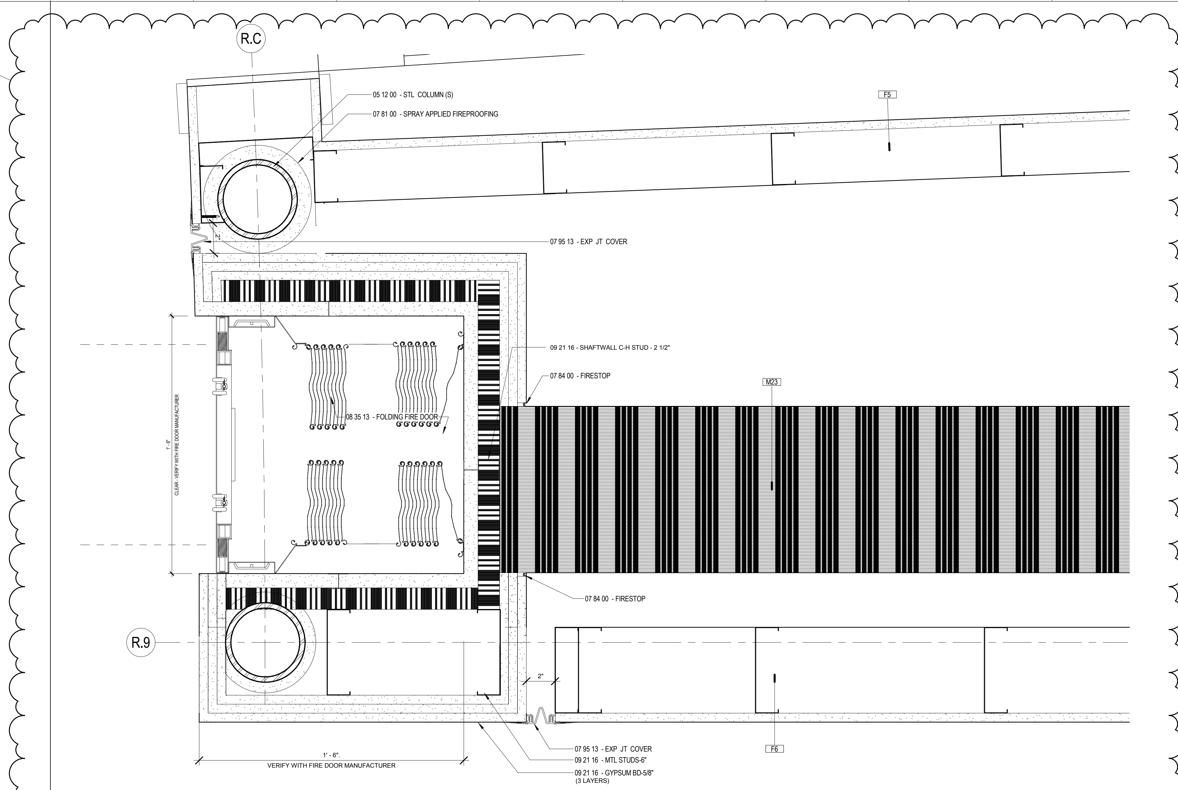
E6 PLAN DETAIL @ WON DOOR POCKET A5.8 3" = 1'-0"
