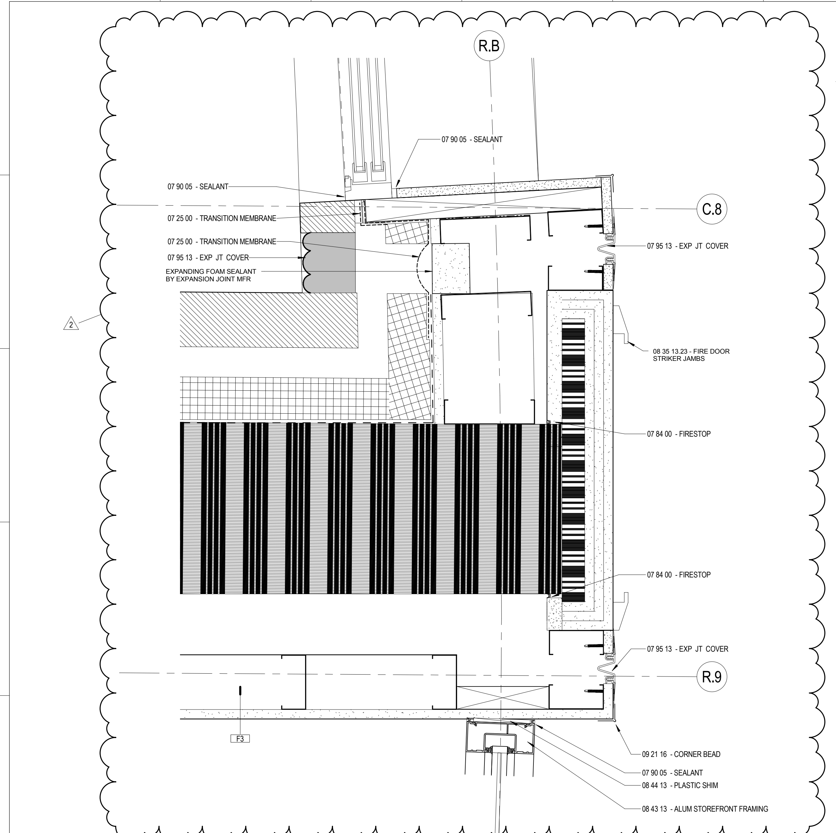
E1 PLAN DETAIL @ WON DOOR RECEIVER A5.8 3" = 1'-0"
