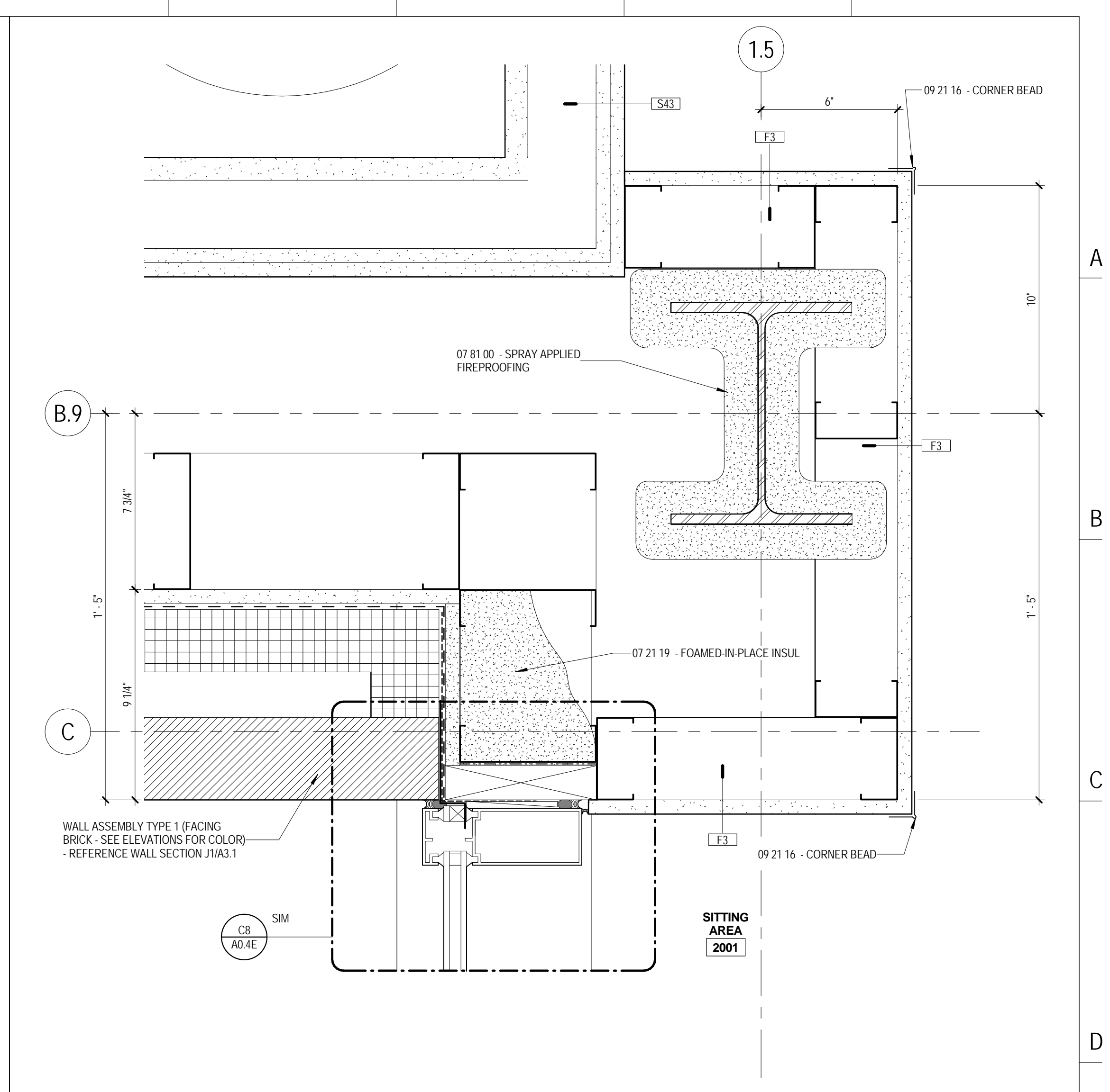
E10 PLAN DETAIL LEVEL 2 - SITTING AREA 2001 A5.5 3" = 1'-0"
