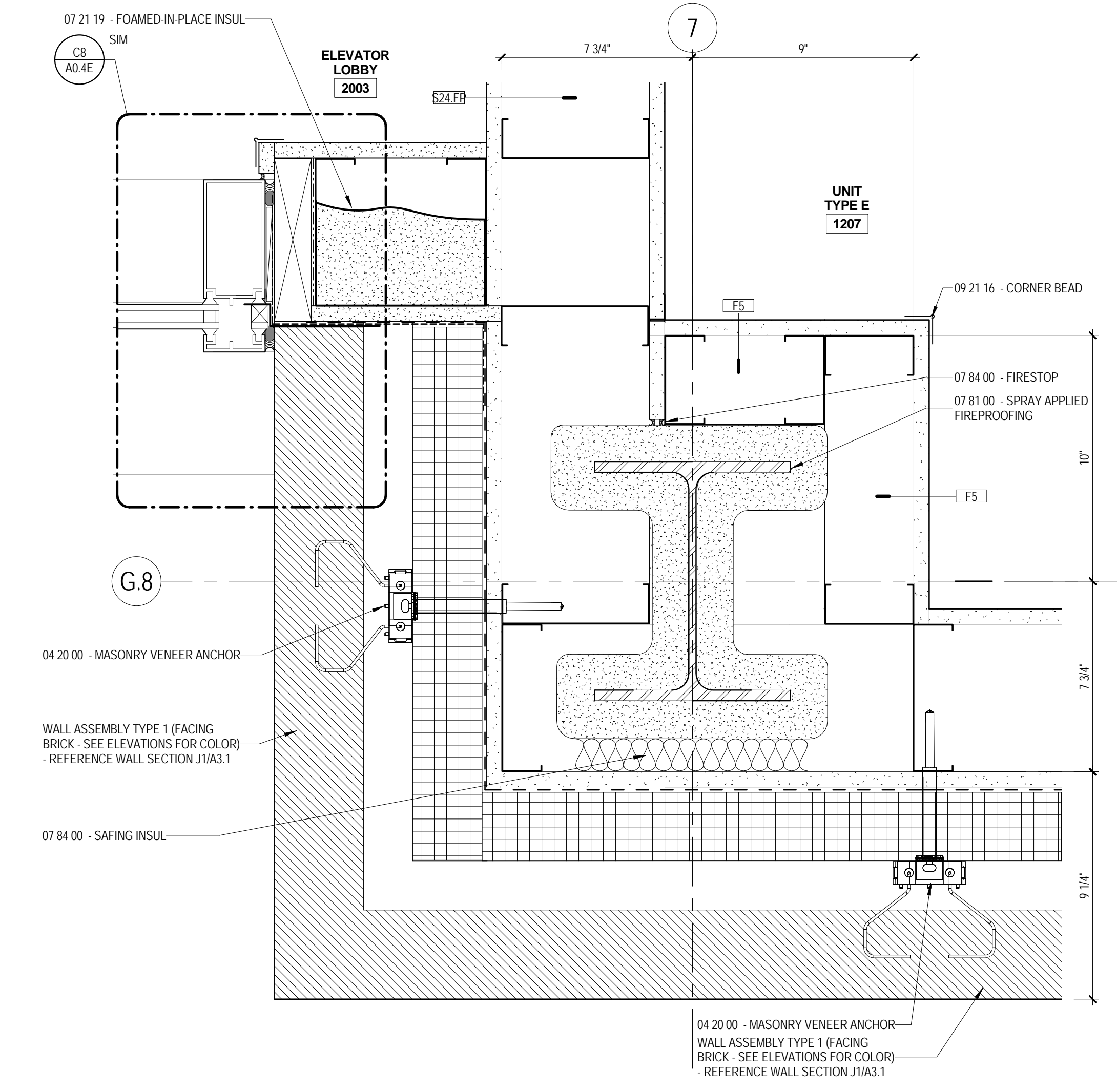
J8 PLAN DETAIL LEVEL 2 - ELEVATOR LOBBY 2003 A5.4 3" = 1'-0"
