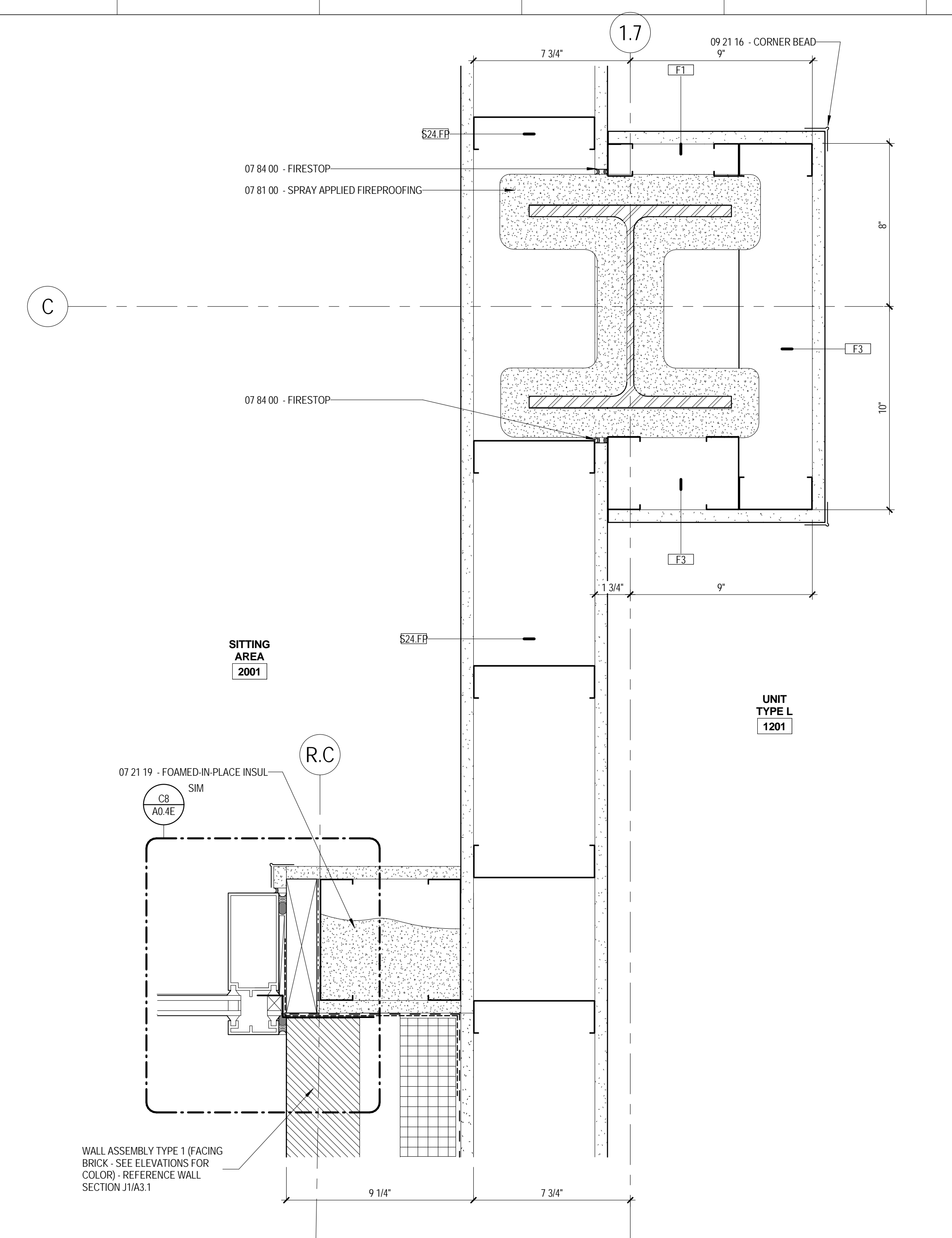
F8 PLAN DETAIL LEVEL 2 - SITTING AREA 2001 A5.4 3" = 1'-0"
