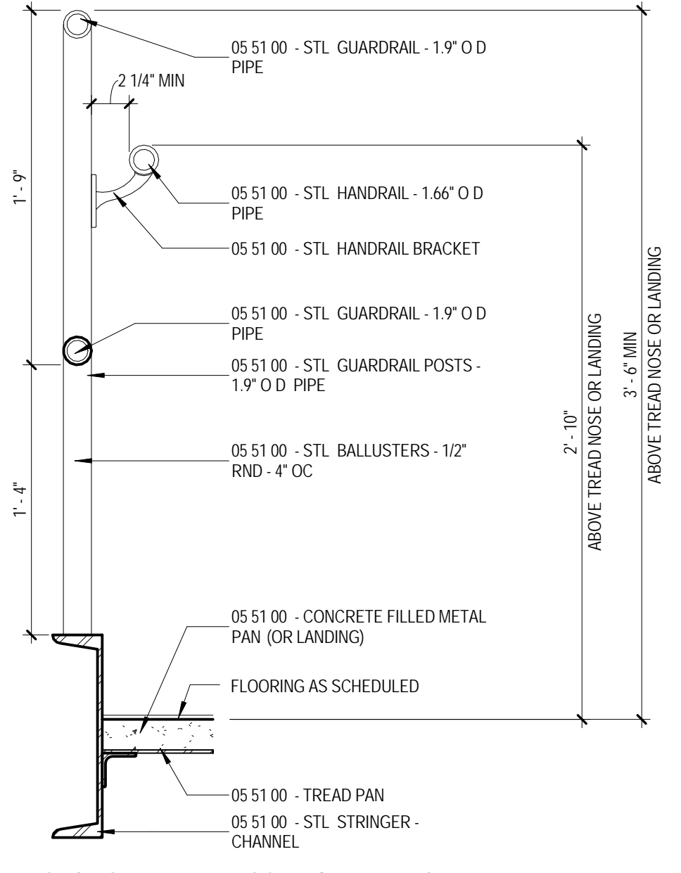
H7 STAIR SECTION DETAIL at OSHA GUARD and HANDRAIL (CHANNEL STRINGER) A4.9 1/12" = 1'-0"
