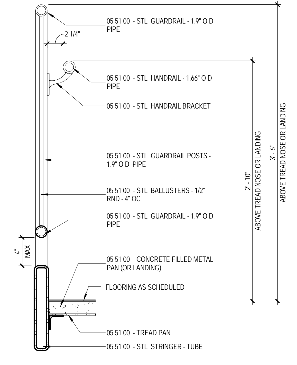
H1 STAIR DETAIL at GUARDRAIL AND HANDRAIL A4.9 1/12" = 1'-0"
