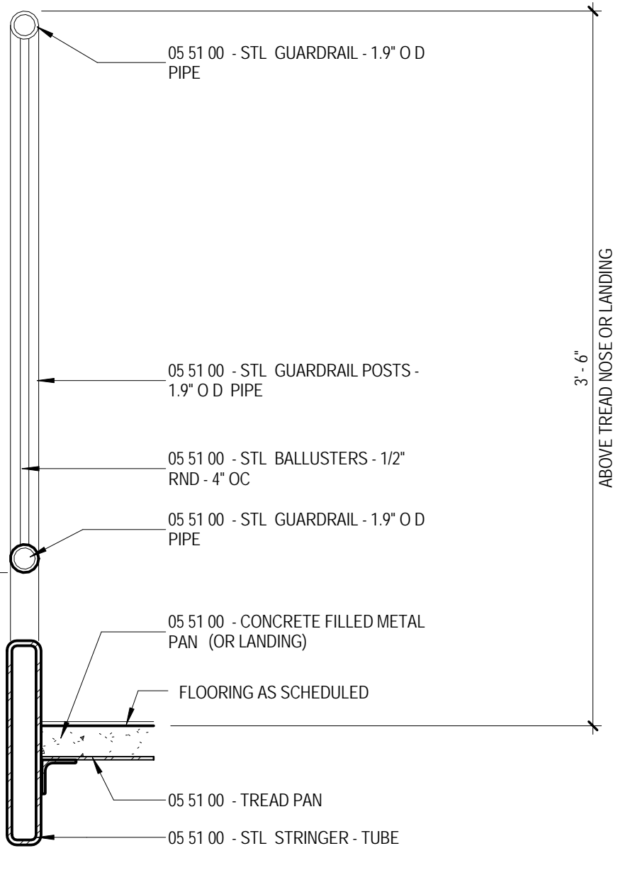
H4 STAIR DETAIL AT GUARDRAIL A4.9 1/12" = 1'-0"
