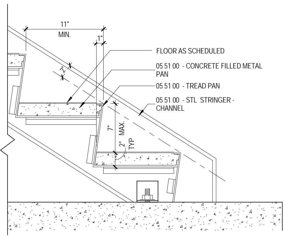
J1 TYP. STAIR DETAIL at BOTTOM of STAIR A4.9 1/12" = 1'-0"
