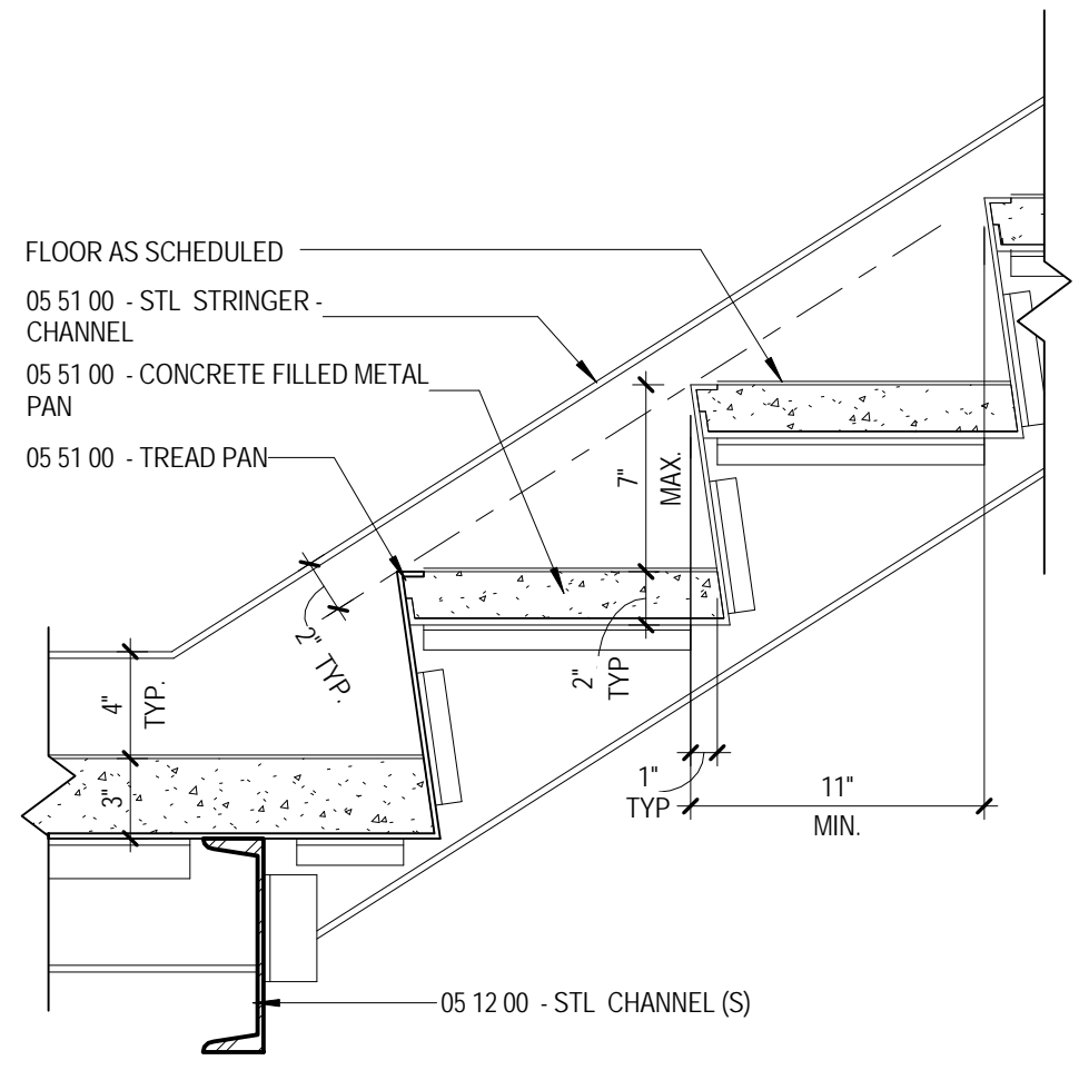
J4 TYP. STAIR DETAIL AT BOTTOM OF STAIR LANDING A4.9 1/12" = 1'-0"
