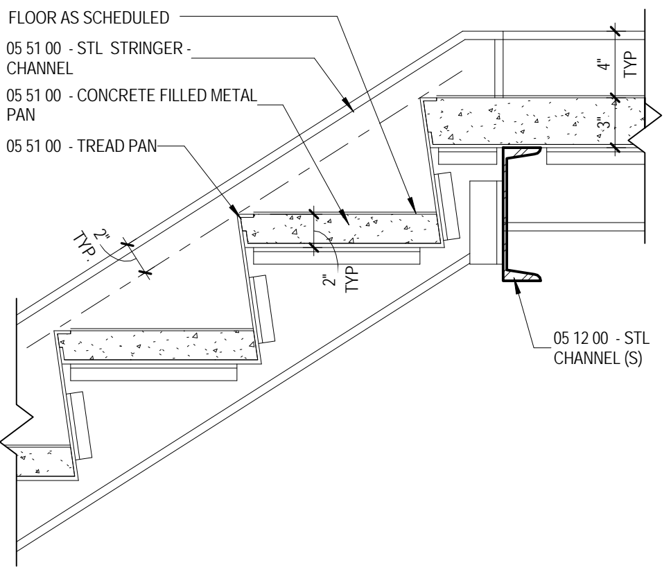
J7 TYP. STAIR DETAIL AT TOP OF STAIR LANDING A4.9 1/12" = 1'-0"
