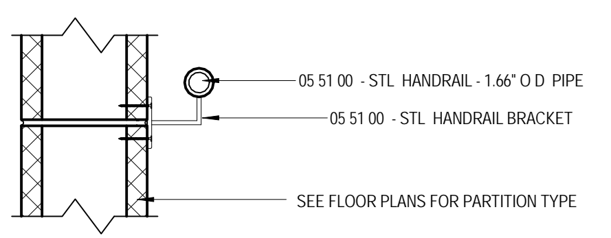
D4 STAIR SECTION DETAIL AT HANDRAIL A4.9 1/12" = 1'-0"
