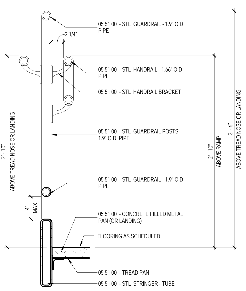
H10 STAIR DETAIL at GUARDRAIL AND HANDRAIL AT RAMPS A4.9 1/12" = 1'-0"
