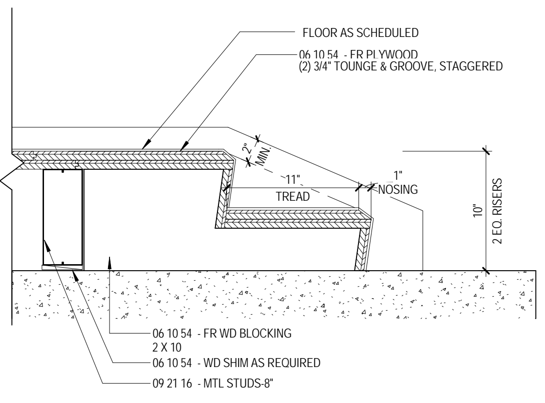
J10 TYP. STAIR DETAIL at BOTTOM of LIGHTWEIGHT FRAMING STAIR A4.9 1/12" = 1'-0"
