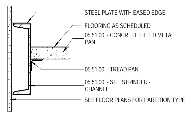
D7 STAIR SECTION DETAIL at PARTITION ALONG STRINGER A4.9 1/12" = 1'-0"
