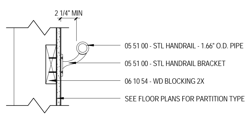
D1 SECTION DETAIL at HANDRAIL A4.9 1/12" = 1'-0"
