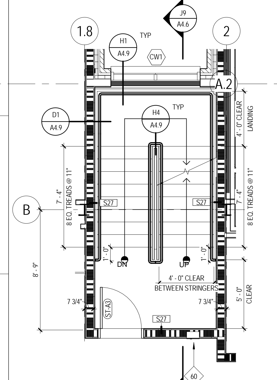
G1 LEVEL 3 STAIR A A4.6 1/4" = 1'-0"
