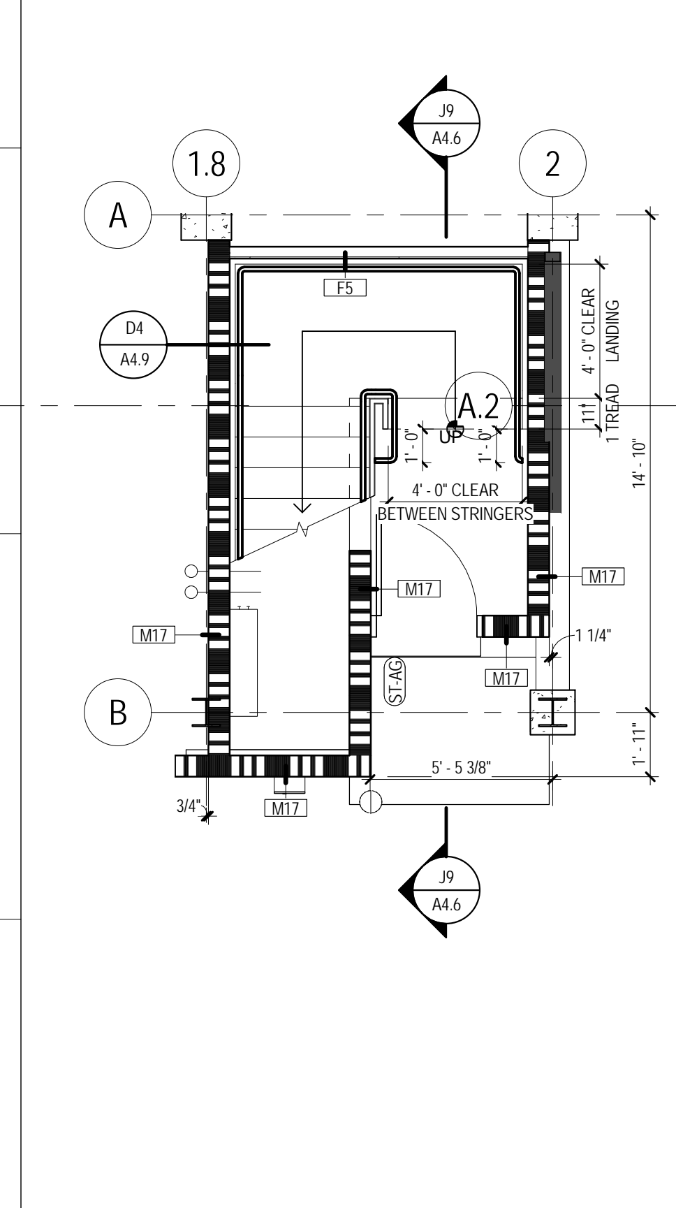
E1 BASEMENT LEVEL STAIR A A4.6 1/4" = 1'-0"
