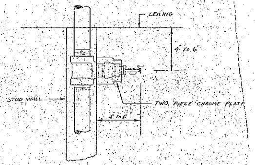
SIDEWALL SPRINKLER LOCATION 3" = 1'-0"
