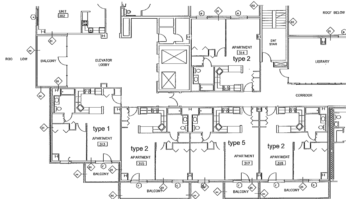
Third Floor Partial Plan
