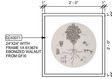
2 X0071 - ARTWORK DETAIL Scale: 1" = 1'-0"
