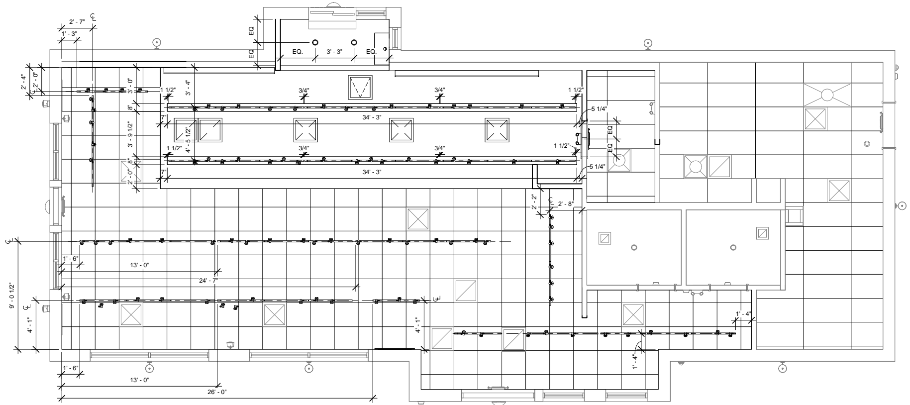
DIMENSIONED CEILING PLAN
