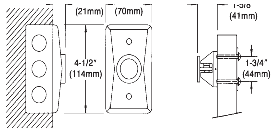
1505-AQN5 Flush Wall Mounted (Short Catch Plate)
