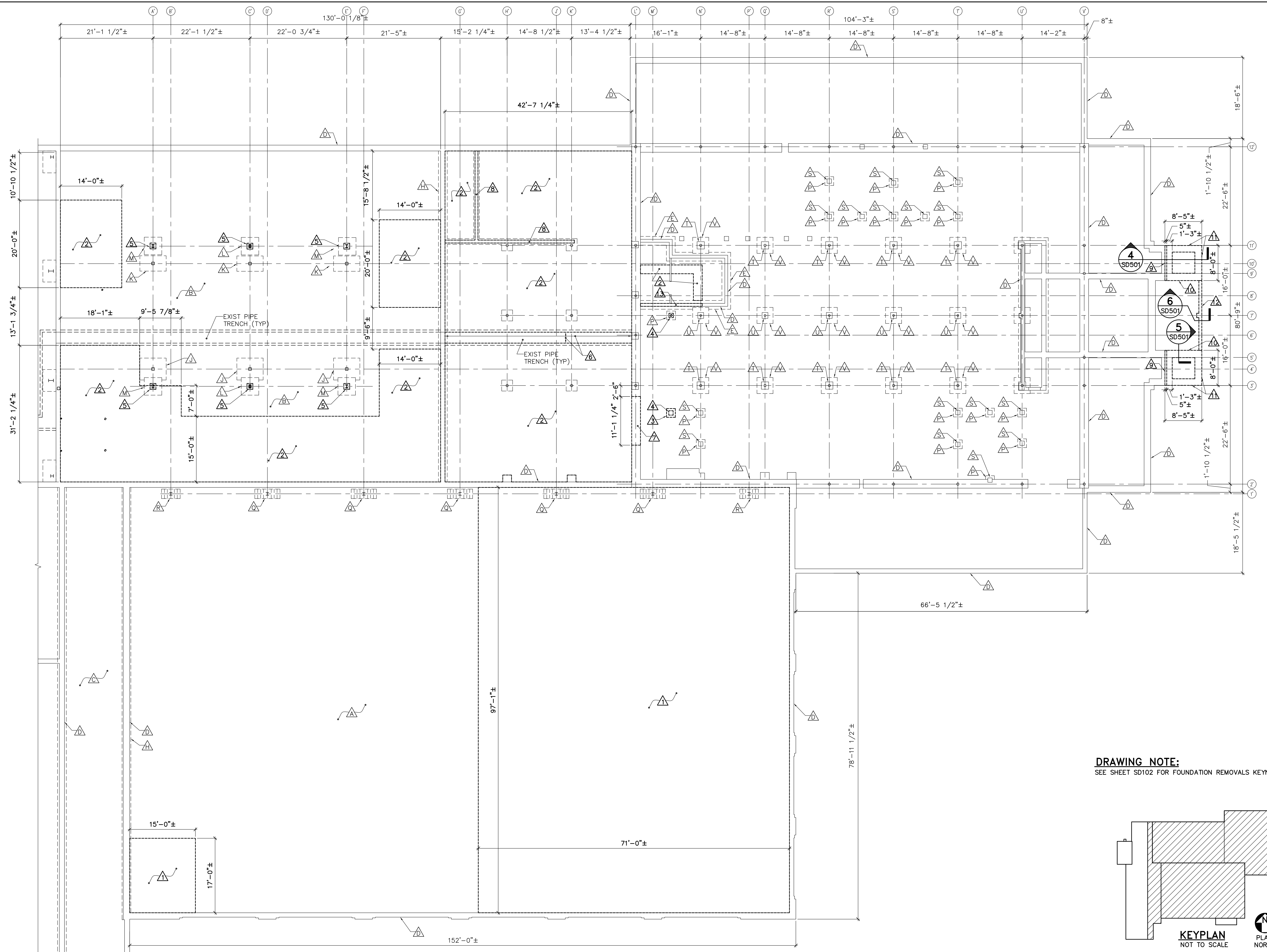
1 FOUNDATION REMOVALS PART PLAN SD101 SCALE: 1/8"=1'-0" PLAN NORTH
