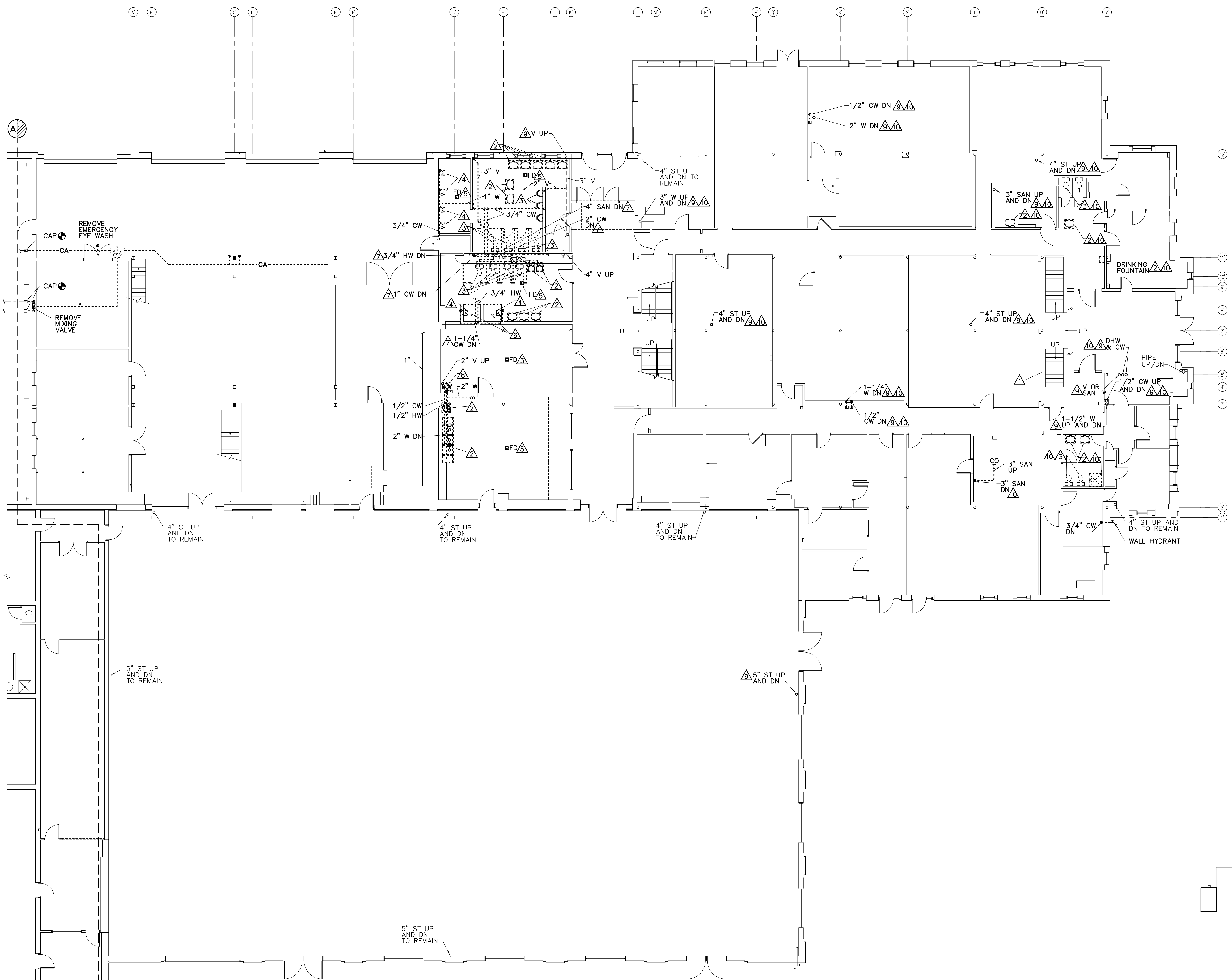
1 FIRST FLOOR PLUMBING REMOVALS PART PLAN PD102 SCALE: 1/8"=1'-0" PLAN NORTH
