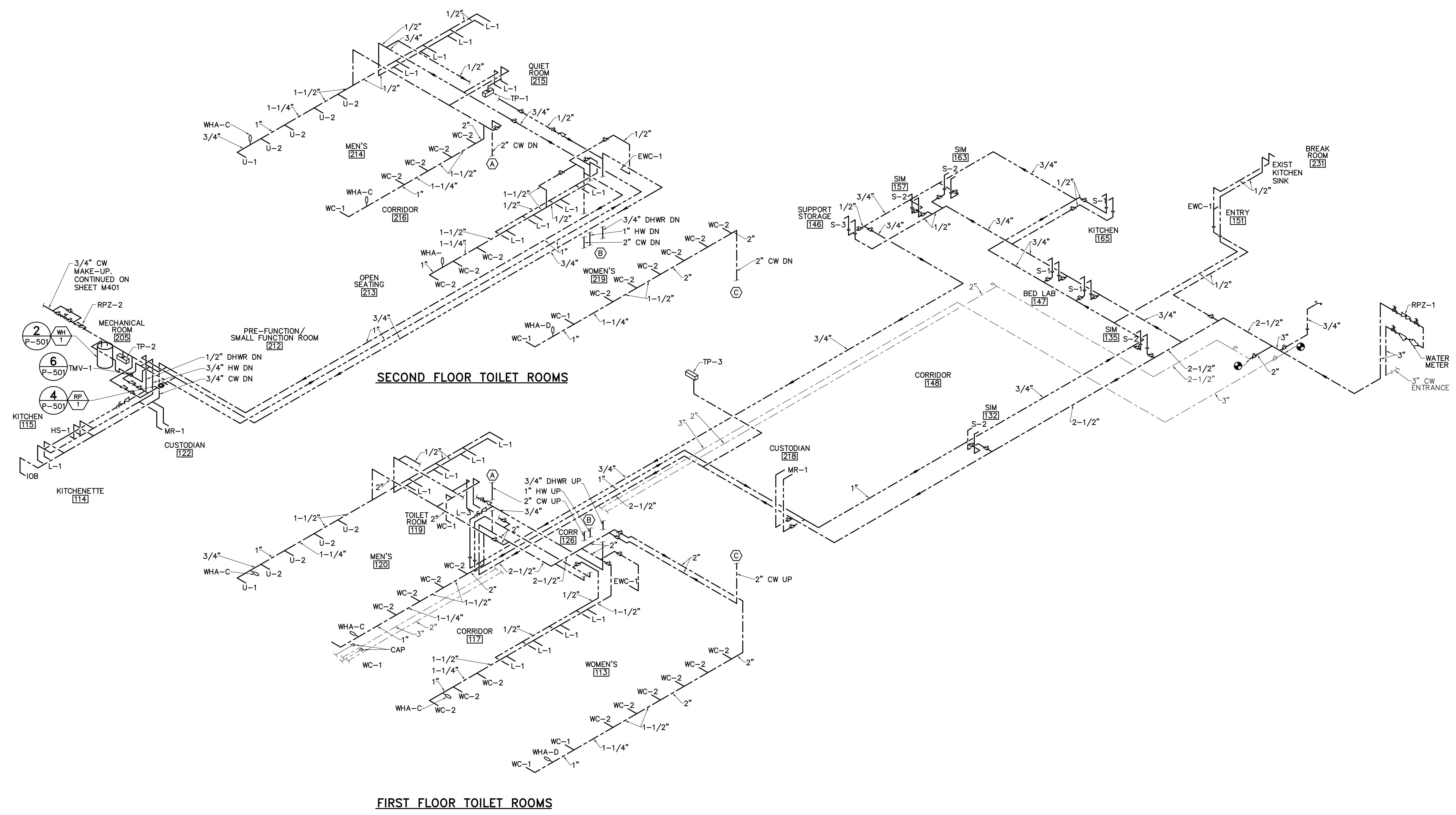
1 WATER SUPPLY RISER DIAGRAM P-702 NOT TO SCALE
