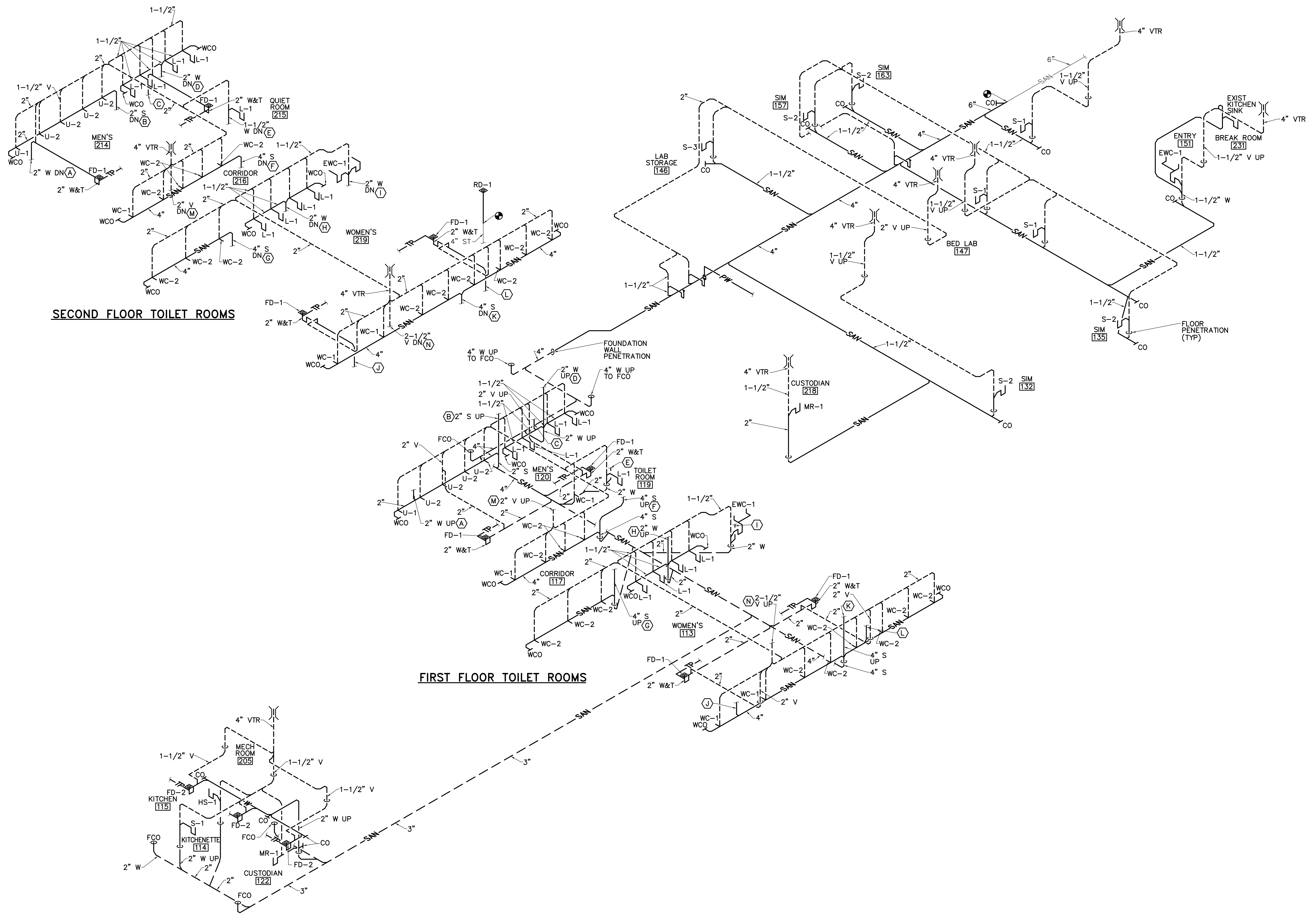
1 SANITARY RISER DIAGRAM P-701 NOT TO SCALE
