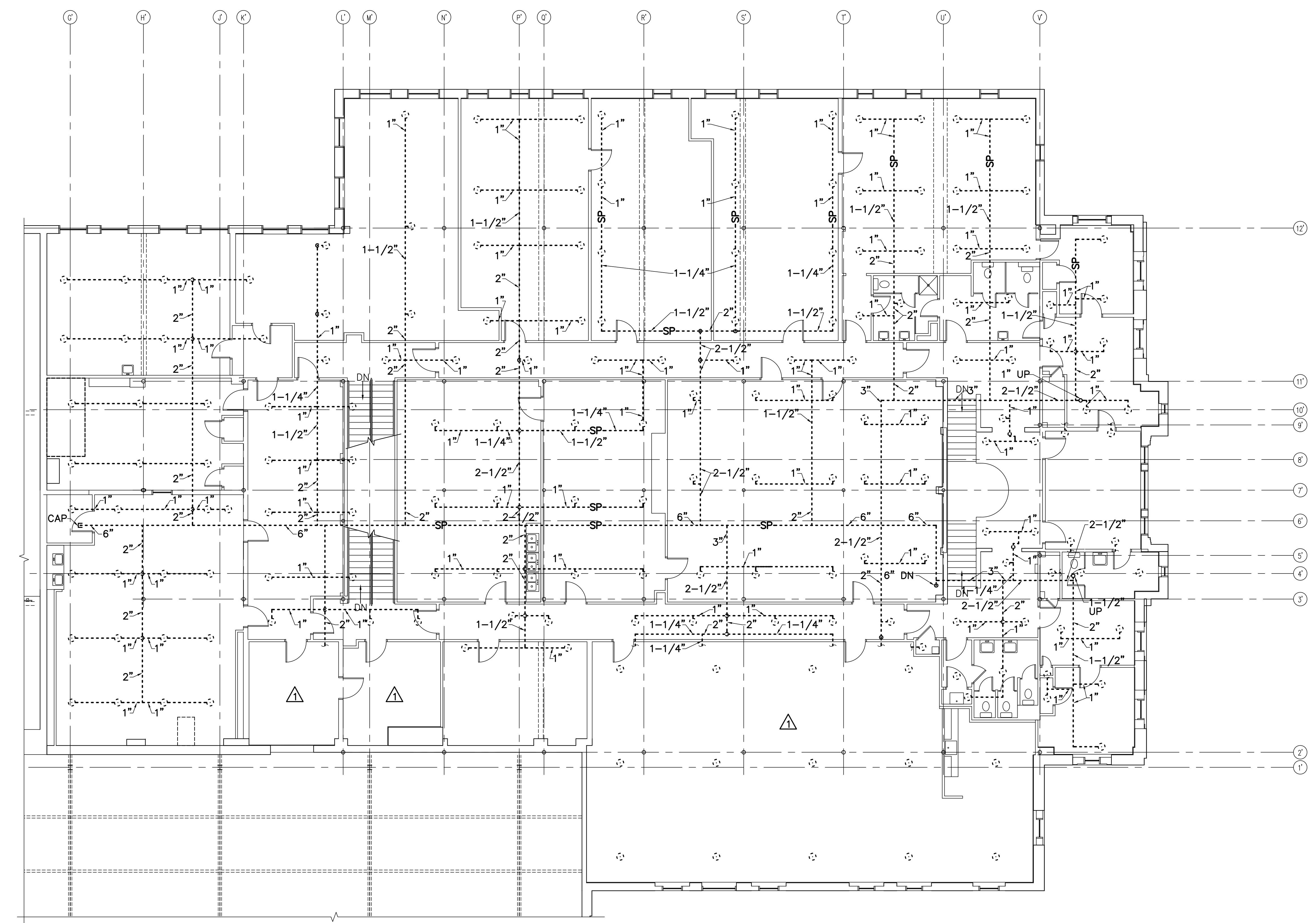
1 SECOND FLOOR FIRE SUPPRESSION REMOVALS PART PLAN FD103 SCALE: 1/8"=1'-0" PLAN NORTH
