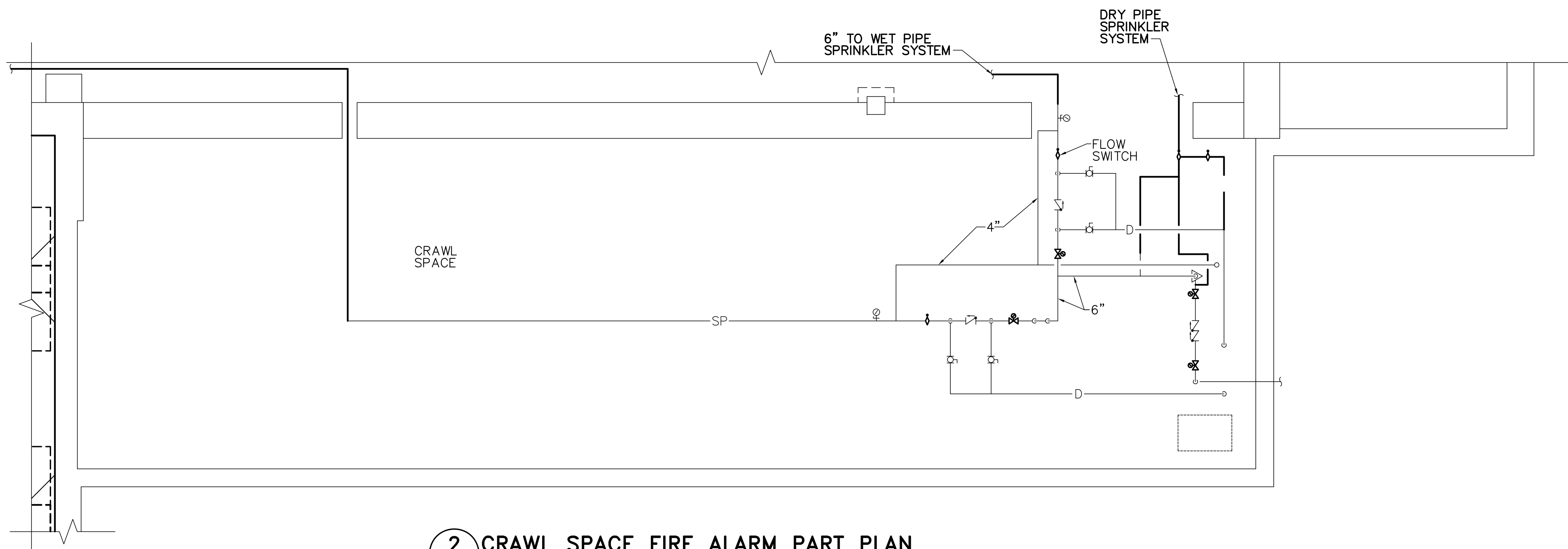
2 CRAWL SPACE FIRE ALARM PART PLAN FA102 SCALE: 1/8"=1'-0"
