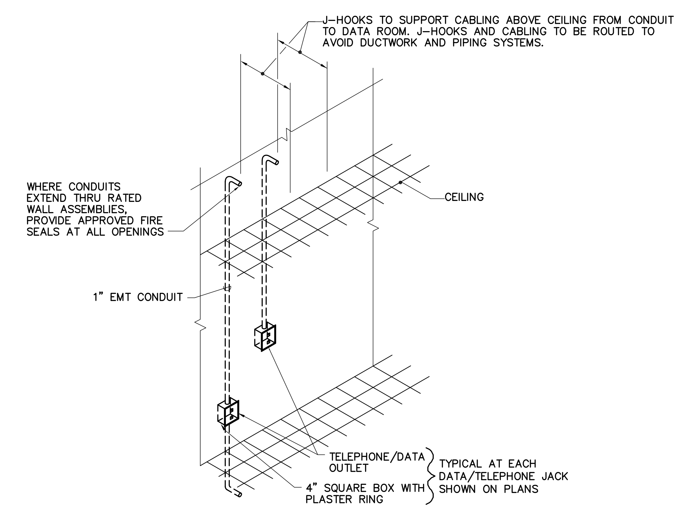
4 TYPICAL DETAIL OF BOXES AND TRAY ET501 NOT TO SCALE
