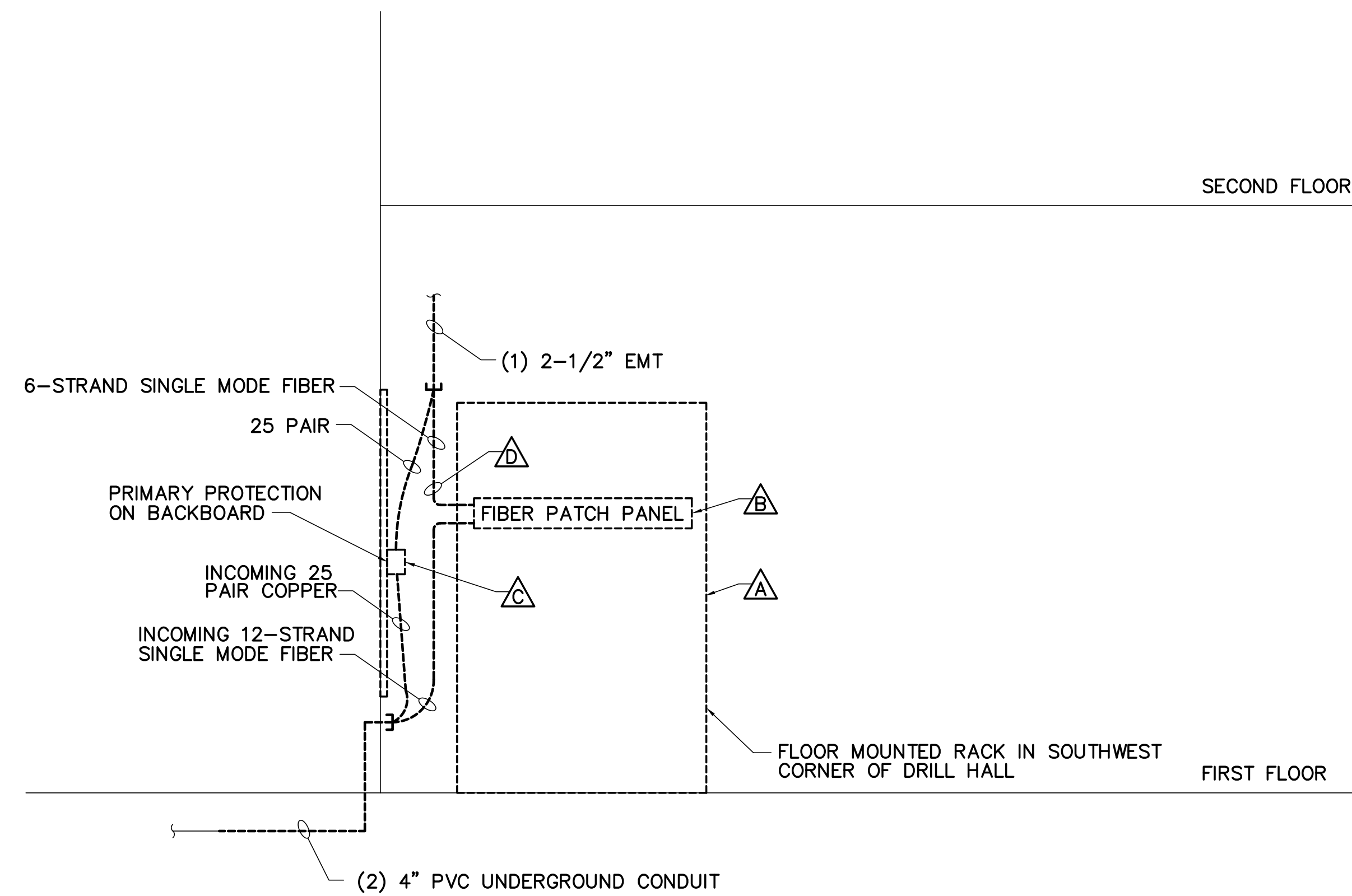
1 EXISTING COMMUNICATIONS ONE-LINE DIAGRAM ET501 NOT TO SCALE
