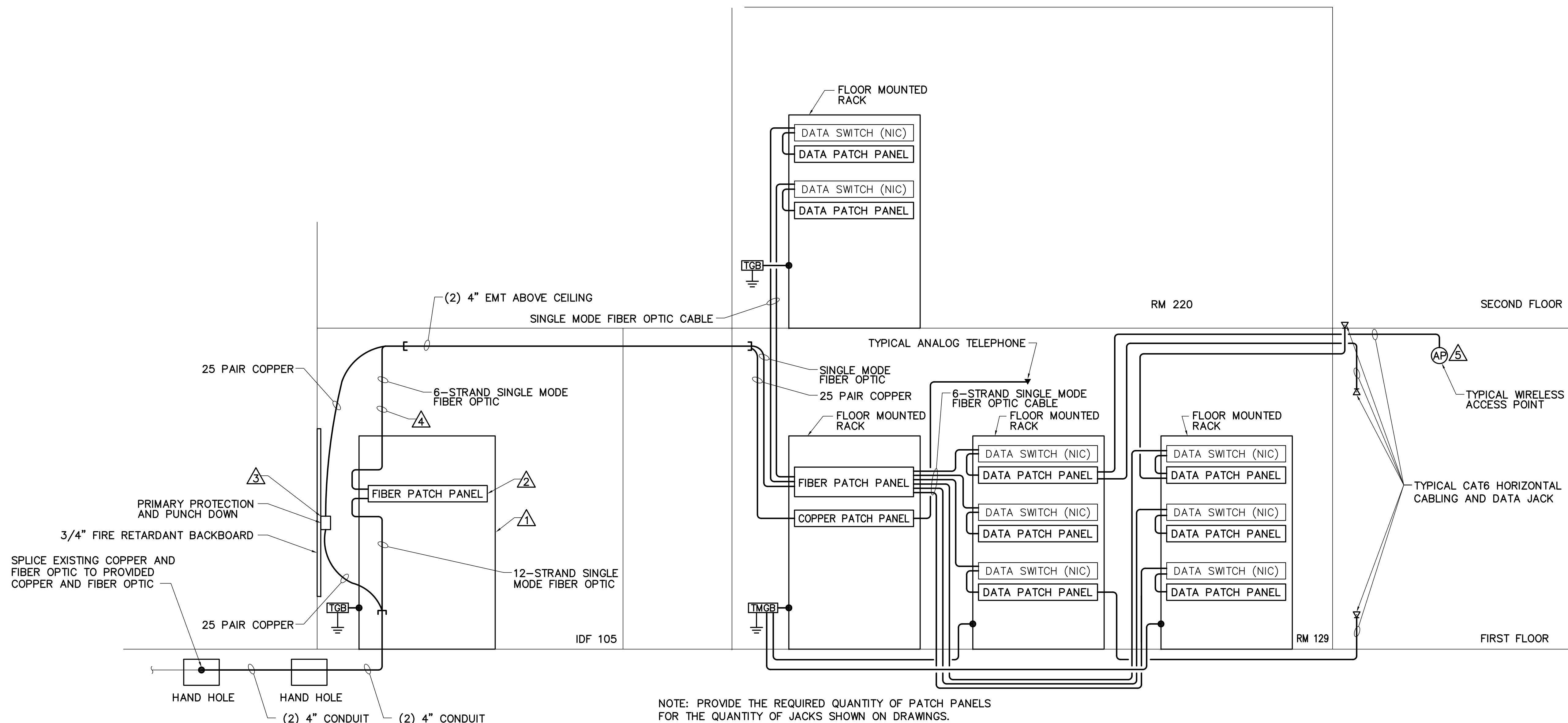
2 COMMUNICATIONS ONE-LINE DIAGRAM ET501 NOT TO SCALE
