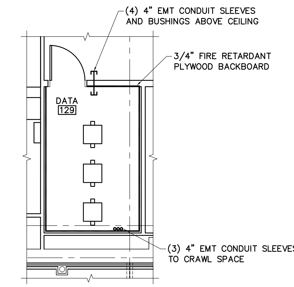
3 DATA ROOM 129 DETAIL ET501 1/4"=1'-0"
