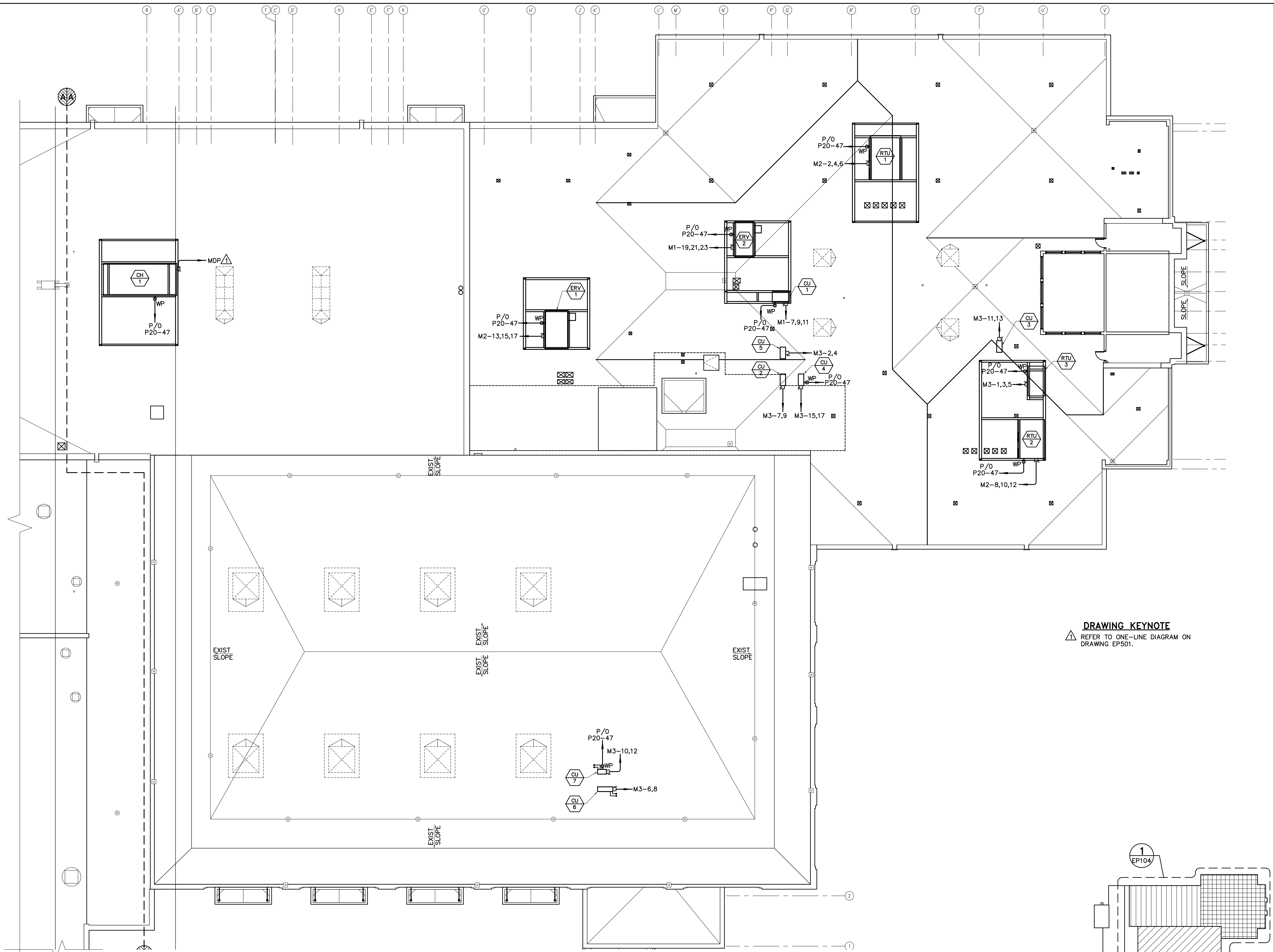
1 ROOF ELECTRICAL PLAN EP104 SCALE: 1/8"=1'-0"
