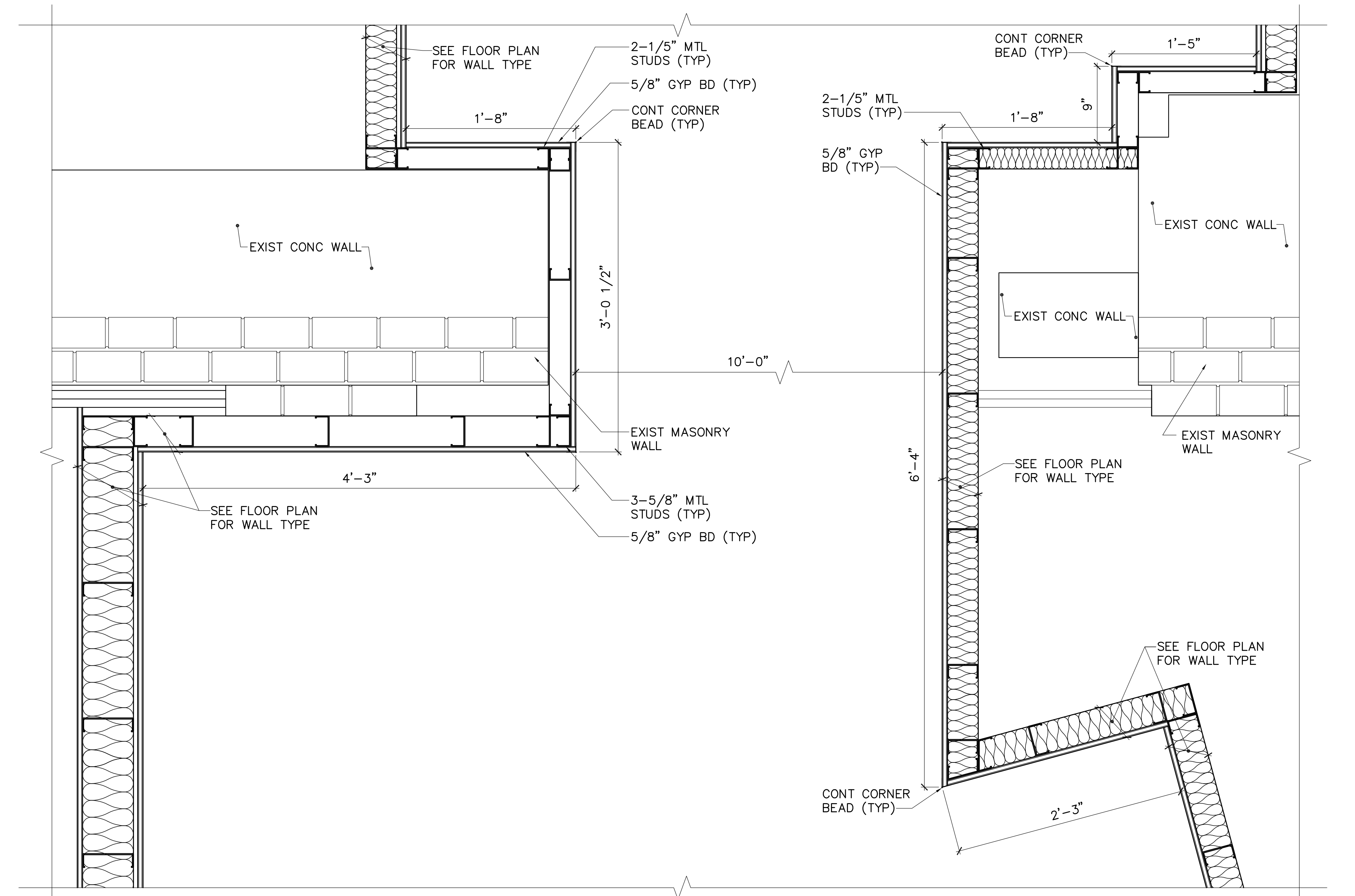
17 WALL DETAIL AE101 AE540 SCALE: 1-1/2"=1'-0"
