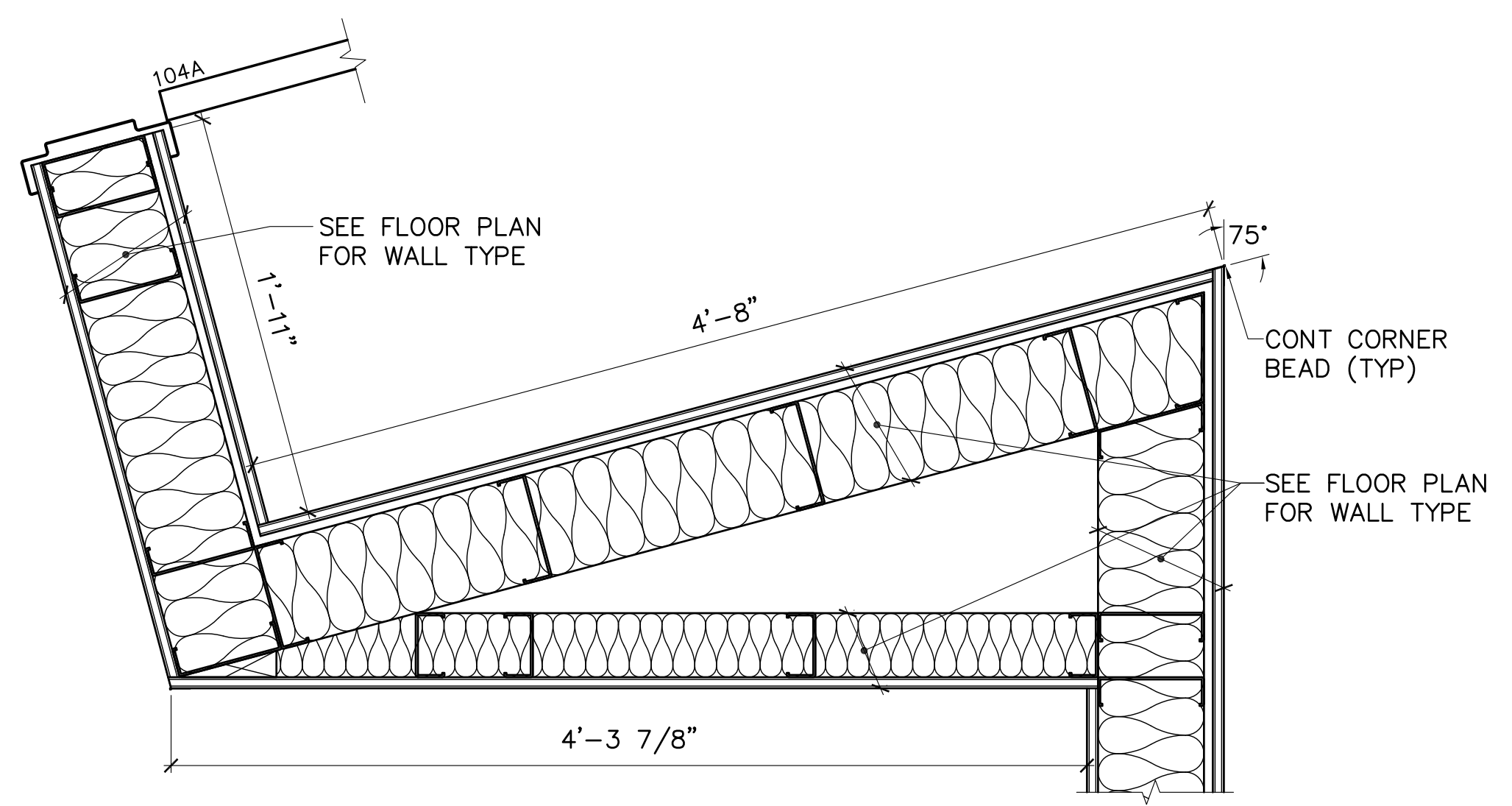
14 WALL DETAIL AE101 AE540 SCALE: 1-1/2"=1'-0"
