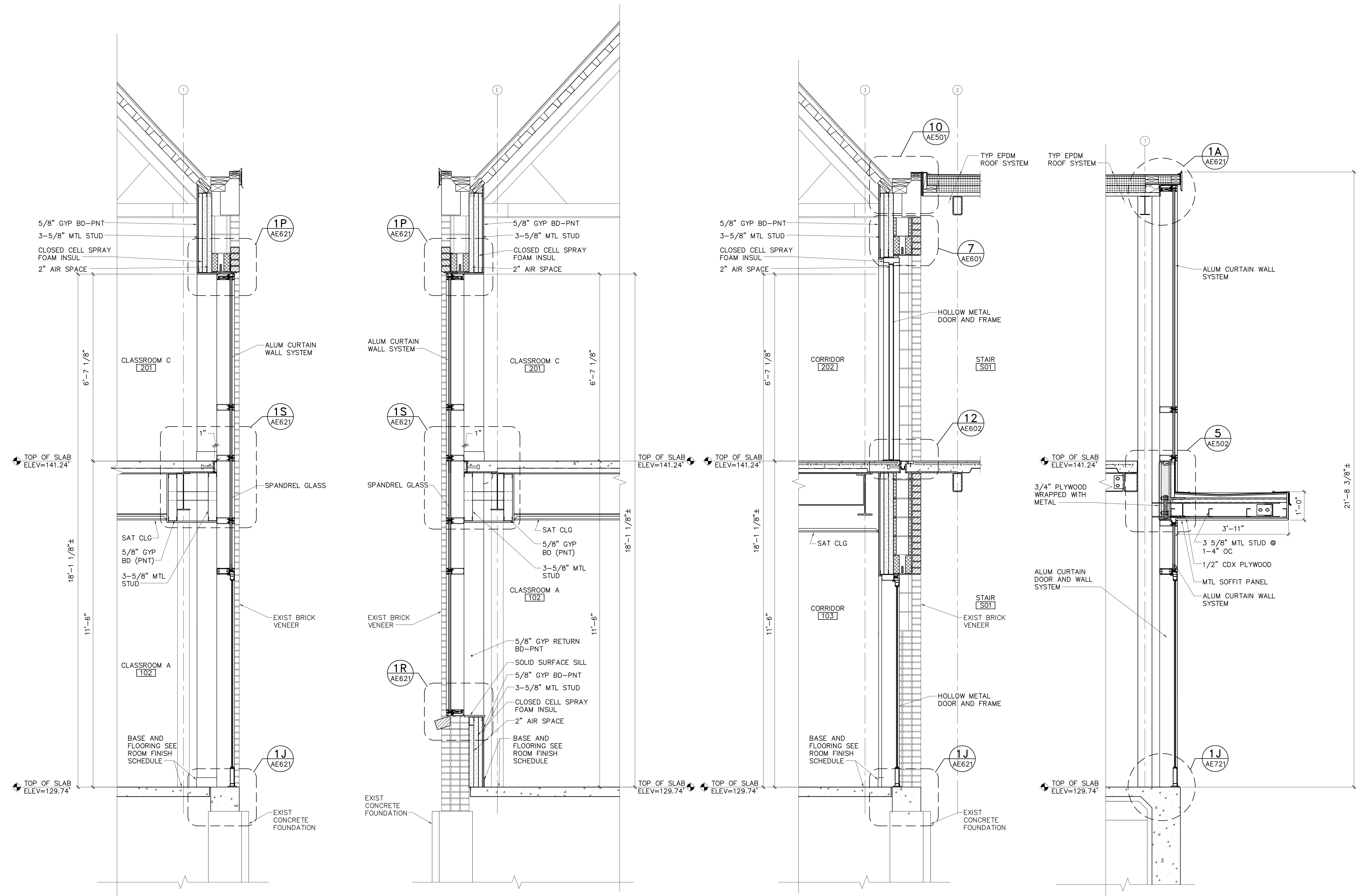
1 EXTERIOR WALL SECTION @ CLASSROOMS AE220, AE201 AE301 SCALE: 3/4"=1'-0"
