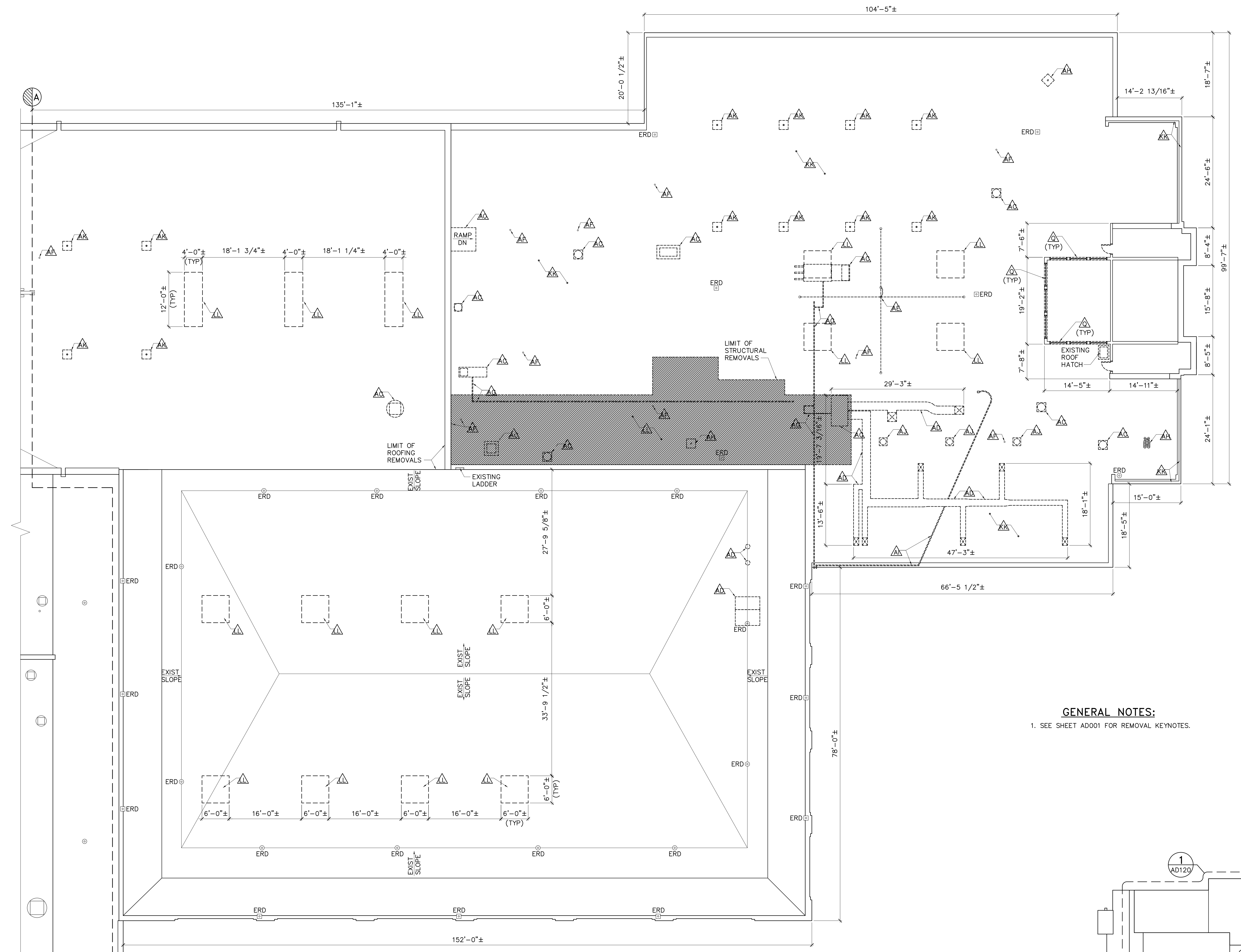
1 ROOF REMOVALS PART PLAN AD120 SCALE: 1/8"=1'-0"
