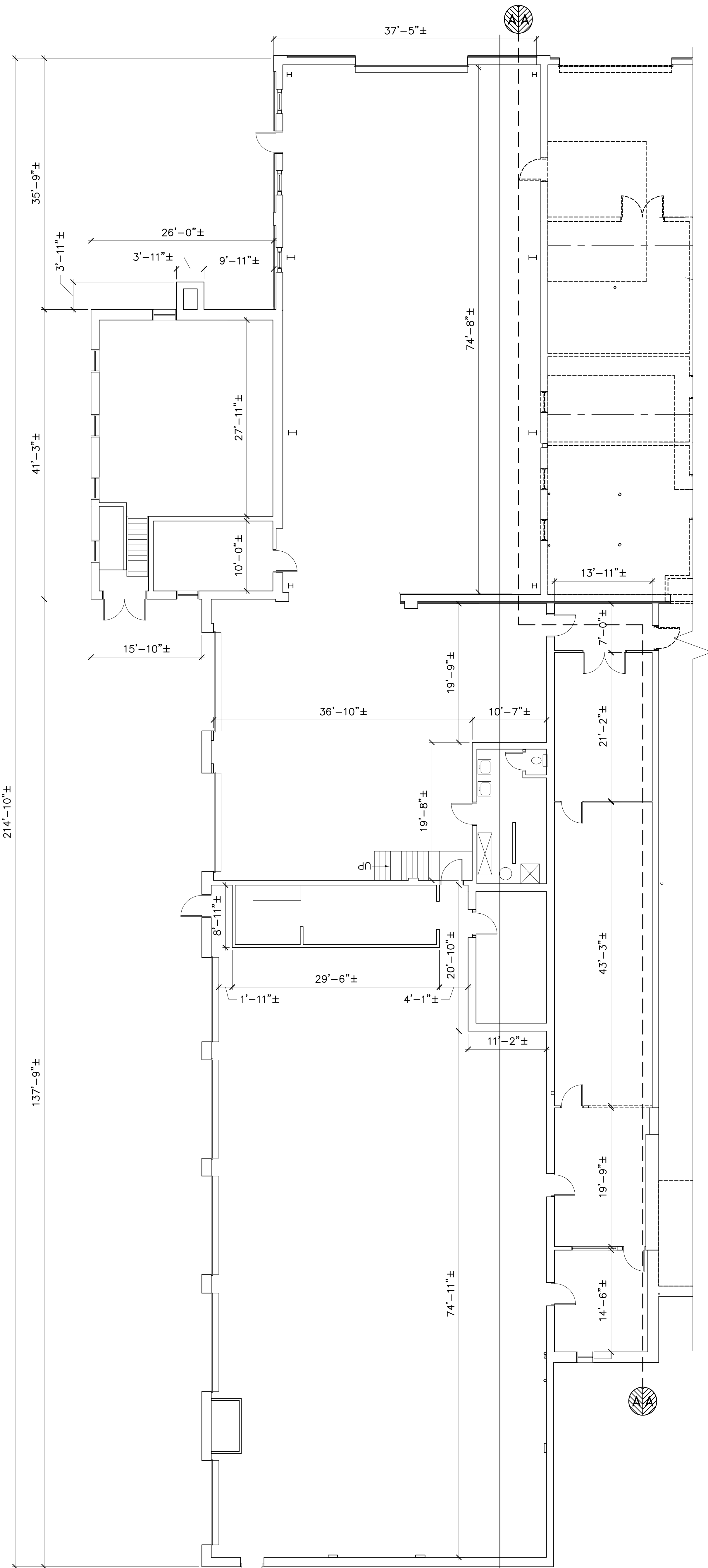
2 FIRST FLOOR REMOVALS PART PLAN
