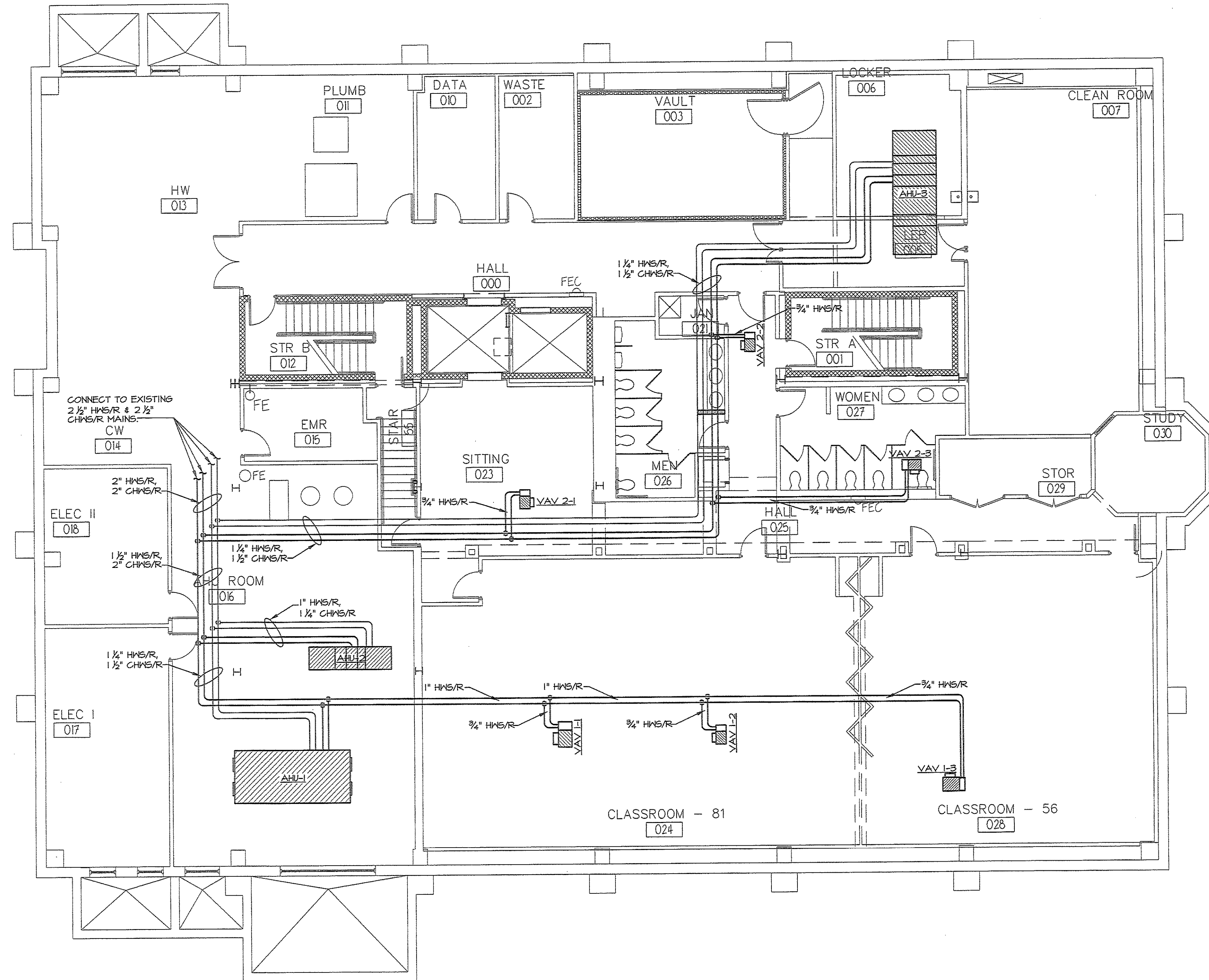
LOWER LEVEL HVAC PIPING PLAN SCALE: 1/8" = 1'-0"
