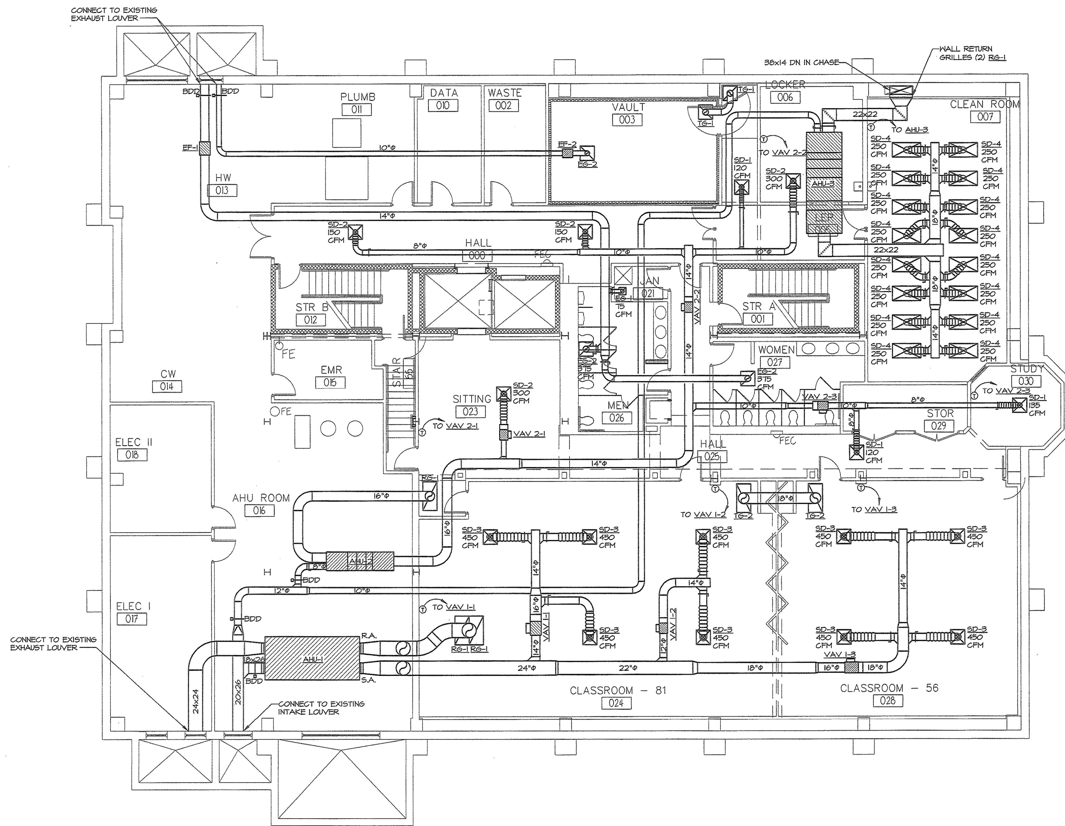
LOWER LEVEL HVAC PLAN SCALE: 1/8" = 1'-0"
