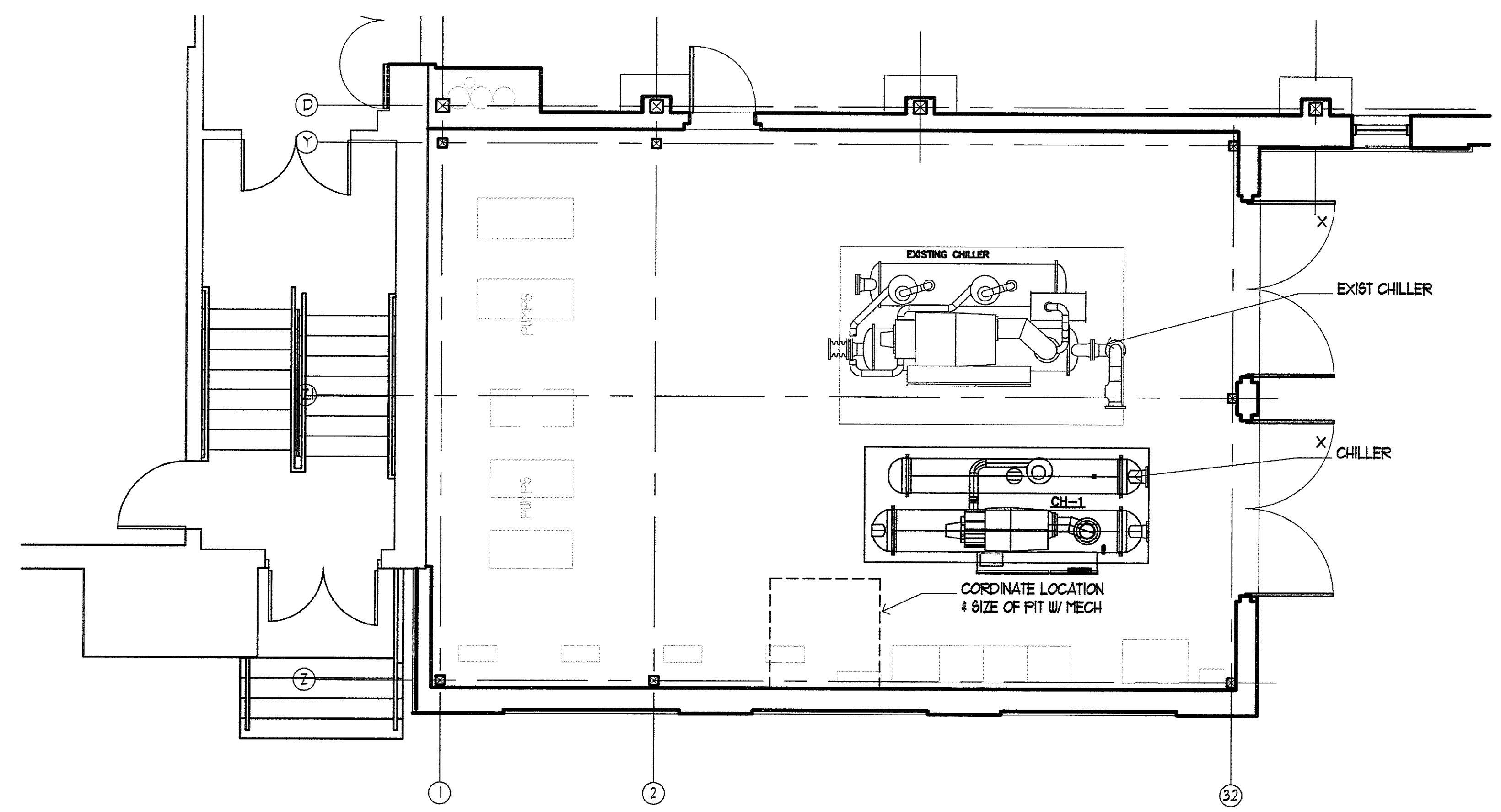
1 EXIST CHILLER ROOM PLAN SCALE: 1/4" = 1'-0"
