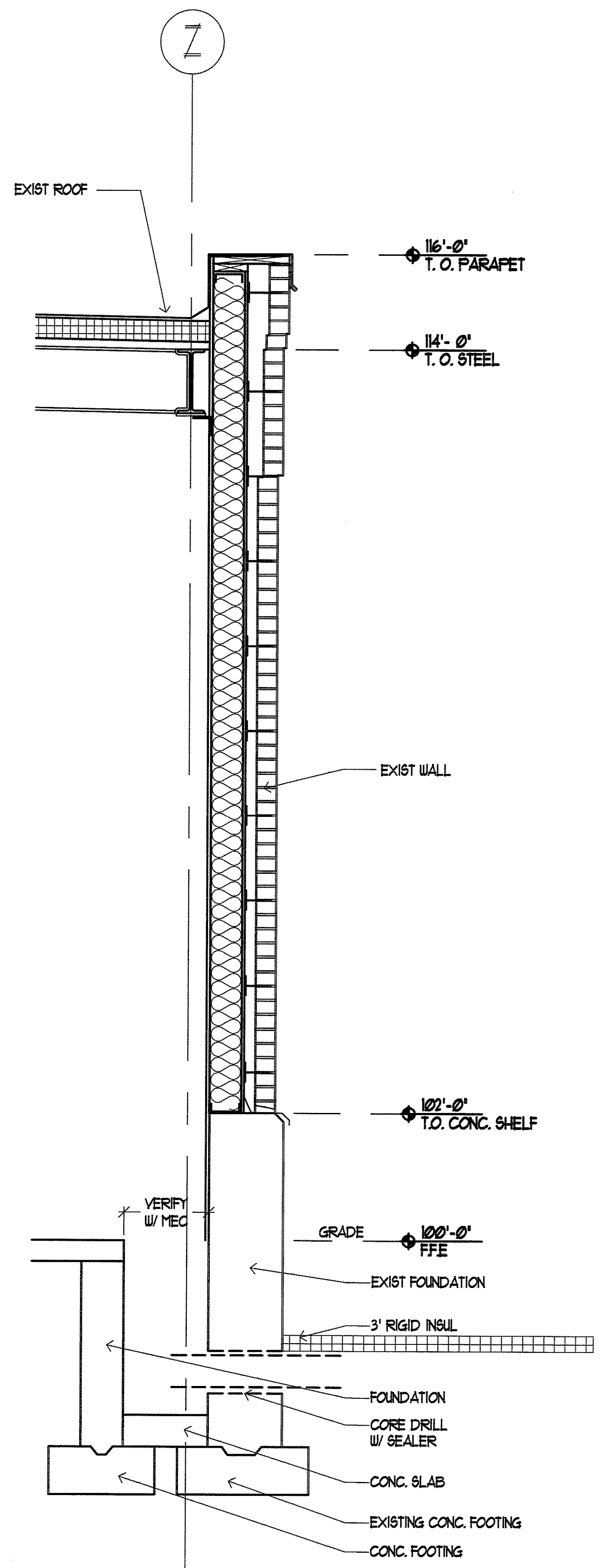
3 EXIST CHILLER ROOM WALL SECTION SCALE: 1/4" = 1'-0"
