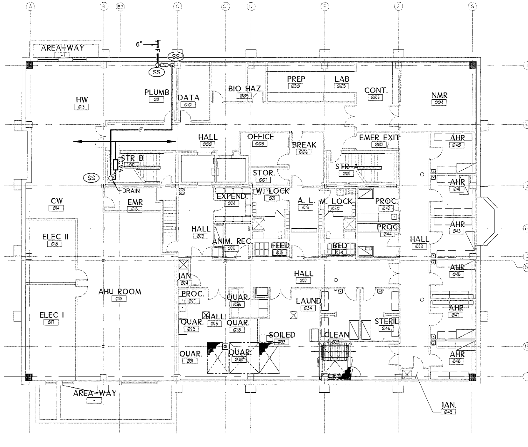
1 FIRE PROTECTION LOWER LEVEL PLAN - ALTERNATE Scale: 1/16"=1'-0"
