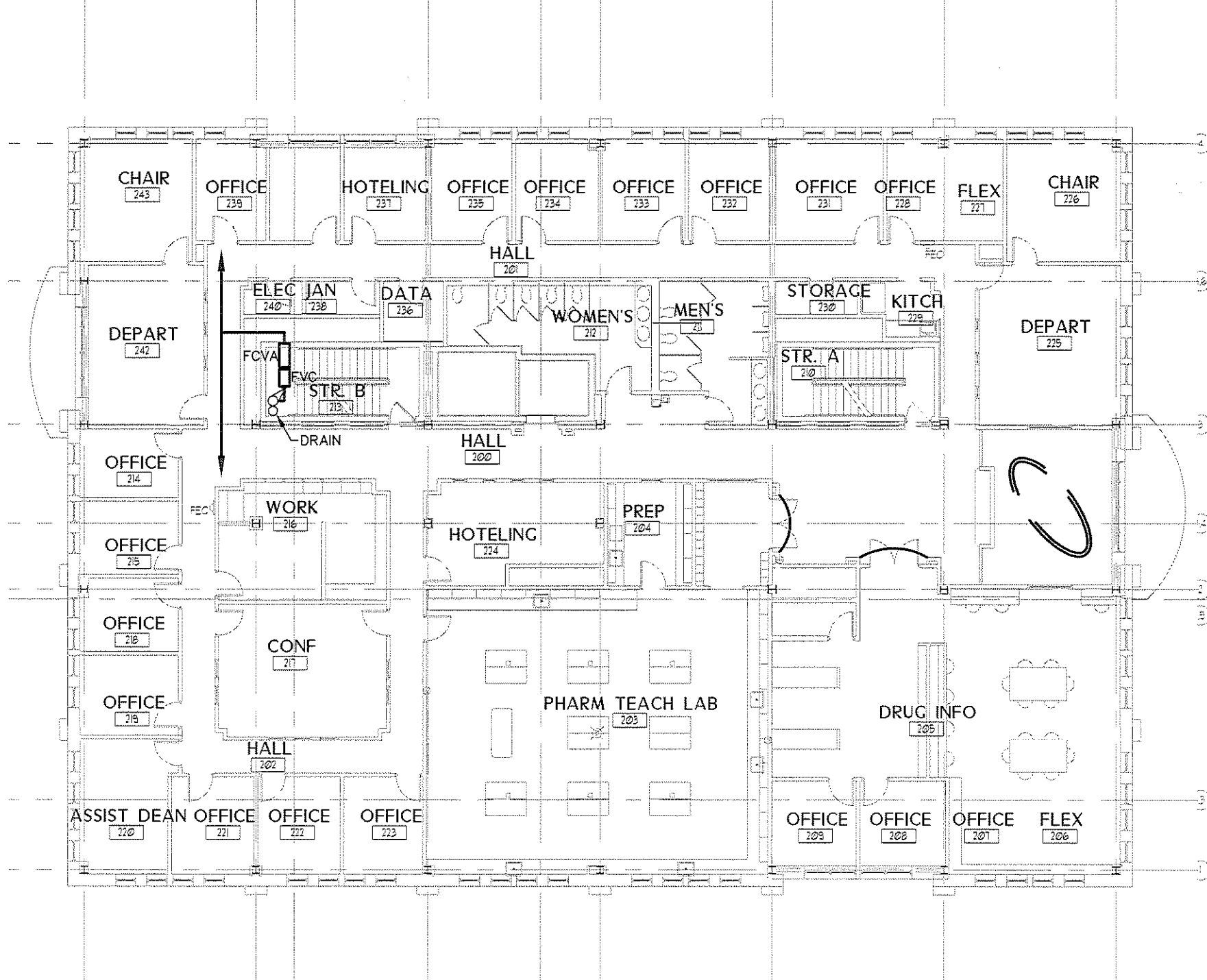
4 FIRE PROTECTION SECOND FLOOR PLAN Scale: 1/16"=1'-0"
