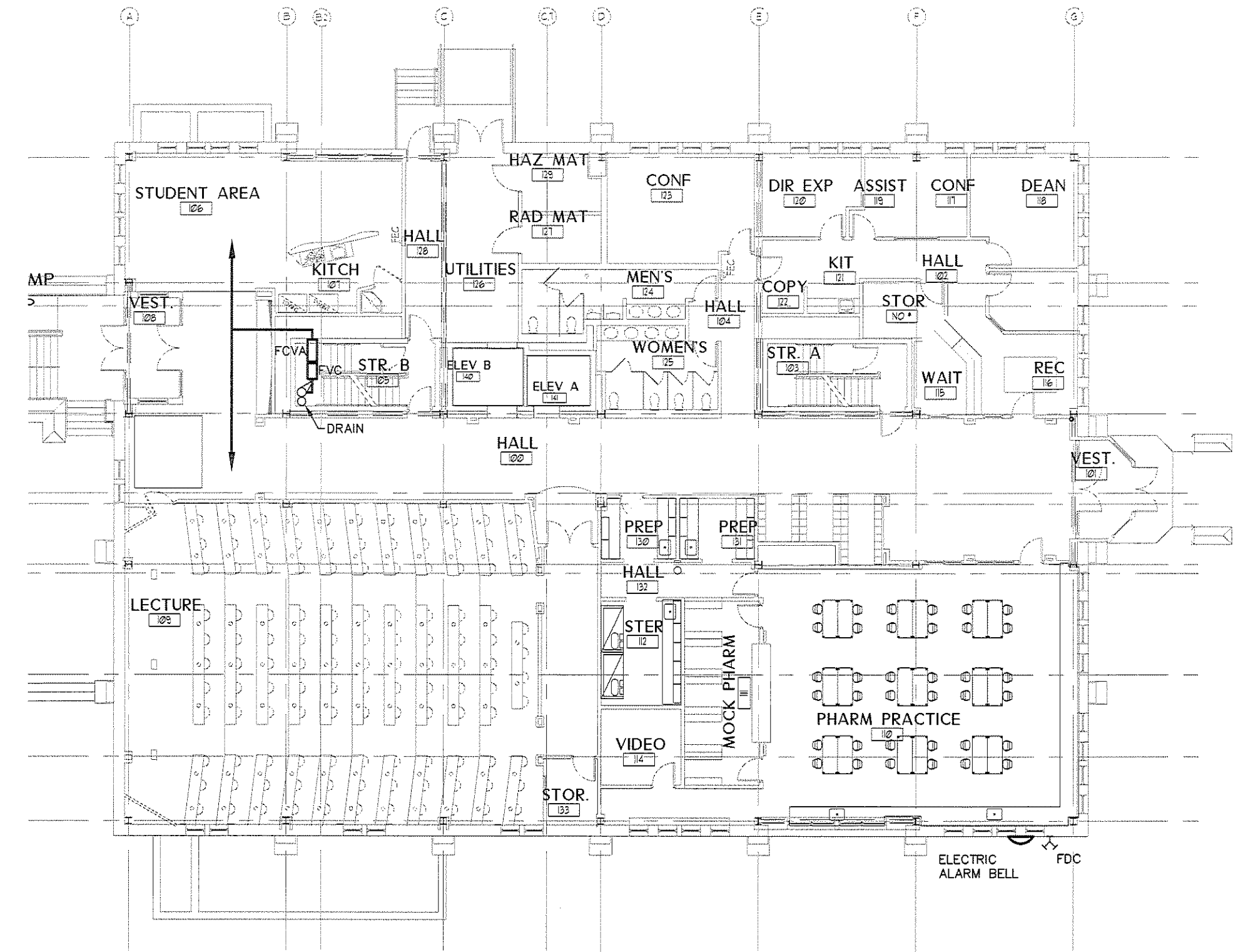
3 FIRE PROTECTION FIRST FLOOR PLAN Scale: 1/16"=1'-0"
