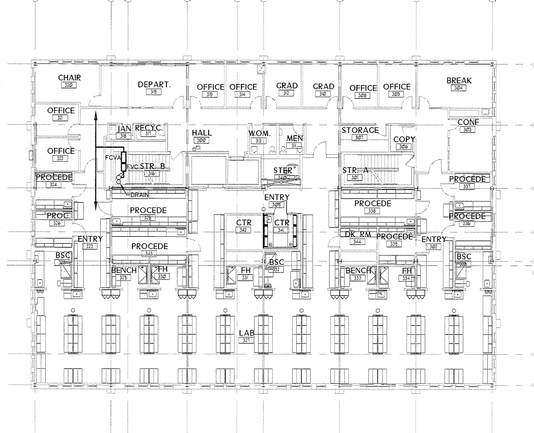
5 FIRE PROTECTION THIRD FLOOR PLAN Scale: 1/16"=1'-0"
