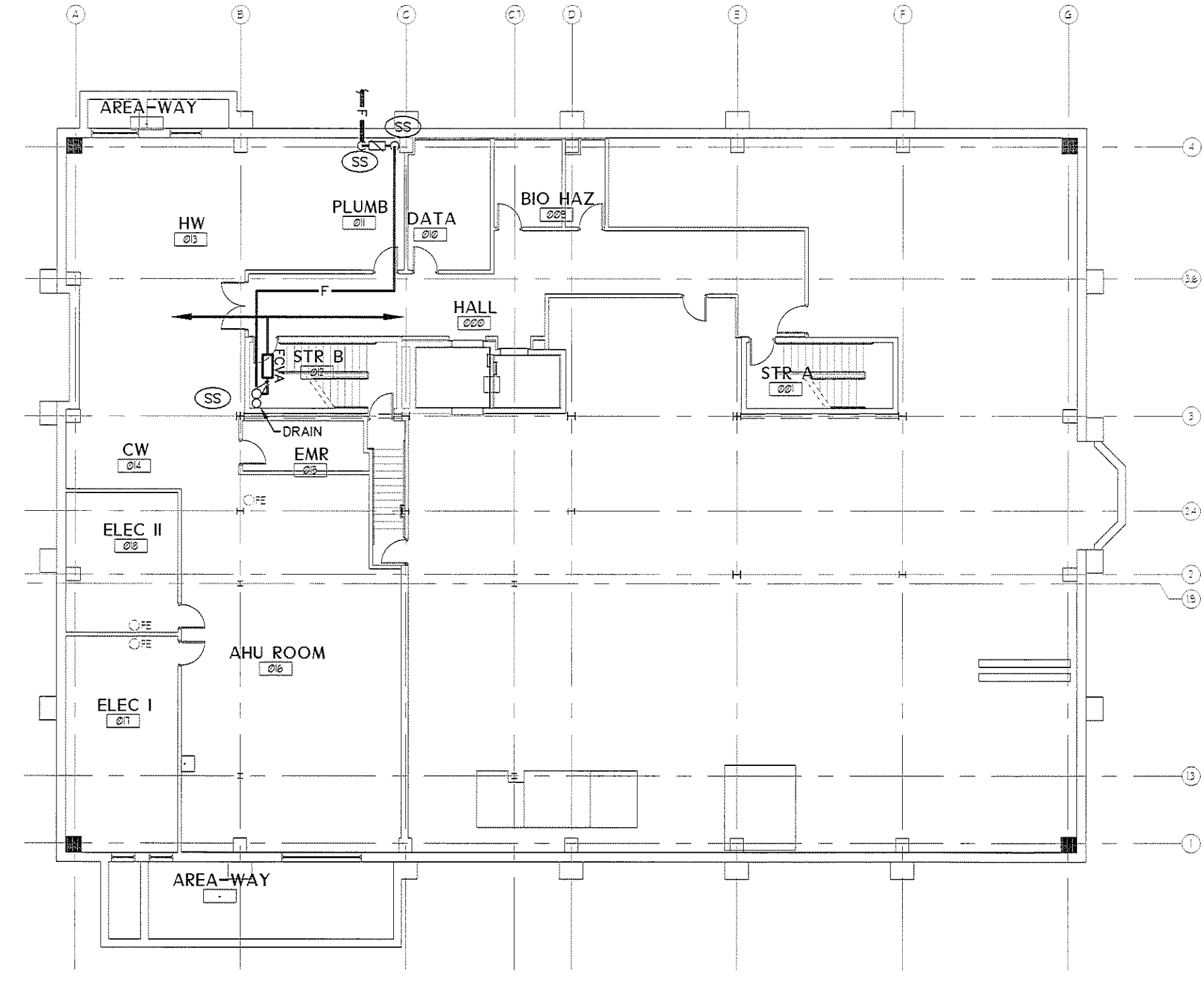
2 FIRE PROTECTION LOWER LEVEL PLAN Scale: 1/16"=1'-0"
