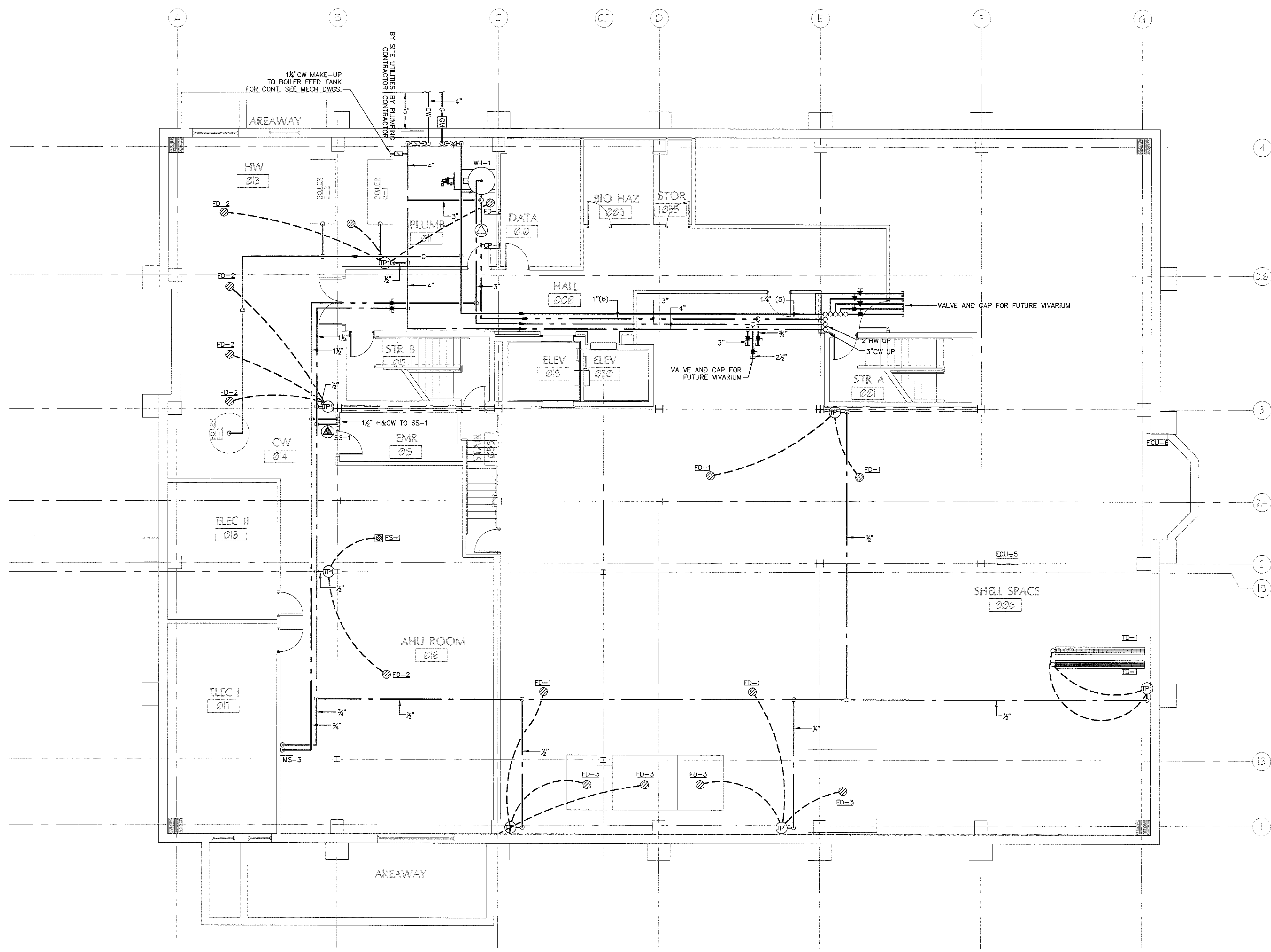
1 PLUMBING LOWER LEVEL PLAN - SUPPLY Scale: 1/8"=1'-0"
