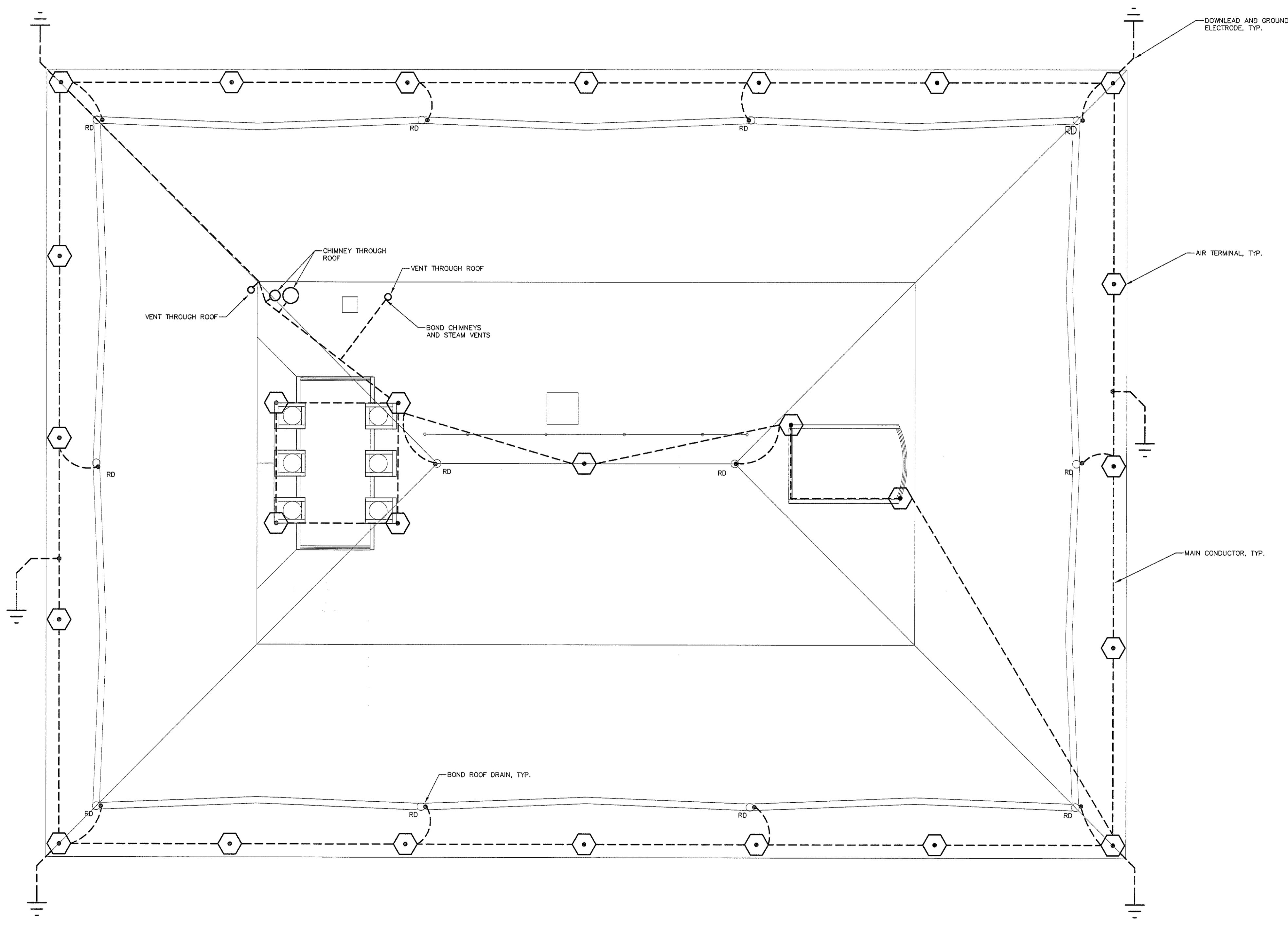
1 LIGHTNING PROTECTION PLAN Scale: 1/8"=1'-0"
