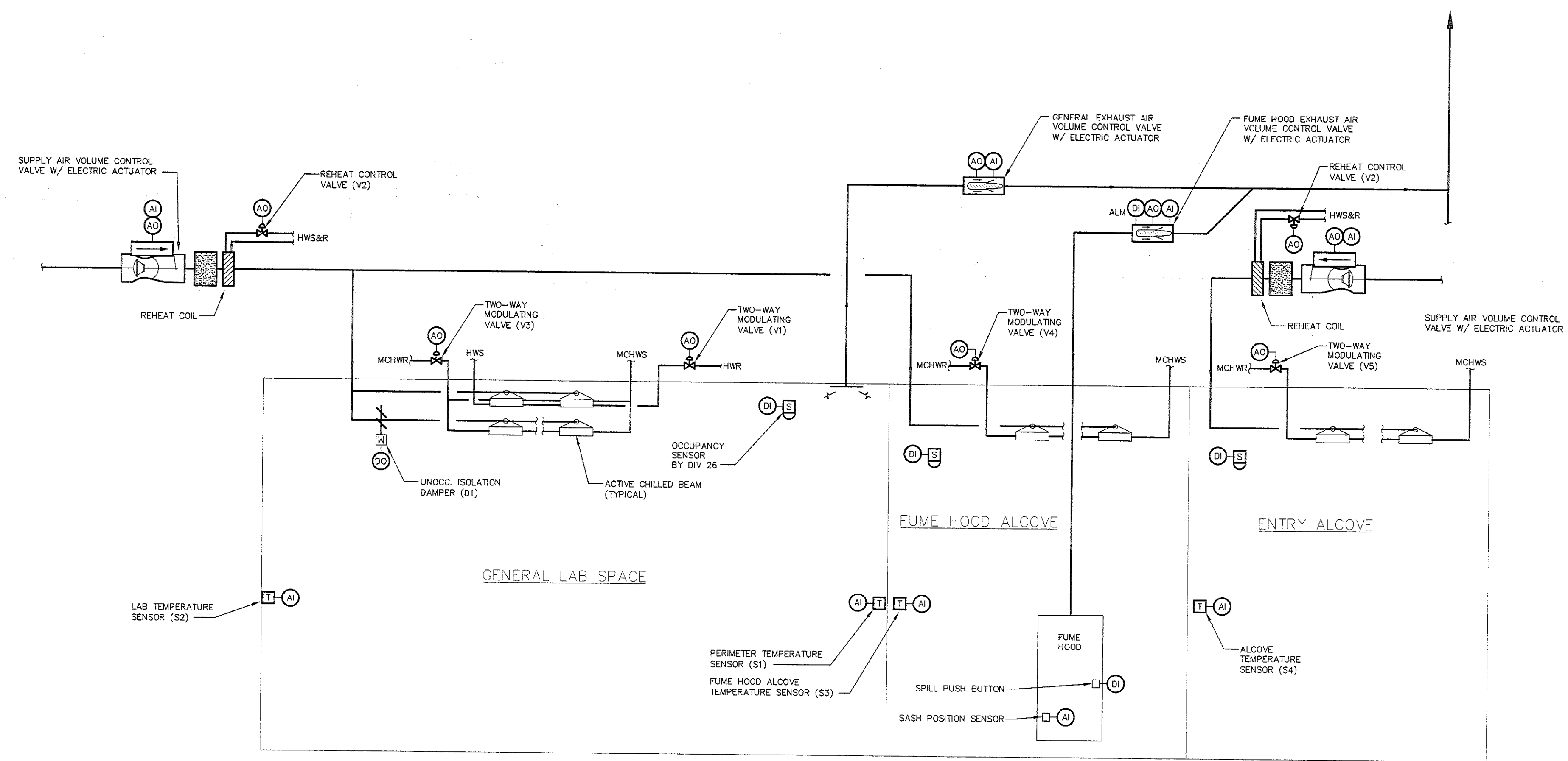
TYPICAL LABORATORY CONTROL DIAGRAM NOT TO SCALE
