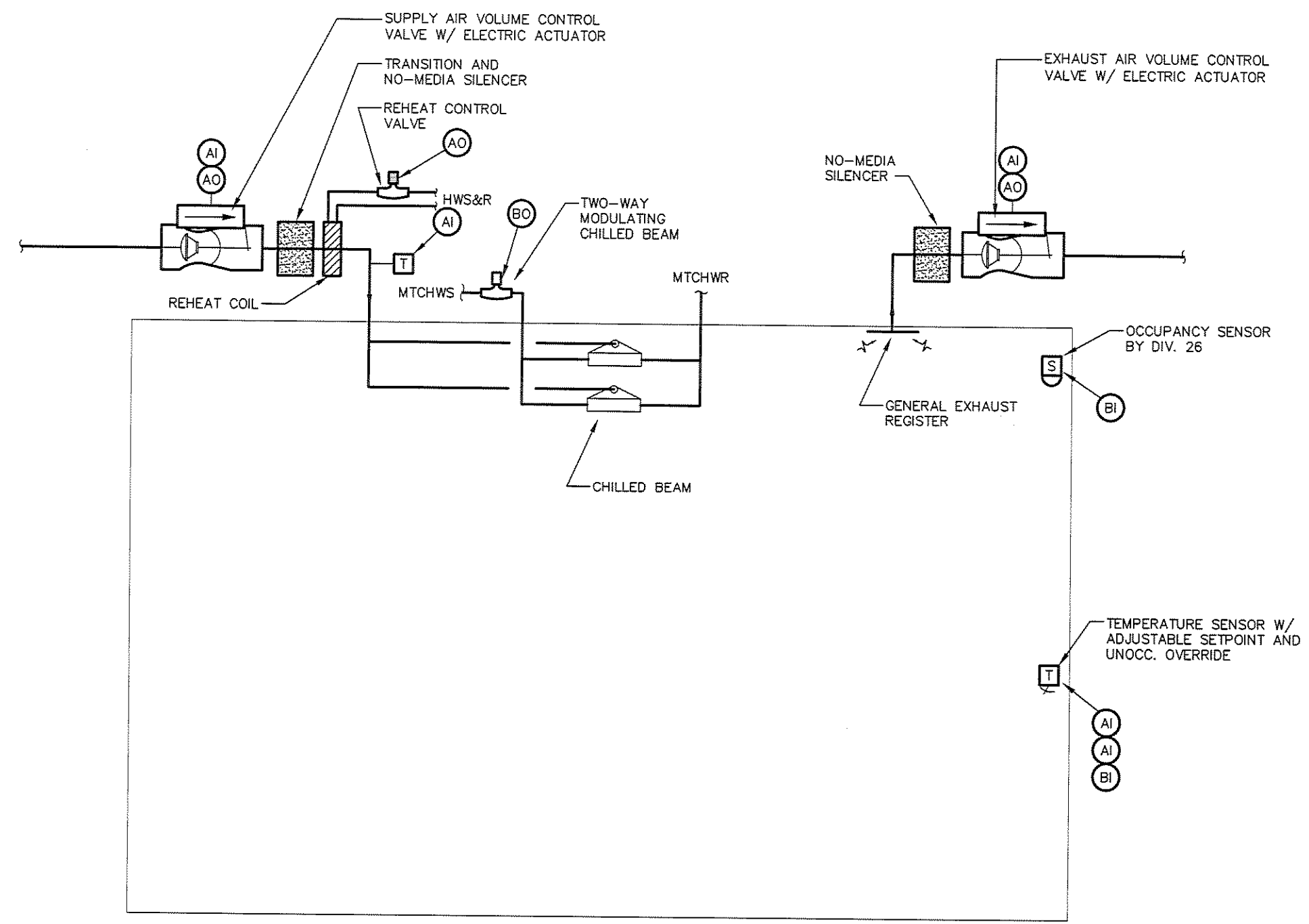
TYPICAL LABORATORY SUPPORT CONTROL DIAGRAM NOT TO SCALE
