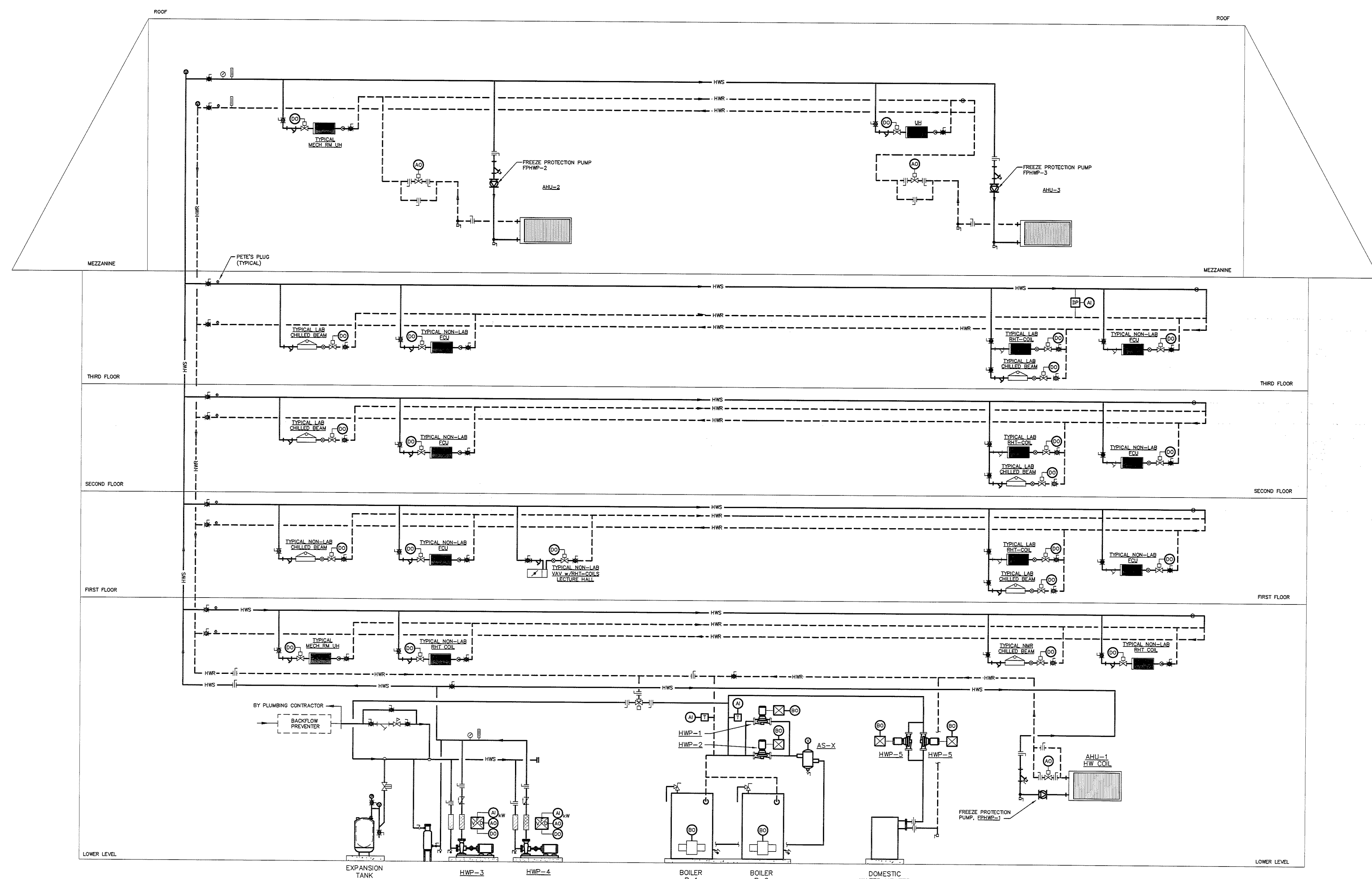
HOT WATER RISER DIAGRAM NOT TO SCALE
