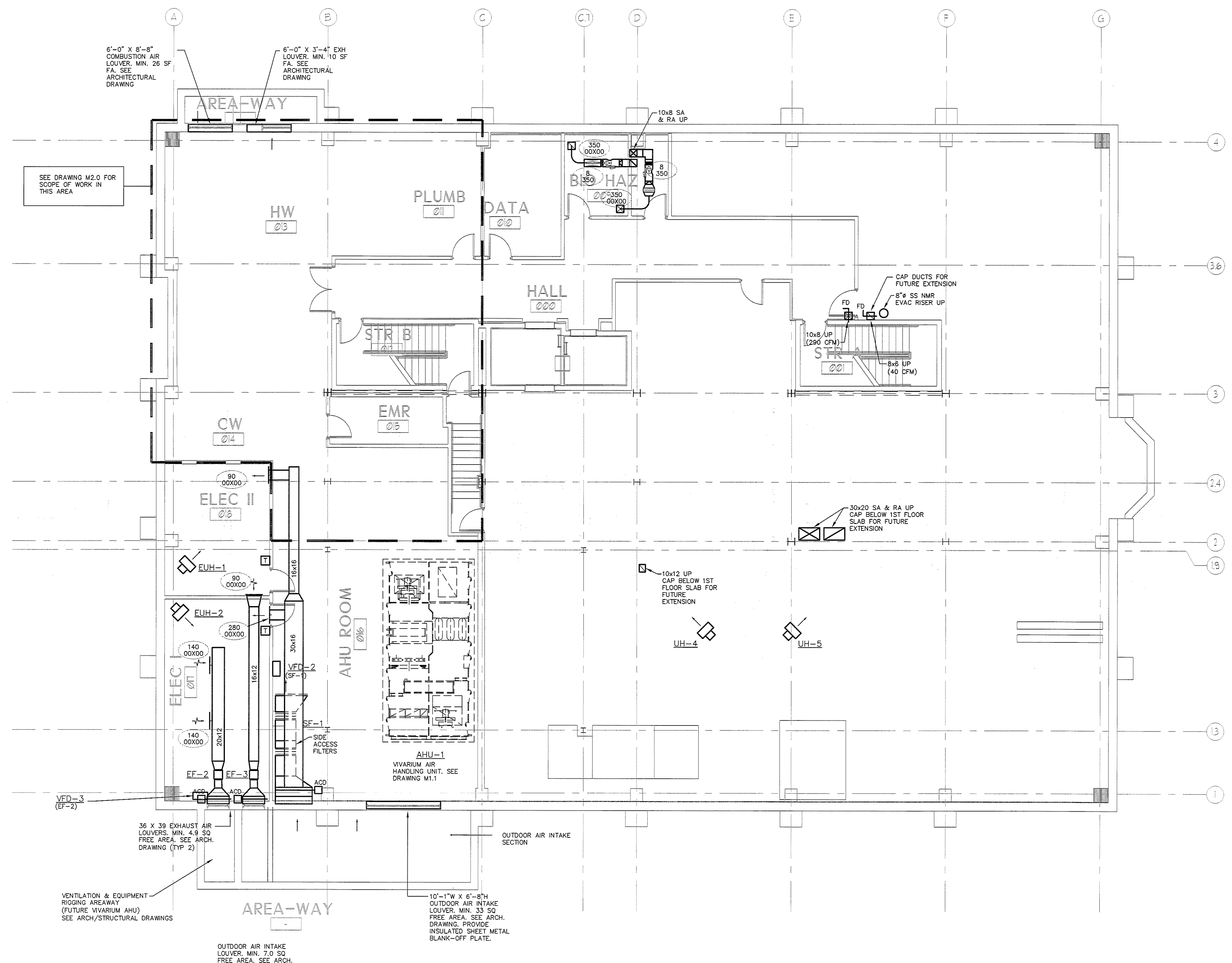
1 MECHANICAL LOWER LEVEL FLOOR PLAN Scale: 1/8"=1'-0"
