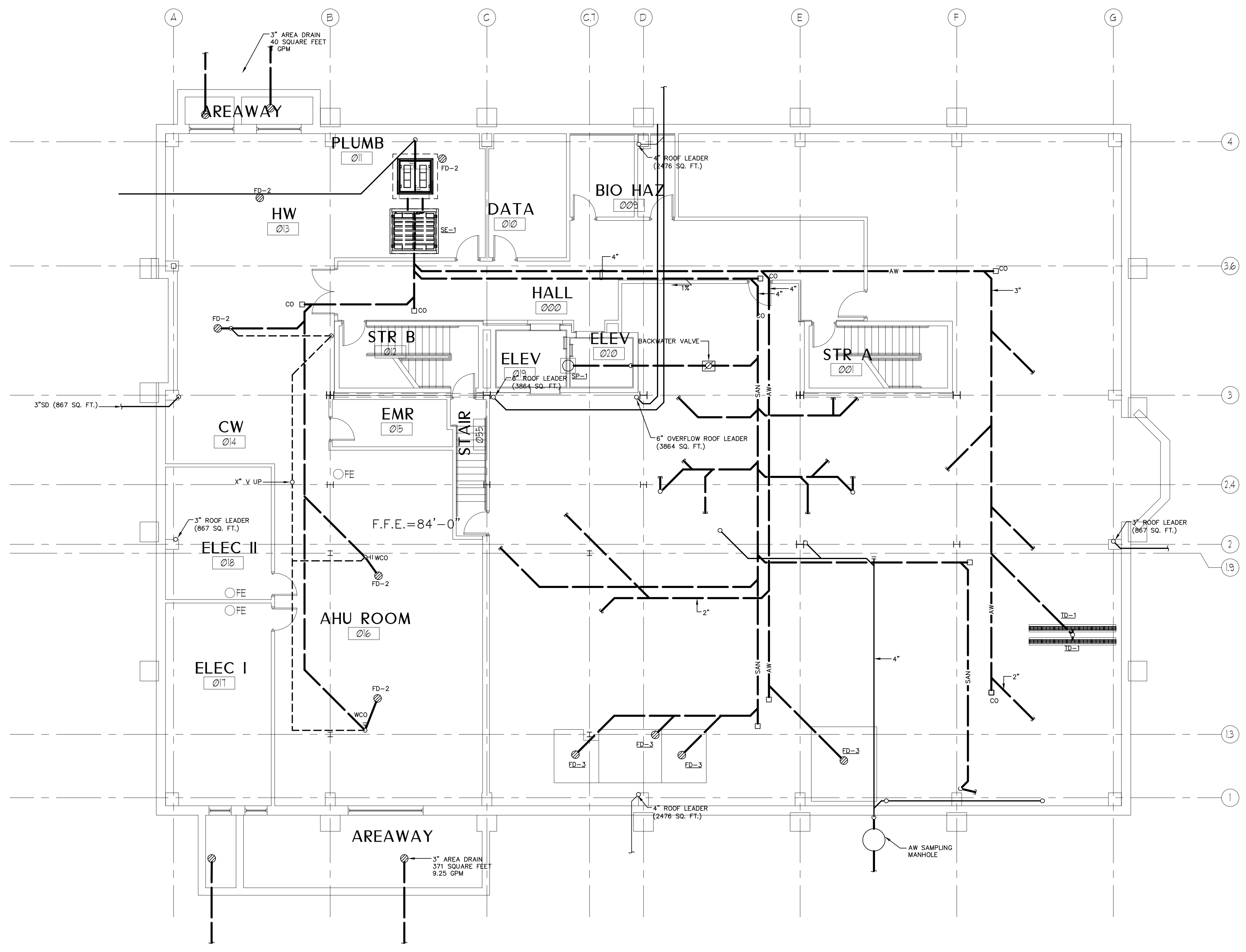
1 PLUMBING LOWER LEVEL PLAN - WASTE Scale: 1/8"=1'-0"
